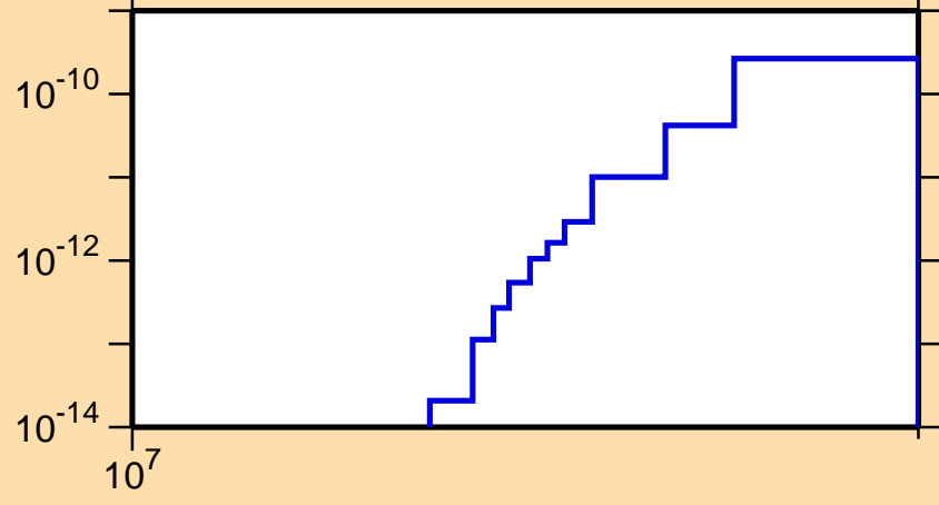
\sigma vs. E for ^{266}\alpha
