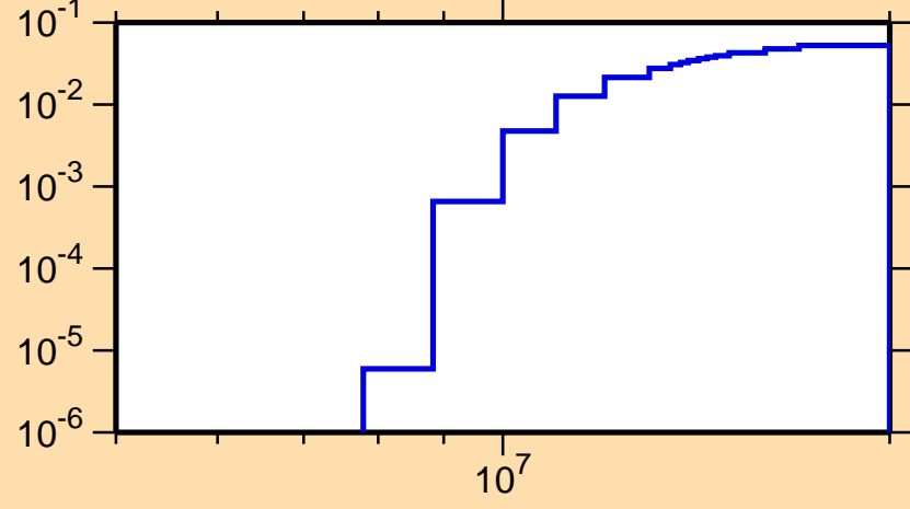
\sigma vs. E for ^{18}\text{F}(n,\text{nd})
