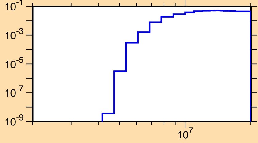
\sigma vs. E for ^{18}\text{F}(n,p\alpha)
