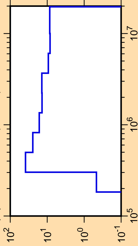
\Delta\mu/\mu vs. E for ^{18}\text{F} (mt251)
