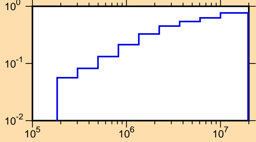
\mu vs. E for ^{18}\text{F} (mt251)
