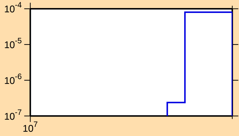
\sigma vs. E for ^{22}\text{F}(n,nt)
