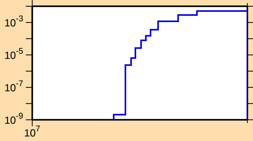
\sigma vs. E for ^{22}\text{F}(n,np)
