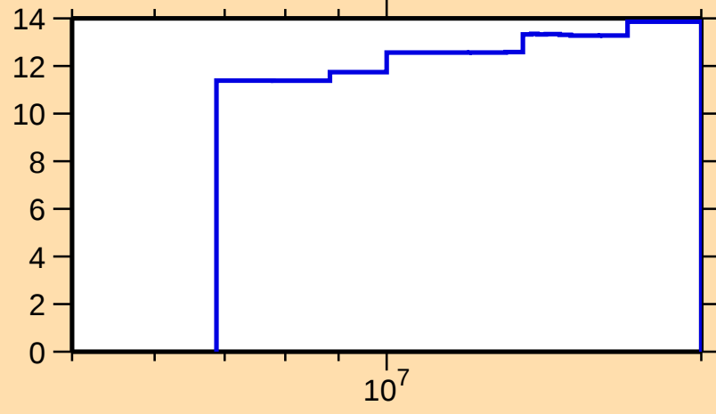
\Delta\sigma/\sigma vs. E for ^{22}\text{F}(\text{n},\text{nonel.})
