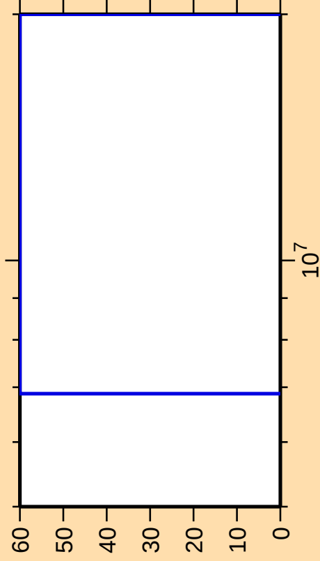
\Delta\sigma/\sigma vs. E for ^{22}\text{F}(\text{n},\text{ncont.})
