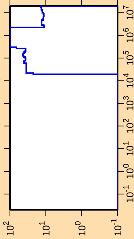
\Delta\sigma/\sigma vs. E for ^{22}\text{F}(n,\text{nonel.})
