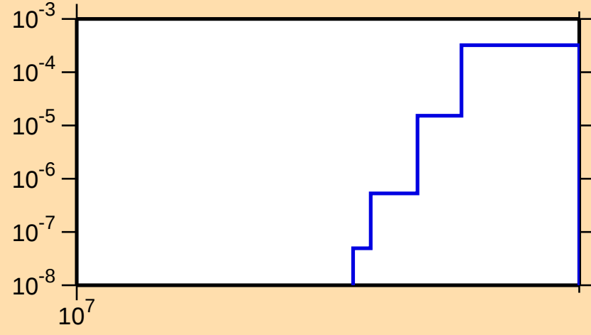
\sigma vs. E for ^{22}\text{F}(n,\text{nd})
