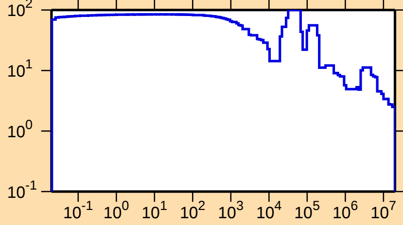
\Delta\sigma/\sigma vs. E for ^{22}\text{F}(n,\text{tot.})
