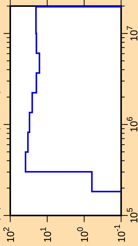
\Delta\mu/\mu vs. E for ^{22}\text{F}(\text{mt251})
