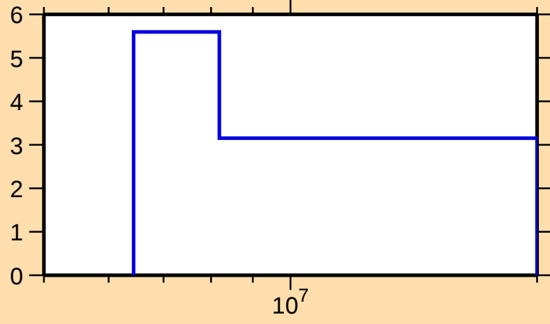
\Delta\sigma/\sigma vs. E for ^{22}\text{F}(\text{n},\text{tot.})
