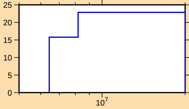
\Delta\sigma/\sigma vs. E for ^{22}\text{F}(\text{n},\text{inel.})
