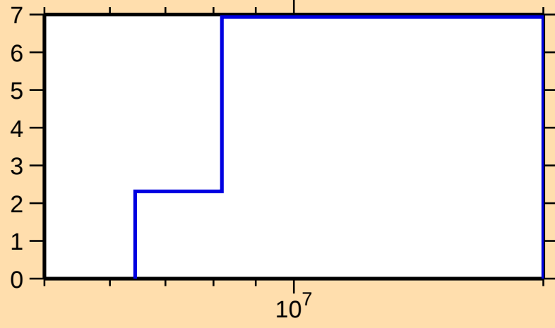
\Delta\sigma/\sigma vs. E for ^{22}\text{F}(\text{n},\text{el.})
