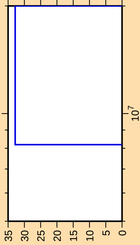
\Delta\sigma/\sigma vs. E for ^{22}\text{F}(\text{n},\text{nd})
