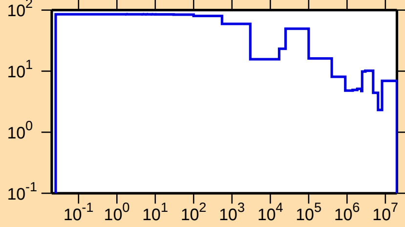
\Delta\sigma/\sigma vs. E for ^{22}\text{F}(n,\text{el.})
