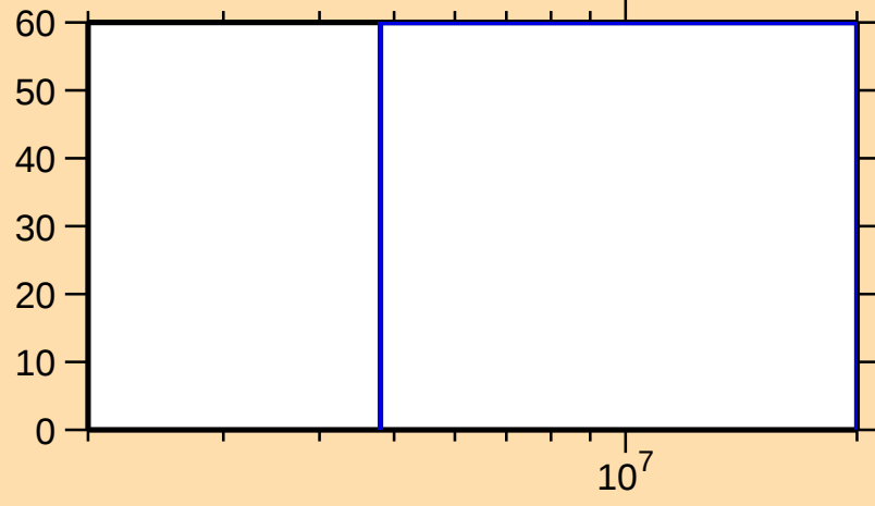
\Delta\sigma/\sigma vs. E for ^{22}\text{F}(n,\gamma)
