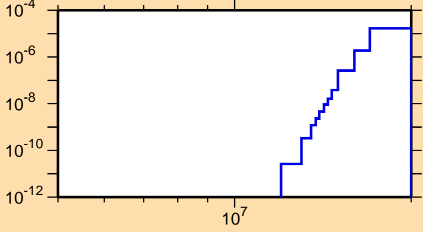
\sigma vs. E for ^{209}\text{Fr}(n,\text{nd})
