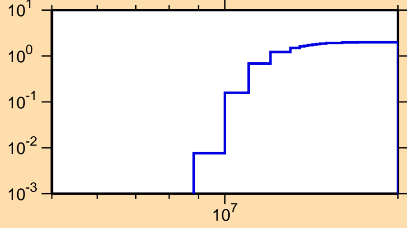
\sigma vs. E for ^{209}\text{Fr}(n,2n)
