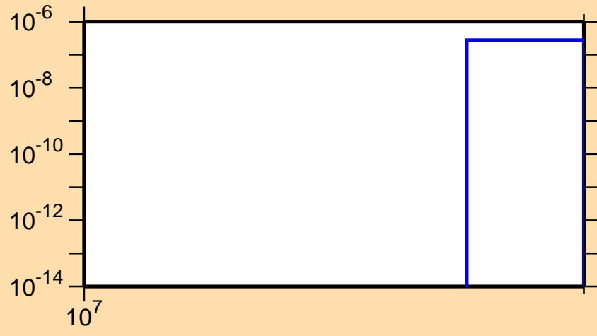
\sigma vs. E for ^{209}\text{Fr}(n,3n\alpha)
