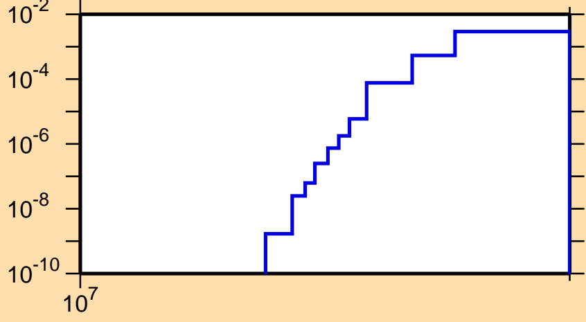
\sigma vs. E for ^{209}\text{Fr}(n,2np)
