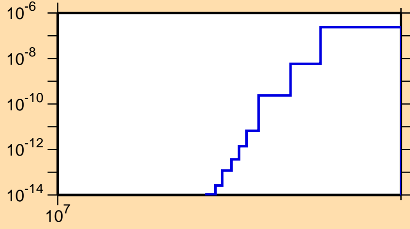
\sigma vs. E for ^{209}\text{Fr}(n,nt)
