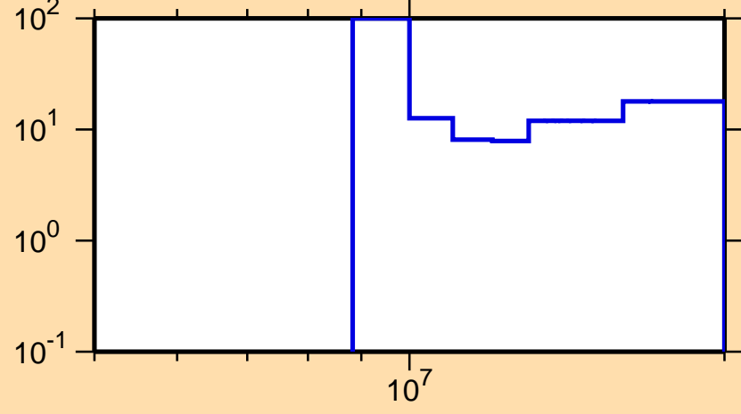
\Delta\sigma/\sigma vs. E for ^{209}\text{Fr}(n,2n)
