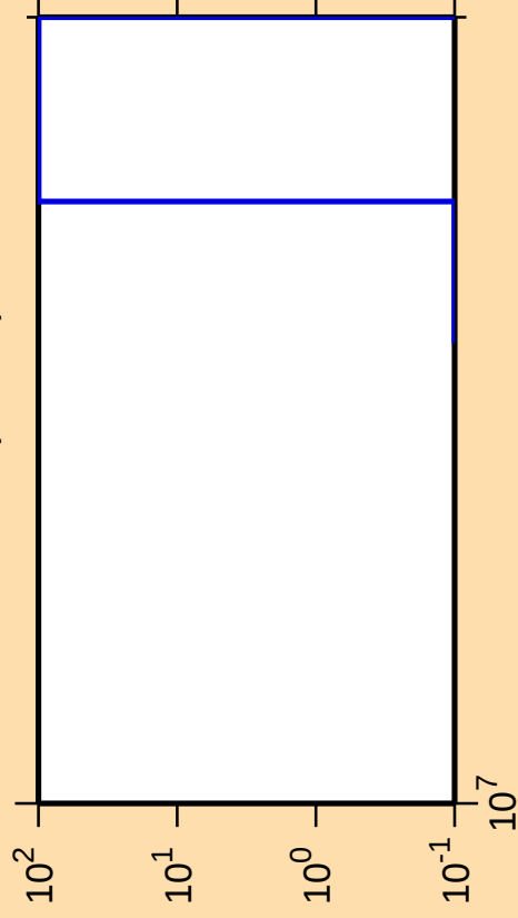
\Delta\sigma/\sigma vs. E for ^{65}\text{Ga} (mt 34)
