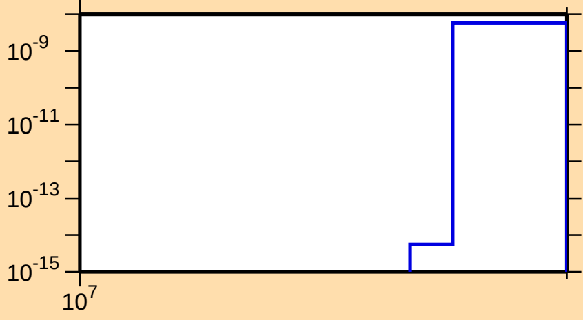
\sigma vs. E for ^{65}\text{Ga}(n,\text{nt})
