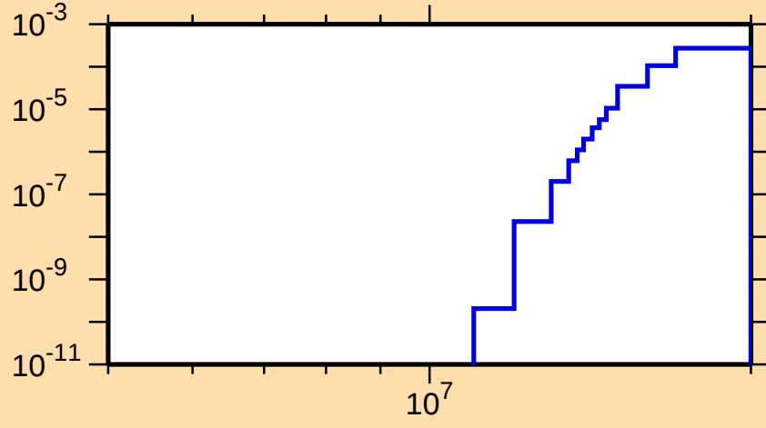
\sigma vs. E for ^{65}\text{Ga}(\text{mt117})
