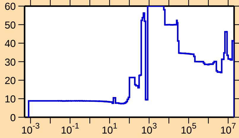
\Delta\sigma/\sigma vs. E for ^{65}\text{Ga}(n,\gamma)
