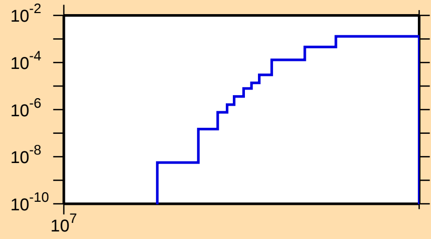
\sigma vs. E for ^{65}\text{Ga}(n,\text{pd})
