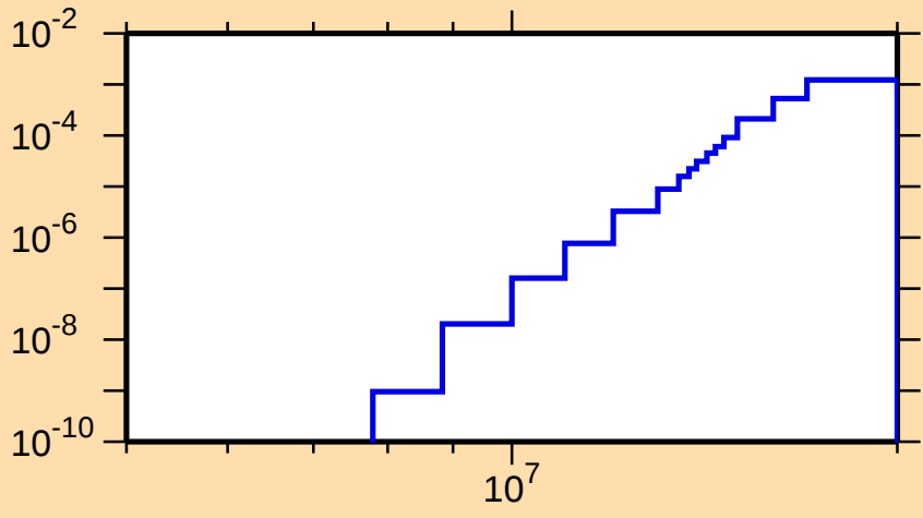
\sigma vs. E for ^{65}\text{Ga}(n,\text{He}3)
