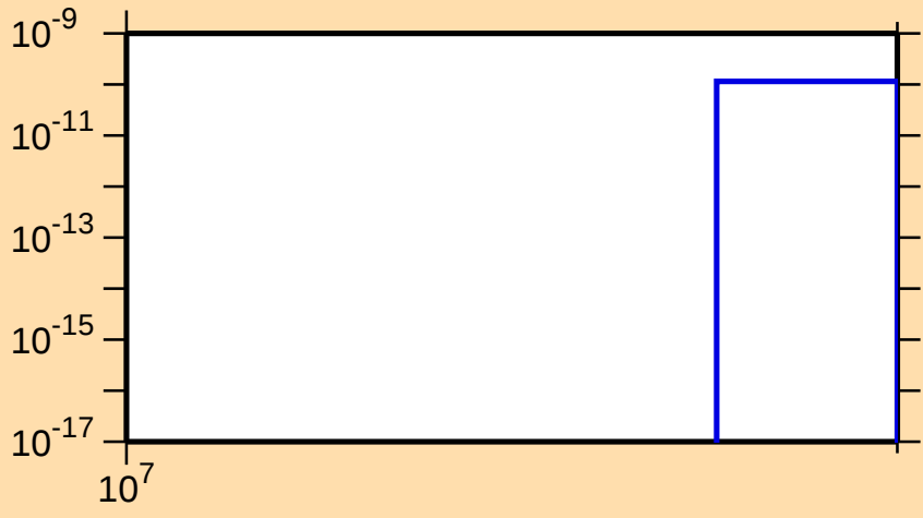
\sigma vs. E for ^{65}\text{Ga} (mt 34)
