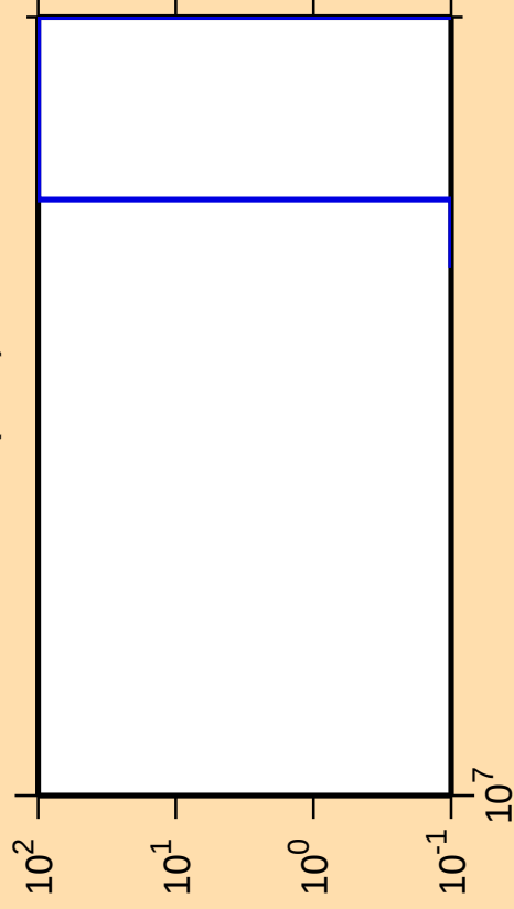
\Delta\sigma/\sigma vs. E for ^{65}\text{Ga}(n,\text{nt})
