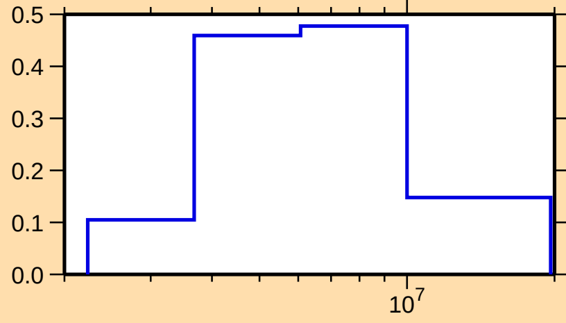
\sigma vs. E for ^{65}\text{Ga}(n,n\text{cont.})
