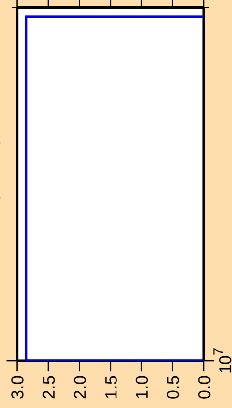
\Delta\sigma/\sigma vs. E for ^{65}\text{Ga}(\text{mt } 34)
