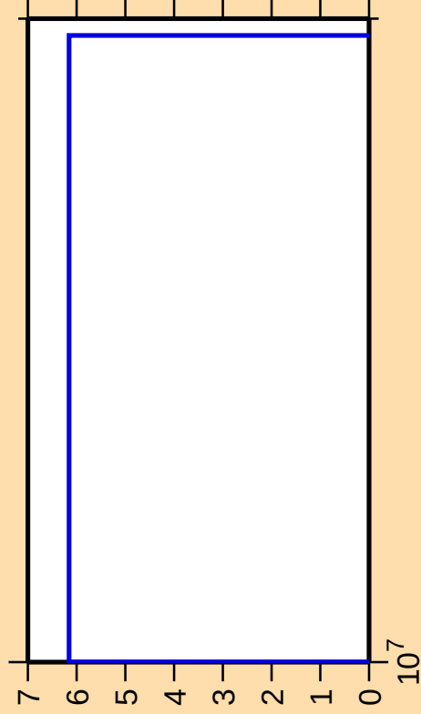
\Delta\sigma/\sigma vs. E for ^{65}\text{Ga}(n,p)
