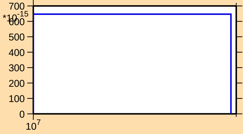
\sigma vs. E for ^{65}\text{Ga}(\text{mt } 34)
