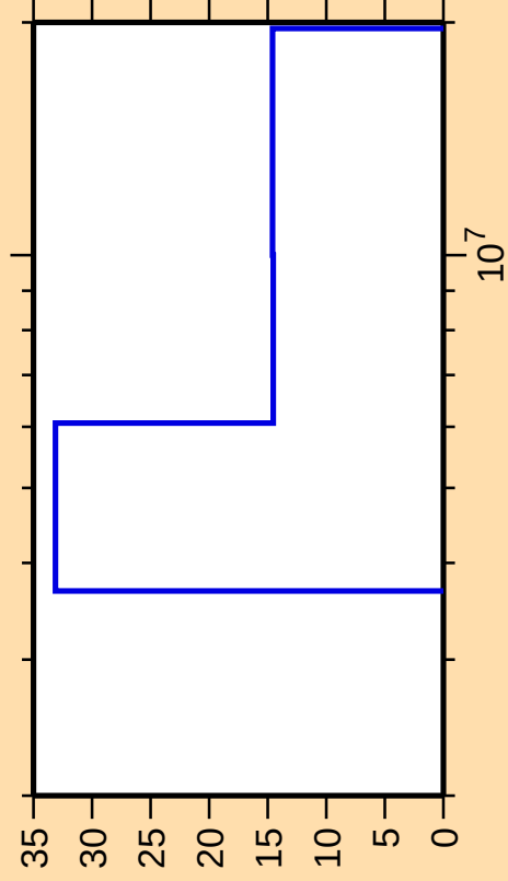
\Delta\sigma/\sigma vs. E for ^{65}\text{Ga}(n,np)
