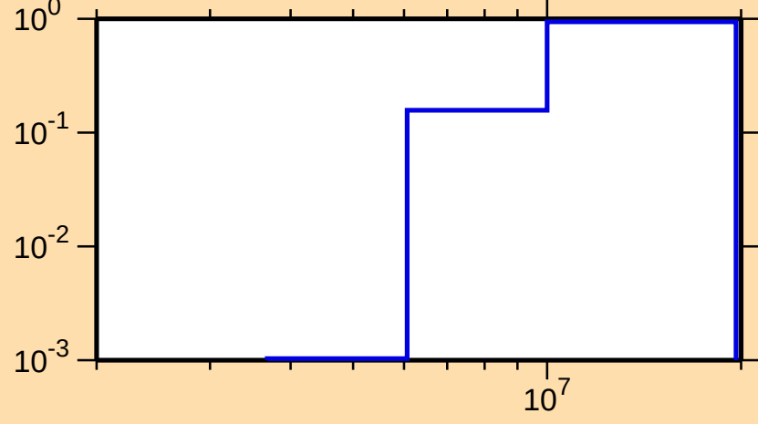
\sigma vs. E for ^{65}\text{Ga}(n,np)
