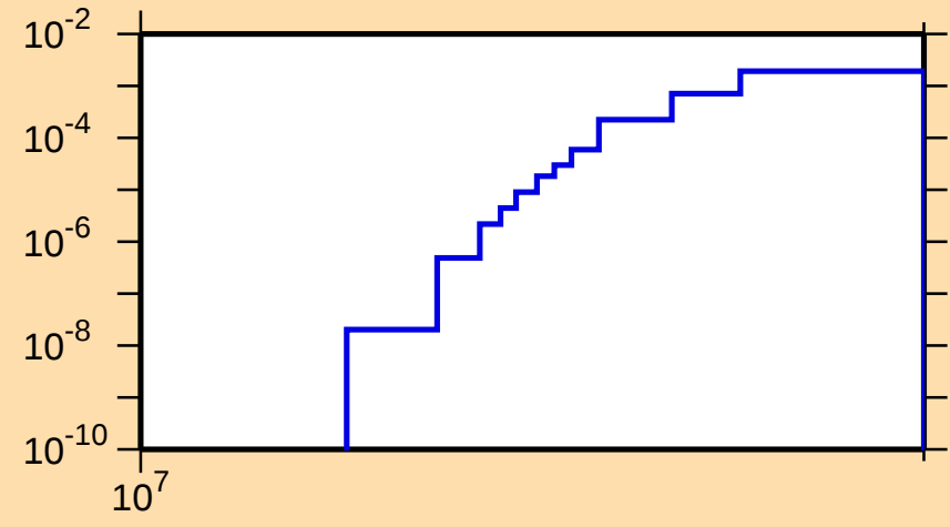
\sigma vs. E for ^{66}\text{Ga}(n,\text{nd})
