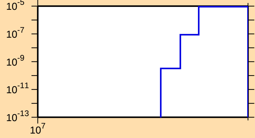
\sigma vs. E for ^{66}\text{Ga}(n,\text{pt})
