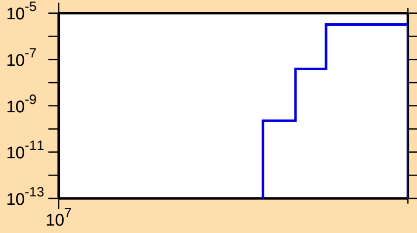
\sigma vs. E for ^{66}\text{Ga}(n,2n\alpha)
