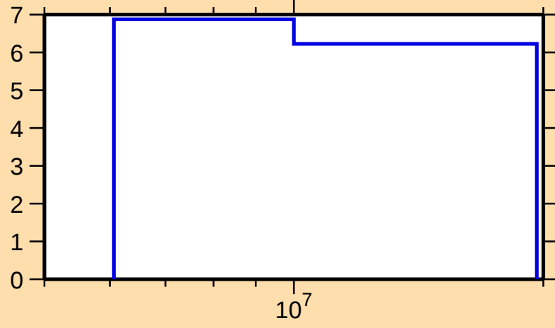
\Delta\sigma/\sigma vs. E for ^{66}\text{Ga}(n,\text{nonel.})
