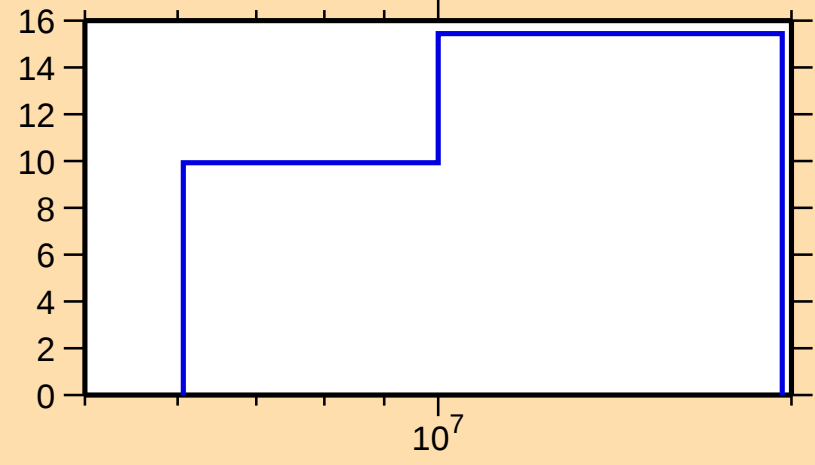
\Delta\sigma/\sigma vs. E for ^{66}\text{Ga}(n,\text{el.})
