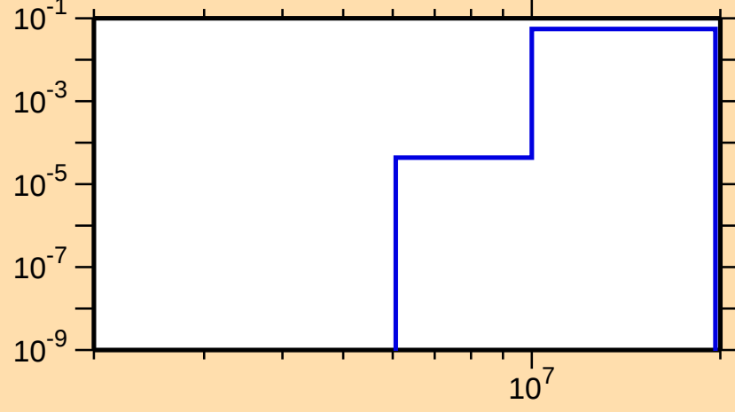
\sigma vs. E for ^{66}\text{Ga}(n,n\alpha)
