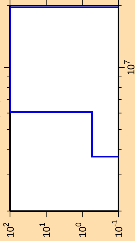
\Delta\sigma/\sigma vs. E for ^{66}\text{Ga}(n,t)
