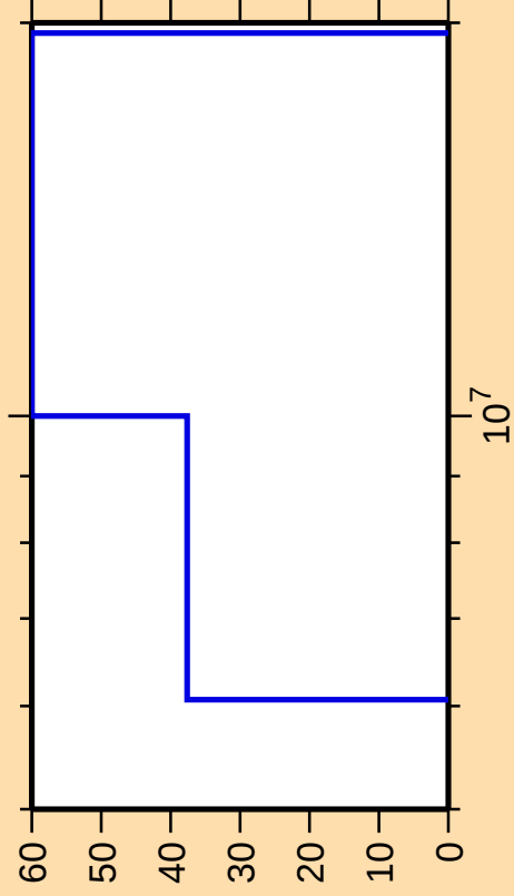
\Delta\sigma/\sigma vs. E for ^{66}\text{Ga}(n,n\text{cont.})
