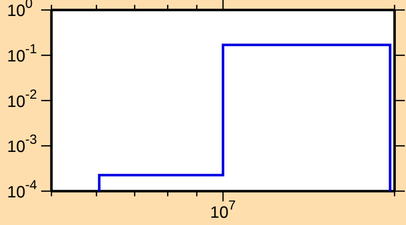
\sigma vs. E for ^{66}\text{Ga}(n,2n)
