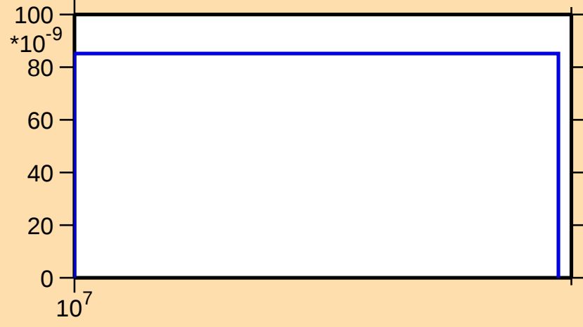
\sigma vs. E for ^{66}\text{Ga}(n,\text{pt})
