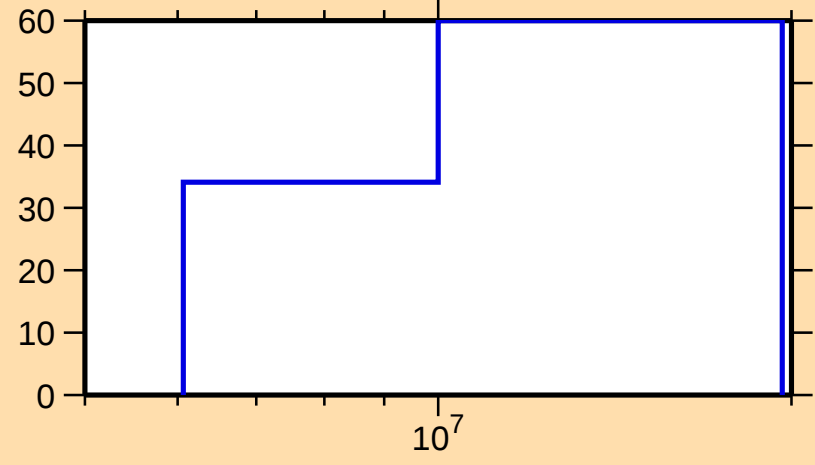
\Delta\sigma/\sigma vs. E for ^{66}\text{Ga}(n,\text{inel.})
