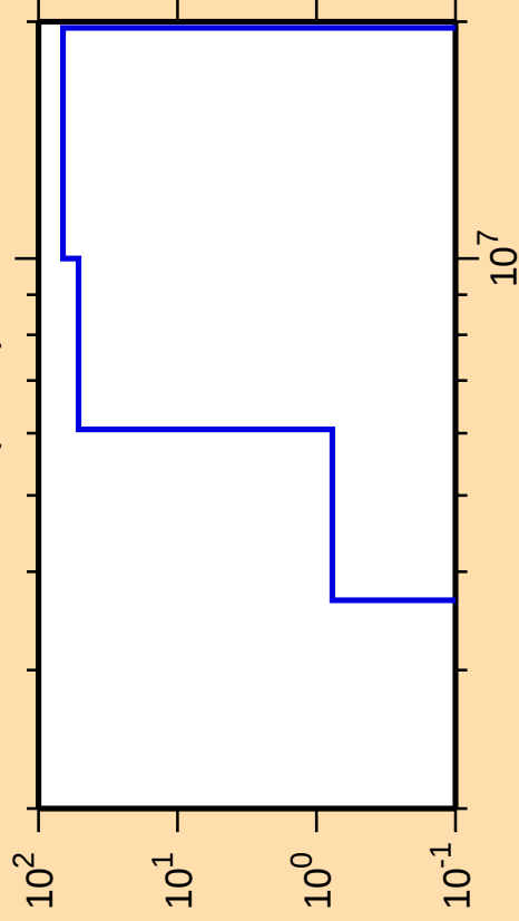
\Delta\sigma/\sigma vs. E for ^{66}\text{Ga}(n,n\alpha)
