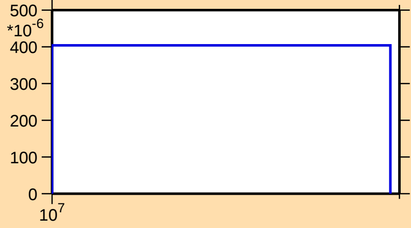
\sigma vs. E for ^{66}\text{Ga}(n,2np)
