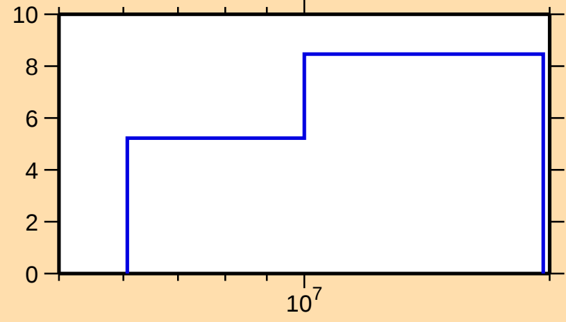
\Delta\sigma/\sigma vs. E for ^{66}\text{Ga}(n,\text{tot.})
