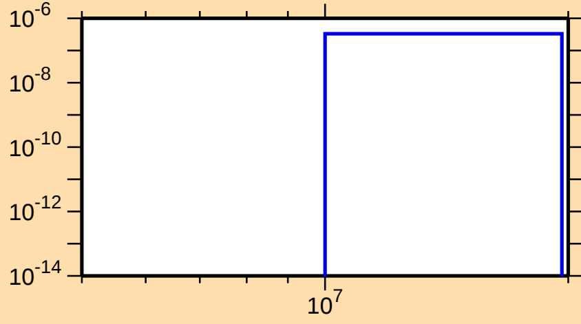
\sigma vs. E for ^{66}\text{Ga}(\text{mt117})
