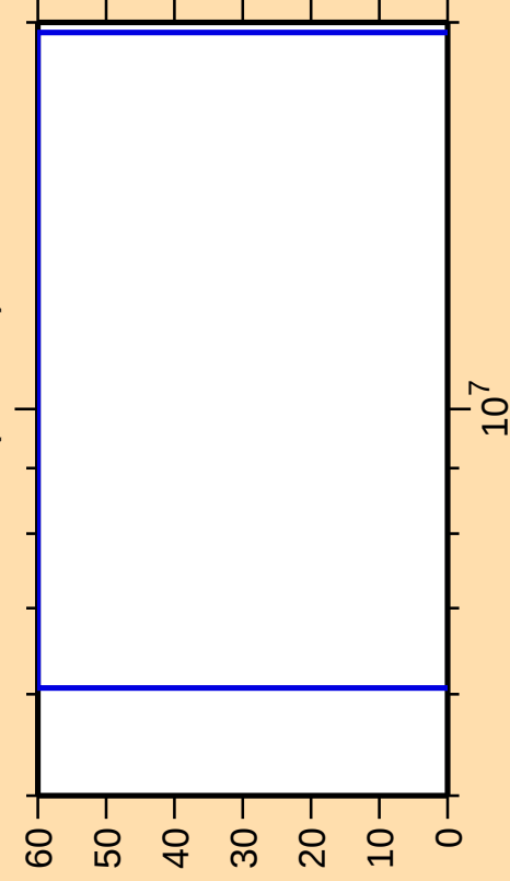
\Delta\sigma/\sigma vs. E for ^{66}\text{Ga}(n,\text{He}3)
