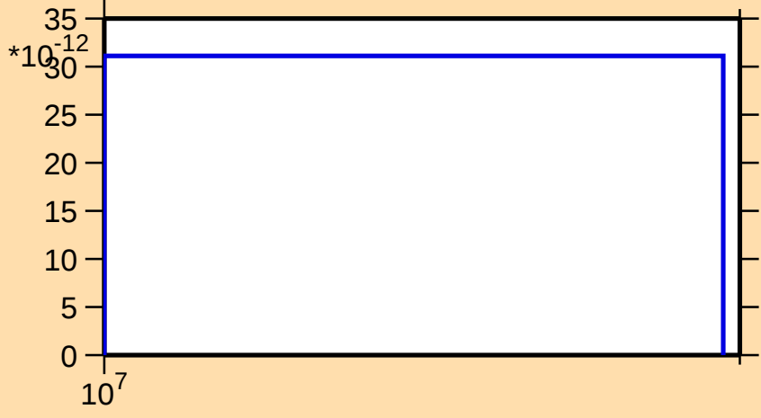
\sigma vs. E for ^{66}\text{Ga}(n,\text{nt})
