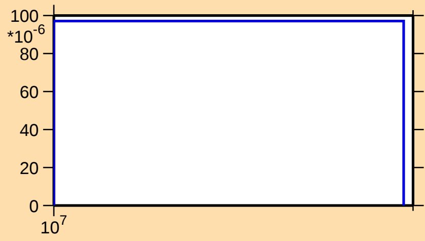
\sigma vs. E for ^{66}\text{Ga}(n,\text{nd})
