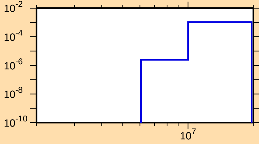
\sigma vs. E for ^{66}\text{Ga}(n,t)
