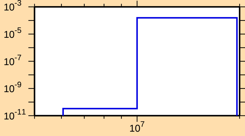
\sigma vs. E for ^{66}\text{Ga}(n,\text{He}3)
