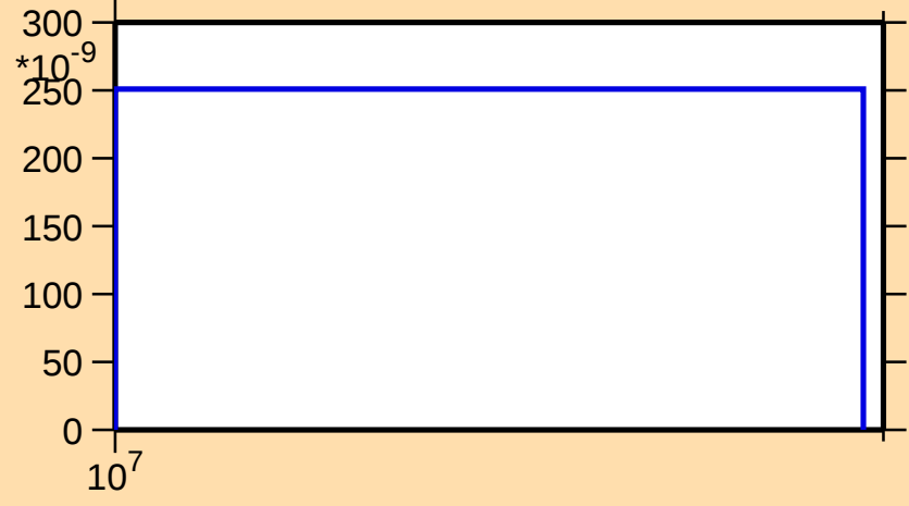
\sigma vs. E for ^{66}\text{Ga}(n,\text{pd})
