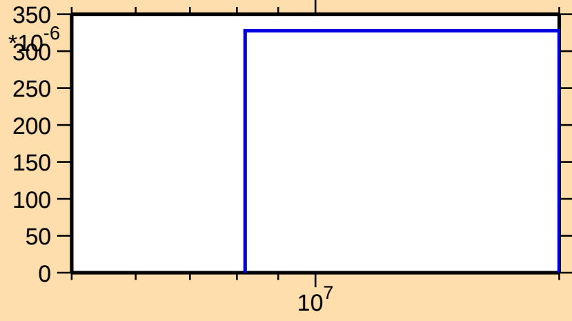
\sigma vs. E for ^{66}\text{Ga}(n,2np)
