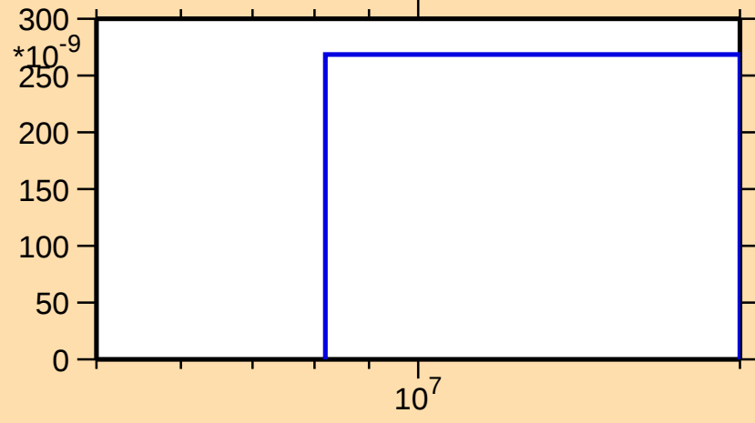
\sigma vs. E for ^{66}\text{Ga}(\text{mt117})
