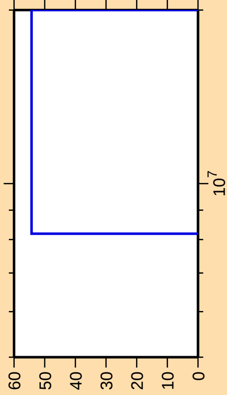
\Delta\sigma/\sigma vs. E for ^{66}\text{Ga}(n,n_1)
