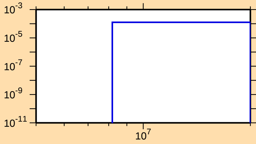
\sigma vs. E for ^{66}\text{Ga}(n,\text{He}3)
