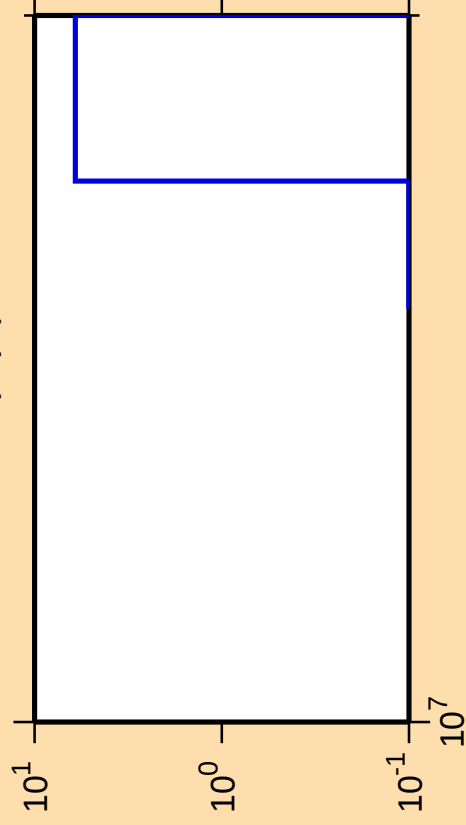
\Delta\sigma/\sigma vs. E for ^{67}\text{Ga}(n,\text{pt})
