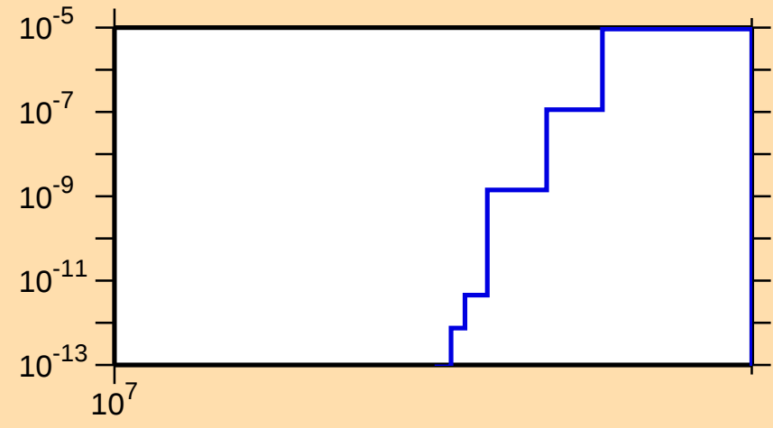
\sigma vs. E for ^{67}\text{Ga}(\text{mt 45})
