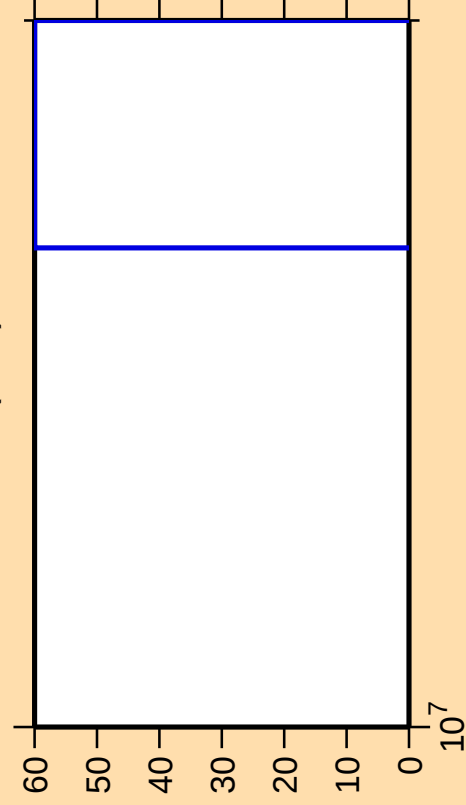
\Delta\sigma/\sigma vs. E for ^{67}\text{Ga}(n,\text{nt})
