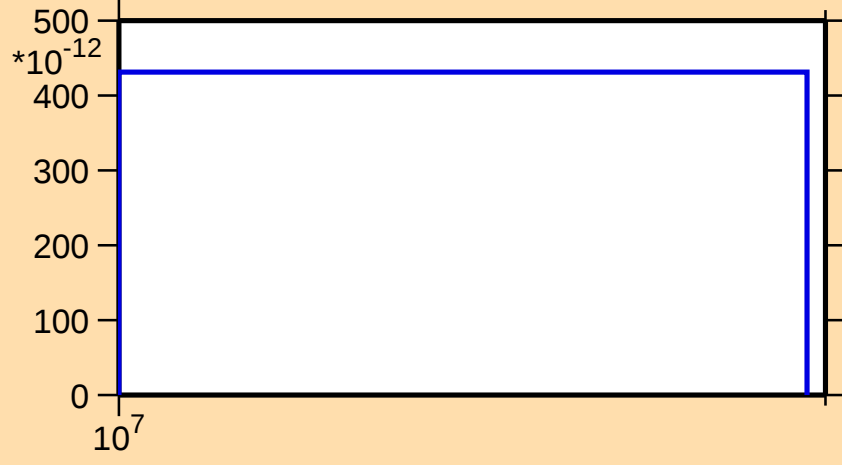
\sigma vs. E for ^{67}\text{Ga}(n,\text{nt})
