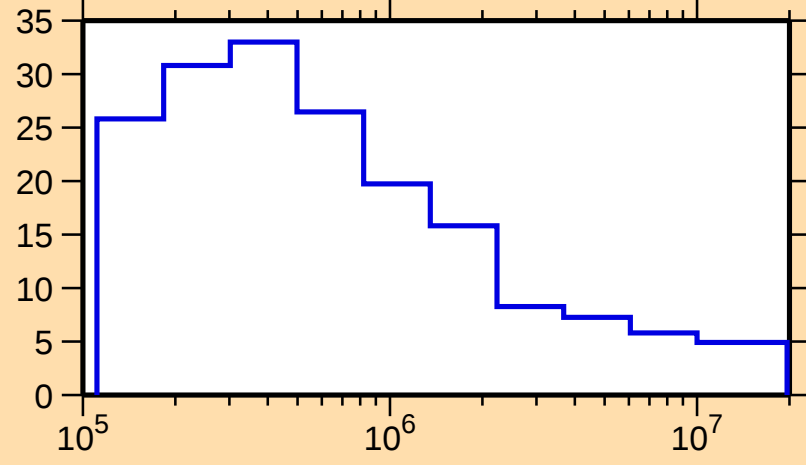
\Delta\sigma/\sigma vs. E for ^{67}\text{Ga}(\text{n,nonel.})
