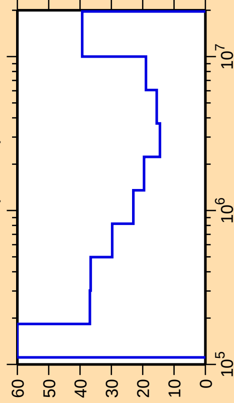
\Delta\sigma/\sigma vs. E for ^{67}\text{Ga}(\text{n,inel.})
