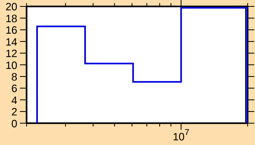
\Delta\sigma/\sigma vs. E for ^{67}\text{Ga}(\text{n},\text{el.})
