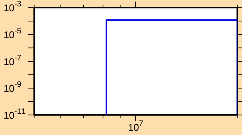
\sigma vs. E for ^{67}\text{Ga}(n,t)
