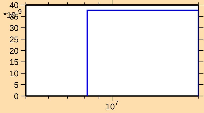
\sigma vs. E for ^{67}\text{Ga}(n,\text{pd})
