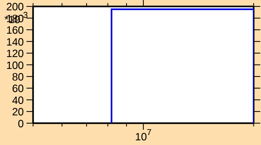
\sigma vs. E for ^{67}\text{Ga}(n,2n)
