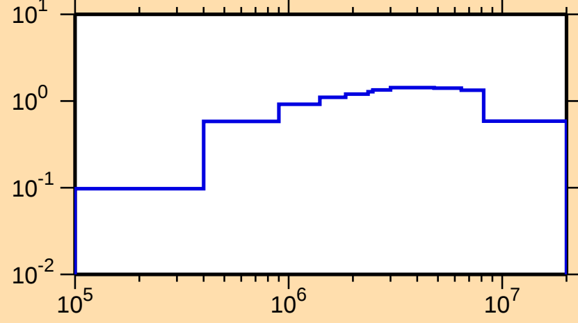
\sigma vs. E for ^{67}\text{Ga}(n,\text{inel.})
