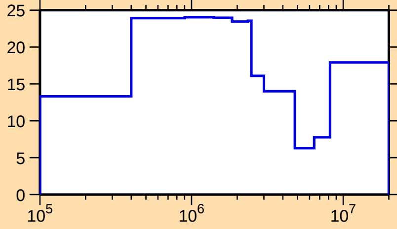
\Delta\sigma/\sigma vs. E for ^{67}\text{Ga}(\text{n,el.})
