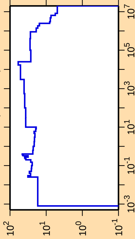
\Delta\sigma/\sigma vs. E for ^{67}\text{Ga}(n,\text{nonel.})
