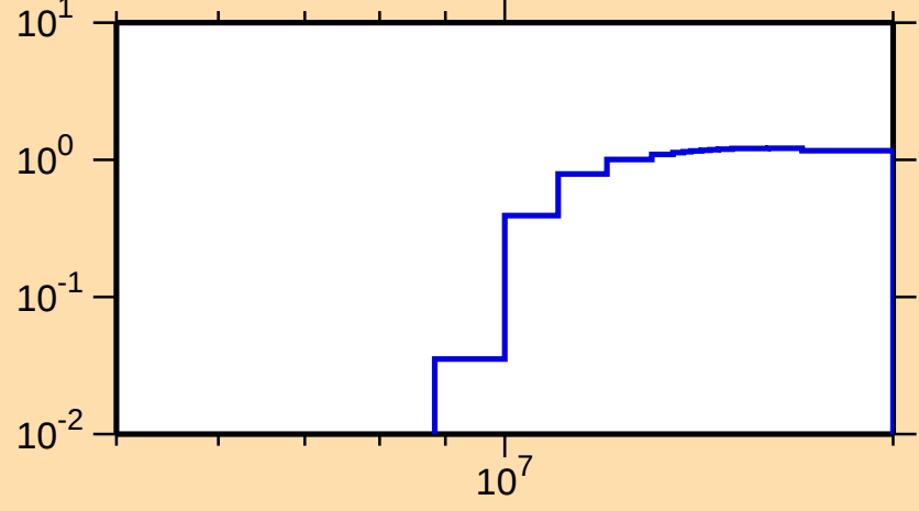
\sigma vs. E for ^{73}\text{Ga}(n,2n)
