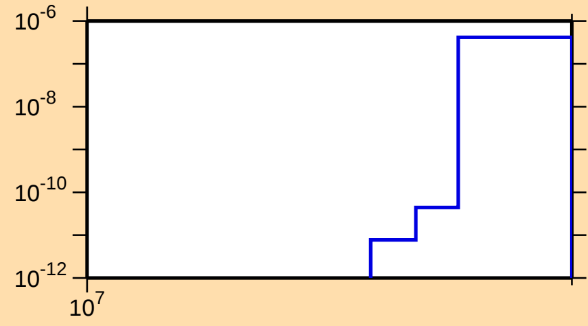
\sigma vs. E for ^{73}\text{Ga}(n,\text{nt})
