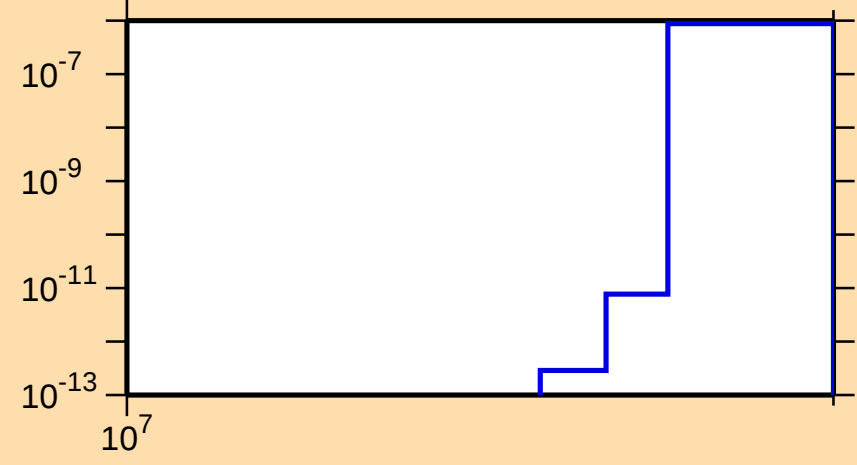
\sigma vs. E for ^{73}\text{Ga}(n,\text{nd})
