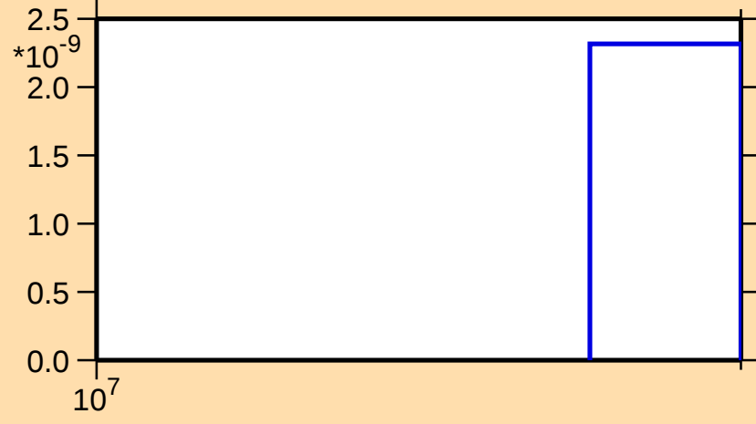
\sigma vs. E for ^{73}\text{Ga}(n,2np)
