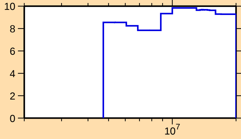
\Delta\sigma/\sigma vs. E for ^{75}\text{Ga}(n,\text{nonel.})
