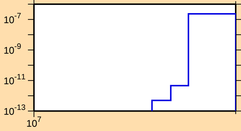
\sigma vs. E for ^{75}\text{Ga}(n,\text{nt})
