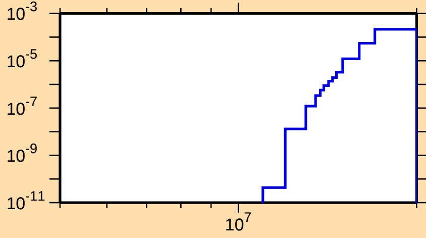
\sigma vs. E for ^{75}\text{Ga}(n,t)
