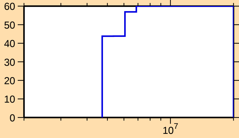
\Delta\sigma/\sigma vs. E for ^{75}\text{Ga}(n,\gamma)
