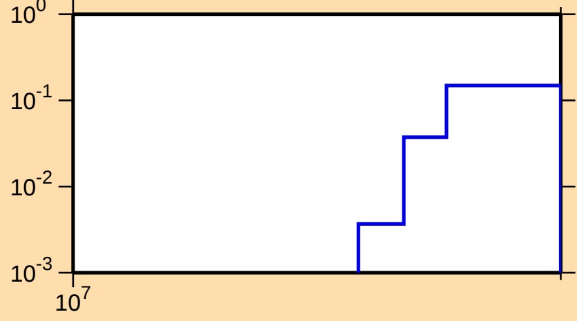
\sigma vs. E for ^{75}\text{Ga}(n,3n)
