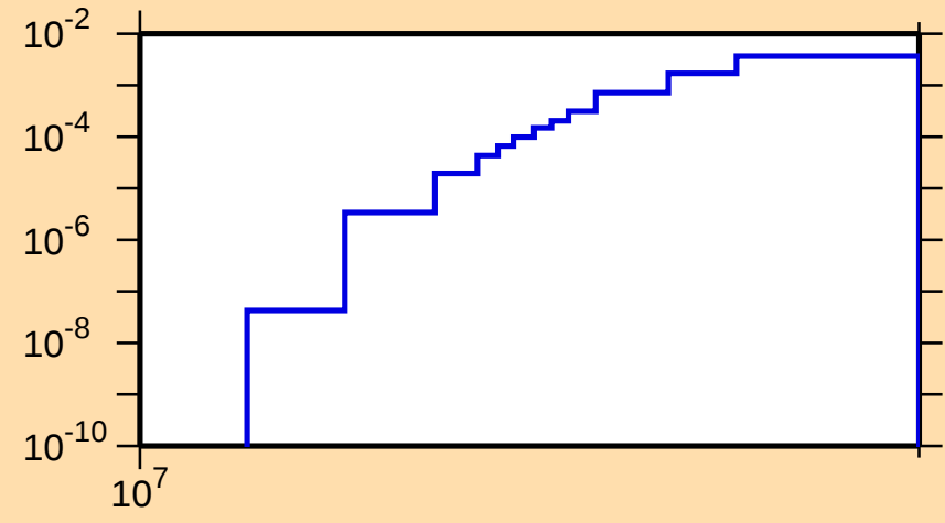
\sigma vs. E for ^{75}\text{Ga}(n,np)
