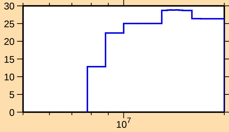
\Delta\sigma/\sigma vs. E for ^{75}\text{Ga}(n,\text{el.})
