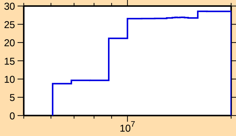
\Delta\sigma/\sigma vs. E for ^{75}\text{Ga}(n,\text{inel.})
