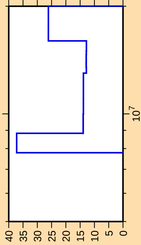
\Delta\sigma/\sigma vs. E for ^{75}\text{Ga}(n,2n)
