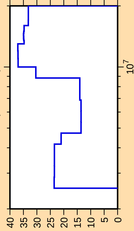
\Delta\sigma/\sigma vs. E for ^{75}\text{Ga}(n,n\text{cont.})
