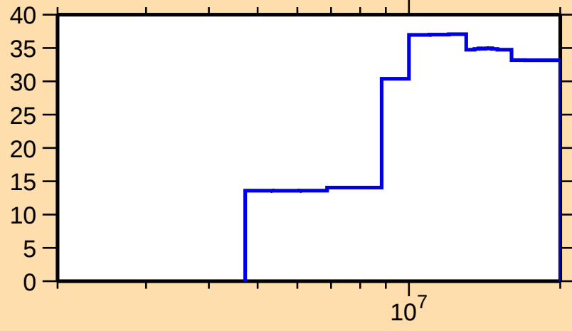
\Delta\sigma/\sigma vs. E for ^{75}\text{Ga}(n,n\text{cont.})
