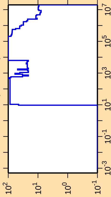
\Delta\sigma/\sigma vs. E for ^{75}\text{Ga}(n,\text{nonel.})
