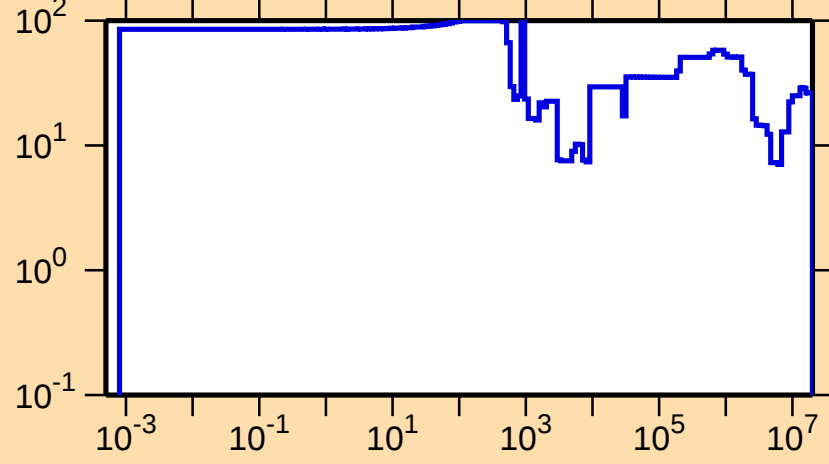
\Delta\sigma/\sigma vs. E for ^{75}\text{Ga}(n,\text{el.})
