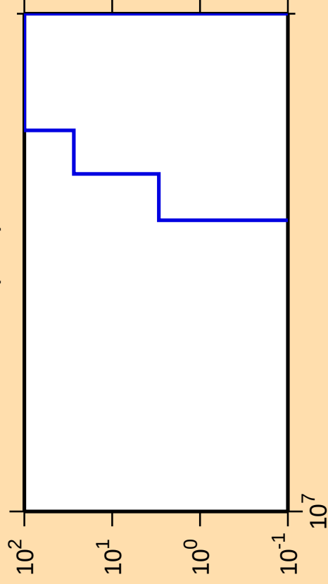
\Delta\sigma/\sigma vs. E for ^{75}\text{Ga}(n,\text{nt})
