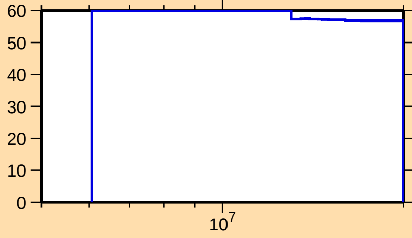
\Delta\sigma/\sigma vs. E for ^{75}\text{Ga}(n,p)
