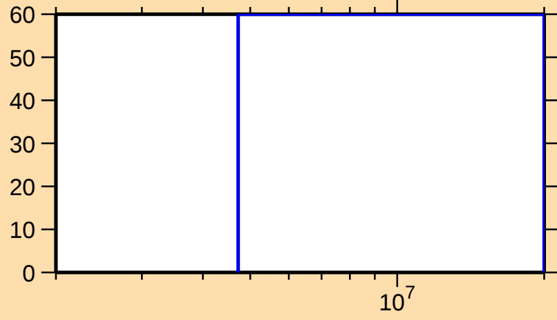
\Delta\sigma/\sigma vs. E for ^{75}\text{Ga}(n,n_1)
