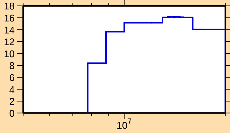
\Delta\sigma/\sigma vs. E for ^{75}\text{Ga}(n,\text{tot.})
