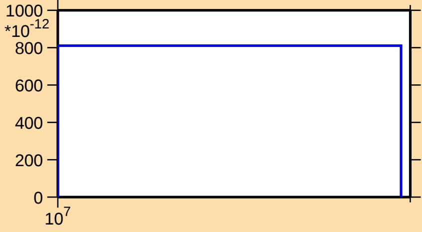
\sigma vs. E for ^{75}\text{Ga}(n,\text{nd})
