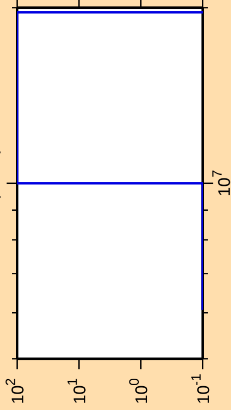
\Delta\sigma/\sigma vs. E for ^{75}\text{Ga}(n,n\alpha)
