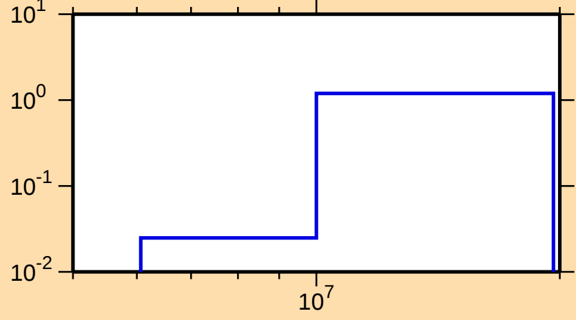
\sigma vs. E for ^{75}\text{Ga}(n,2n)
