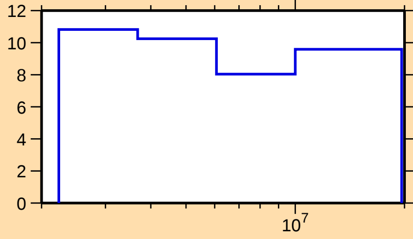
\Delta\sigma/\sigma vs. E for ^{75}\text{Ga}(n,n\text{onrel.})
