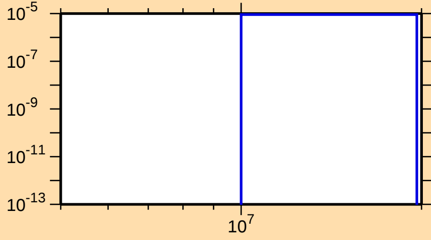
\sigma vs. E for ^{75}\text{Ga}(n,n\alpha)
