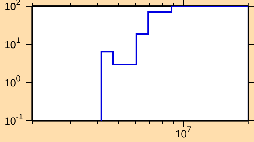
\Delta\sigma/\sigma vs. E for ^{76}\text{Ga}(n,n\text{cont.})
