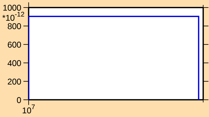
\sigma vs. E for ^{76}\text{Ga}(n,\text{nt})
