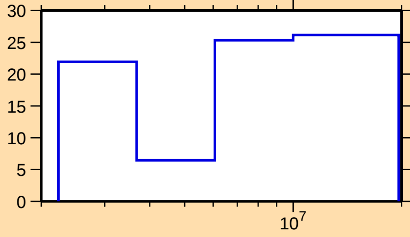
\Delta\sigma/\sigma vs. E for ^{76}\text{Ga}(\text{n},\text{el.})
