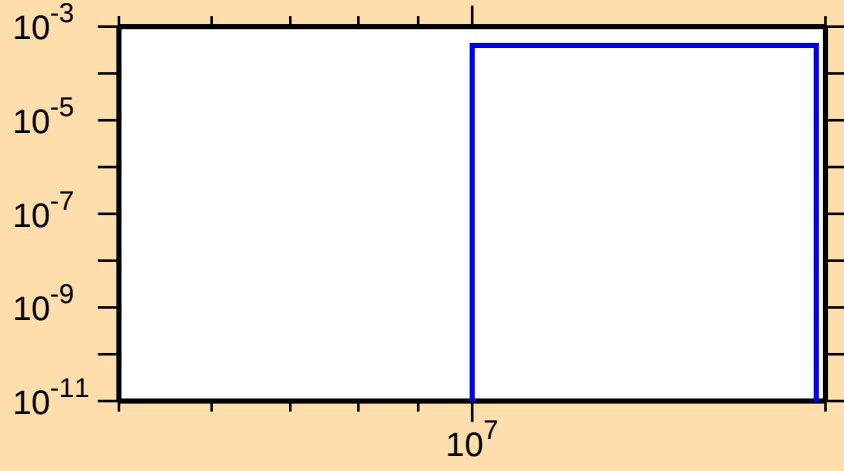
\sigma vs. E for ^{76}\text{Ga}(n,d)
