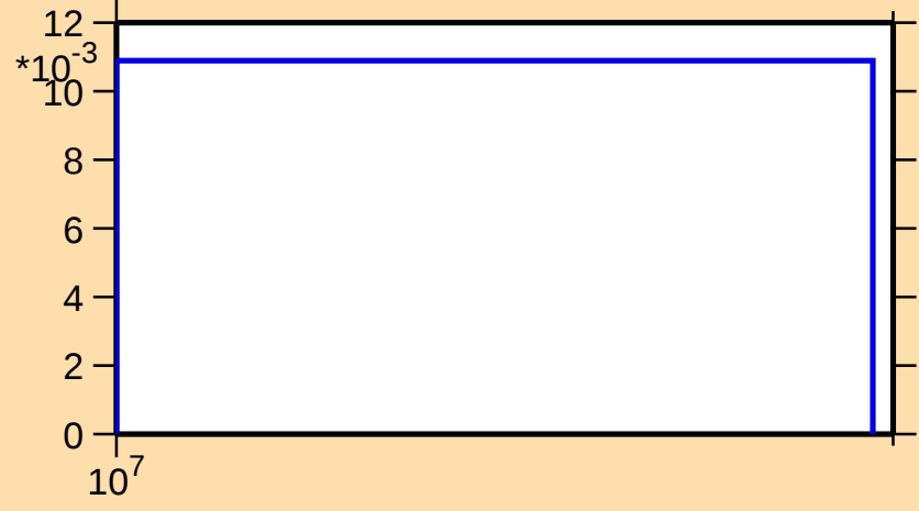
\sigma vs. E for ^{76}\text{Ga}(n,3n)
