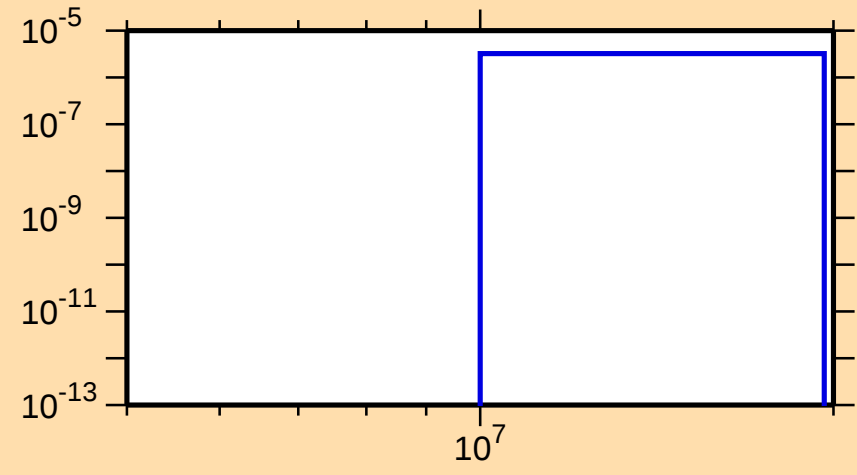
\sigma vs. E for ^{76}\text{Ga}(n,n\alpha)
