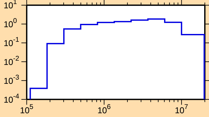
\sigma vs. E for ^{76}\text{Ga}(n,\text{inel.})
