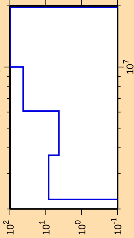
\Delta\sigma/\sigma vs. E for ^{76}\text{Ga}(\text{n},\text{ncont.})
