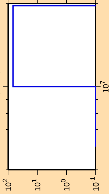
\Delta\sigma/\sigma vs. E for ^{76}\text{Ga}(n,n\alpha)
