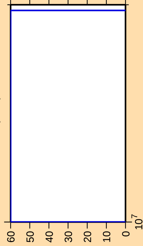
\Delta\sigma/\sigma vs. E for ^{76}\text{Ga}(n,\text{nt})
