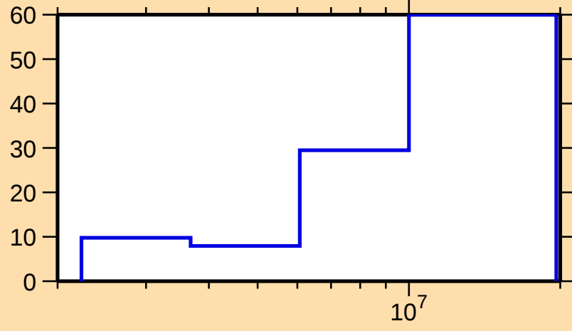
\Delta\sigma/\sigma vs. E for ^{76}\text{Ga}(\text{n},\text{inel.})
