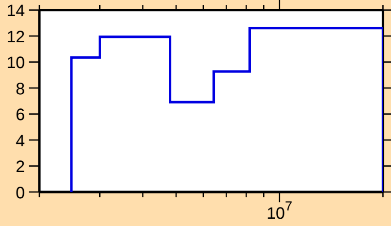
\Delta\sigma/\sigma vs. E for ^{76}\text{Ga}(n,\text{nonel.})
