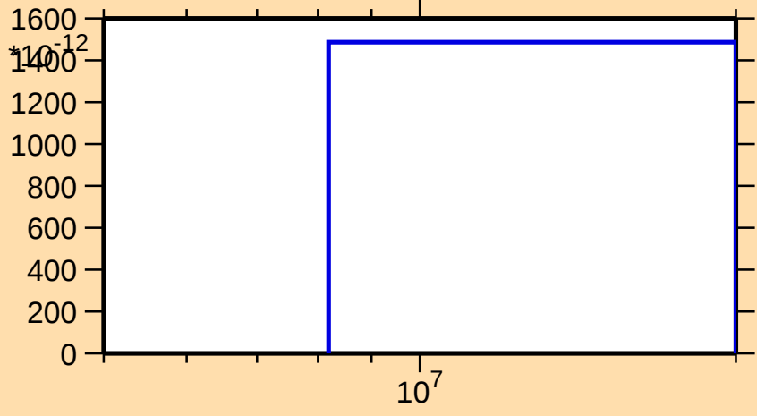
\sigma vs. E for ^{76}\text{Ga}(n,2np)
