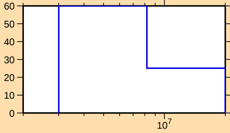
\Delta\sigma/\sigma vs. E for ^{76}\text{Ga}(n,p)
