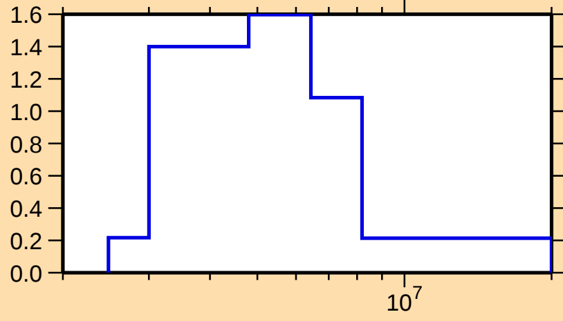
\sigma vs. E for ^{76}\text{Ga}(n,n\text{cont.})
