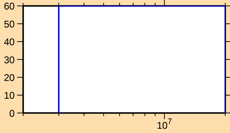
\Delta\sigma/\sigma vs. E for ^{76}\text{Ga}(n,\gamma)
