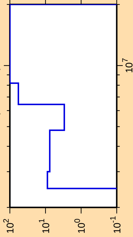
\Delta\sigma/\sigma vs. E for ^{76}\text{Ga}(n,\text{ncont.})
