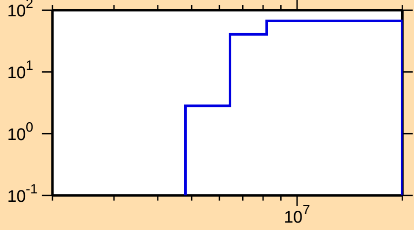
\Delta\sigma/\sigma vs. E for ^{76}\text{Ga}(n,\text{inel.})
