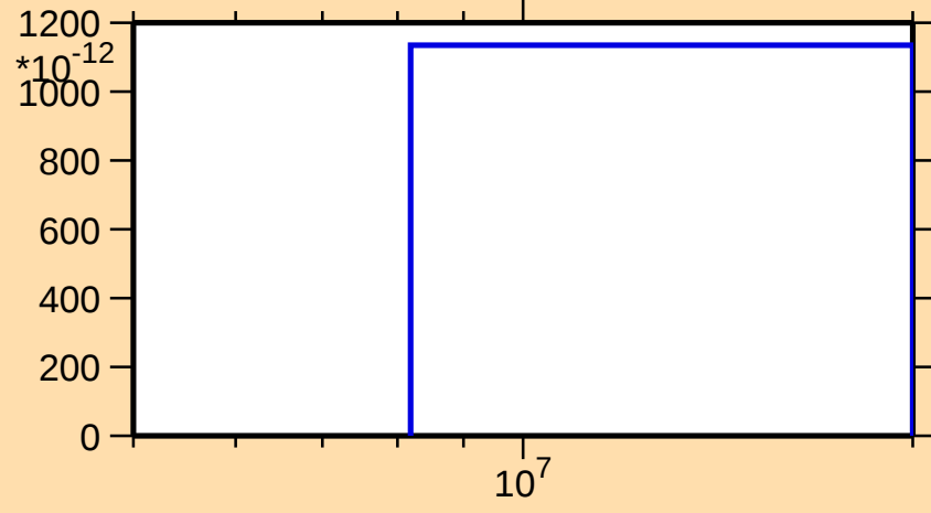
\sigma vs. E for ^{76}\text{Ga}(n,nt)
