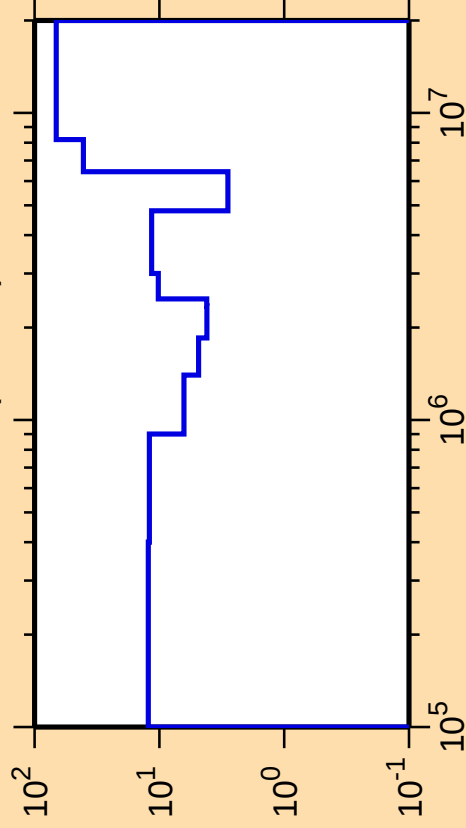
\Delta\sigma/\sigma vs. E for ^{76}\text{Ga}(n,\text{inel.})
