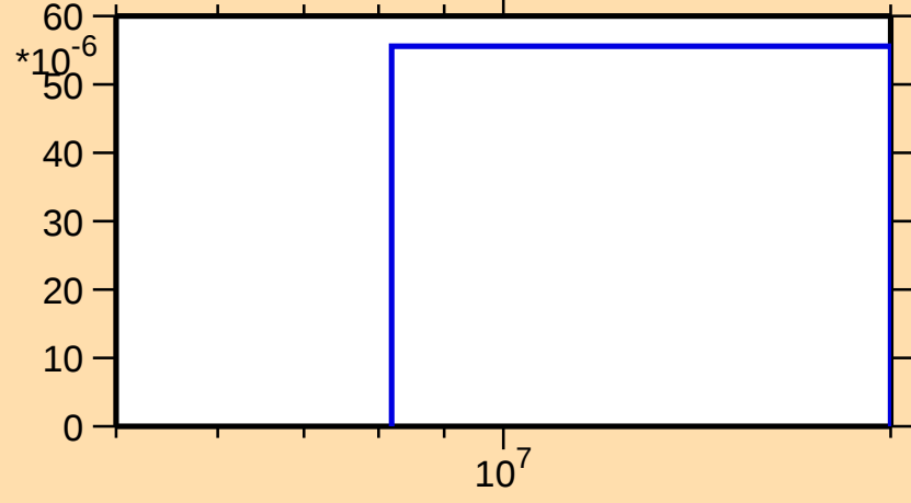
\sigma vs. E for ^{76}\text{Ga}(n,t)
