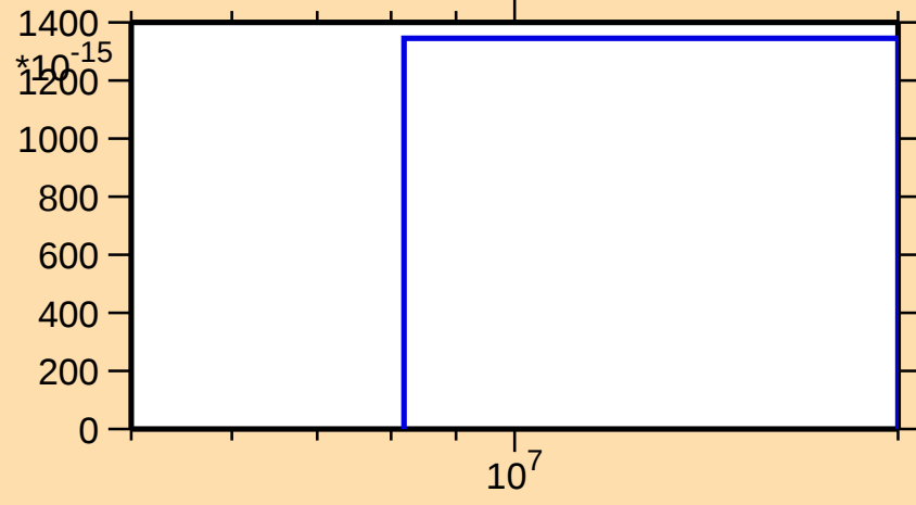
\sigma vs. E for ^{76}\text{Ga}(n,2n\alpha)
