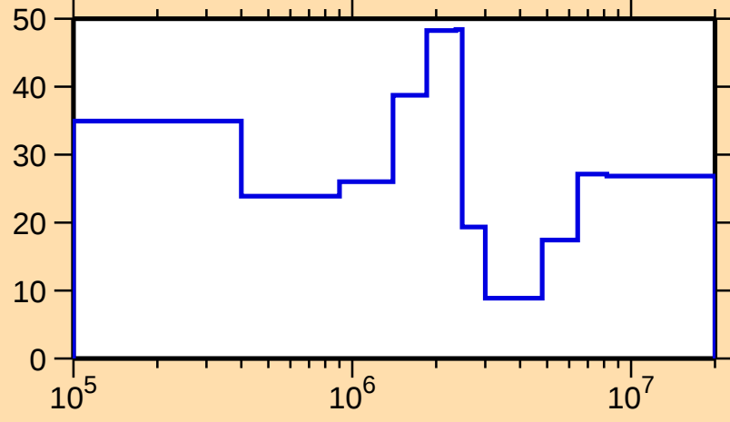
\Delta\sigma/\sigma vs. E for ^{76}\text{Ga}(n,\text{el.})
