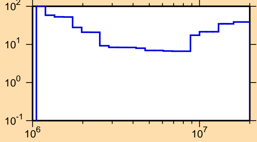
\Delta\sigma/\sigma vs. E for ^{73}\text{Ge}(n,n\text{cont.})
