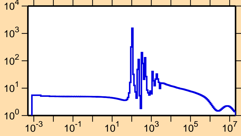
\sigma vs. E for ^{73}\text{Ge}(n,\text{el.})
