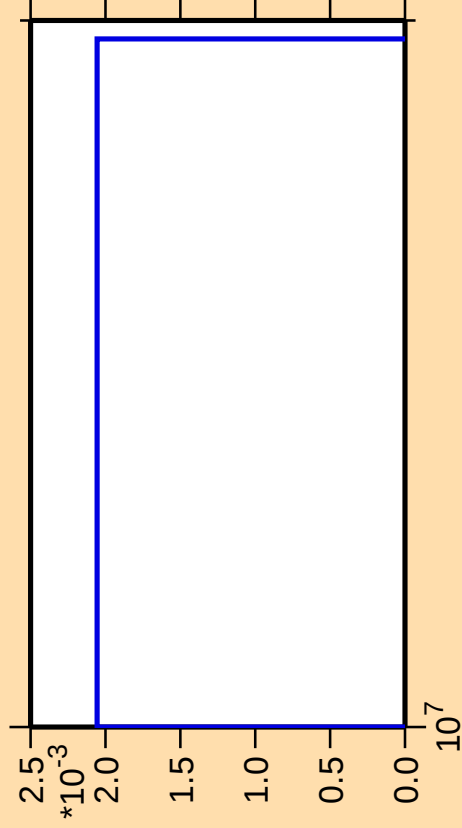
\Delta\sigma/\sigma vs. E for ^{73}\text{Ge}(n,\text{pt})
