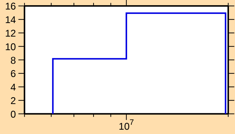
\Delta\sigma/\sigma vs. E for ^{73}\text{Ge}(n,\text{el.})
