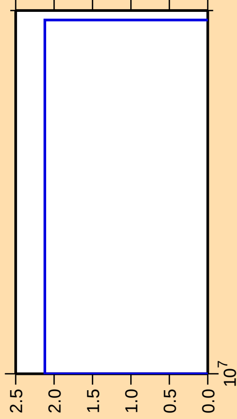
\Delta\sigma/\sigma vs. E for ^{73}\text{Ge}(n,\text{nt})
