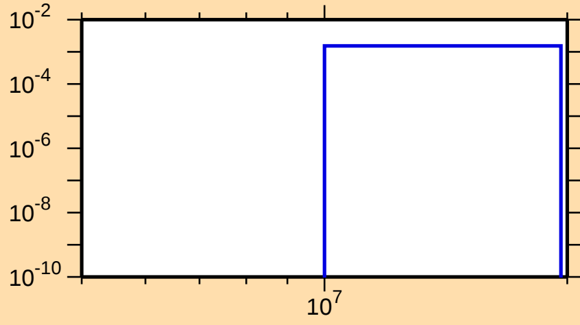
\sigma vs. E for ^{73}\text{Ge}(n,d)
