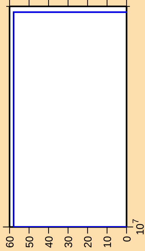
\Delta\sigma/\sigma vs. E for ^{73}\text{Ge}(n,np)
