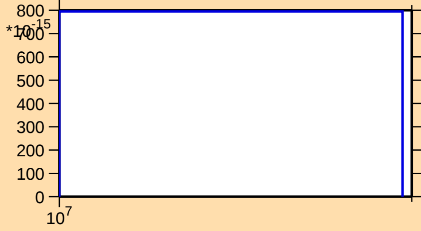
\sigma vs. E for ^{73}\text{Ge}(n,\text{nt})
