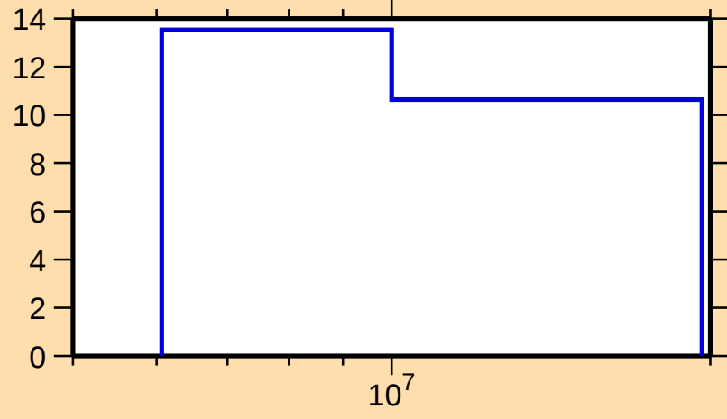
\Delta\sigma/\sigma vs. E for ^{73}\text{Ge}(n,2n)
