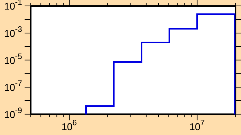
\sigma vs. E for ^{73}\text{Ge}(n,p)
