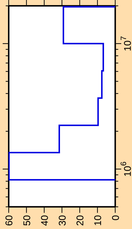
\Delta\sigma/\sigma vs. E for ^{73}\text{Ge}(n,\text{ncont.})
