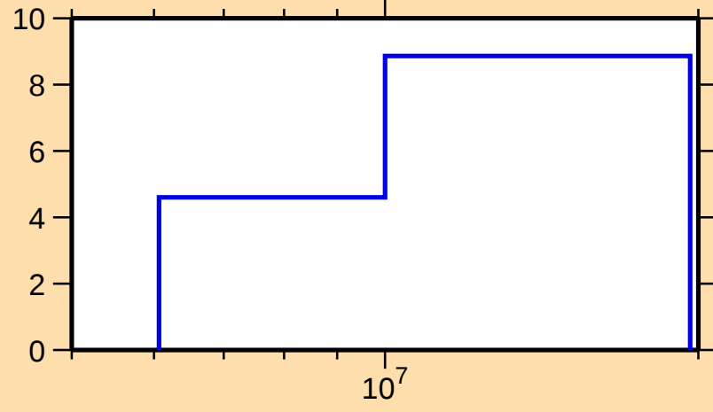
\Delta\sigma/\sigma vs. E for ^{73}\text{Ge}(n,\text{tot.})
