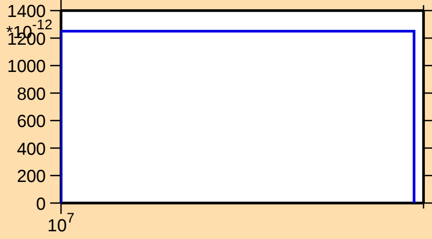
\sigma vs. E for ^{73}\text{Ge}(n,\text{He3})
