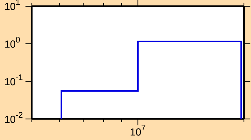
\sigma vs. E for ^{73}\text{Ge}(n,2n)
