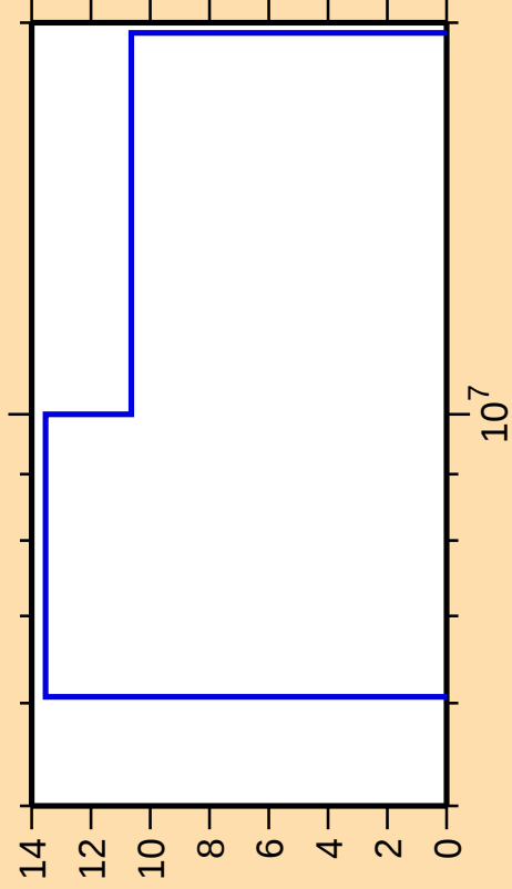
\Delta\sigma/\sigma vs. E for ^{73}\text{Ge}(n,2n)
