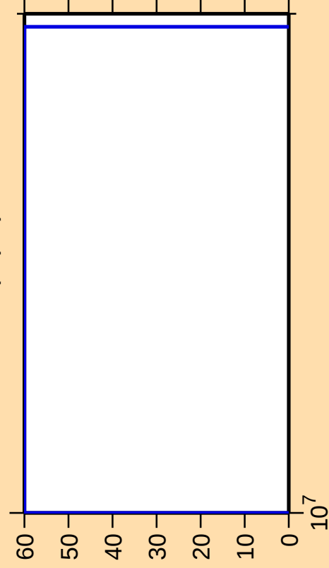
\Delta\sigma/\sigma vs. E for ^{73}\text{Ge}(n,p\alpha)
