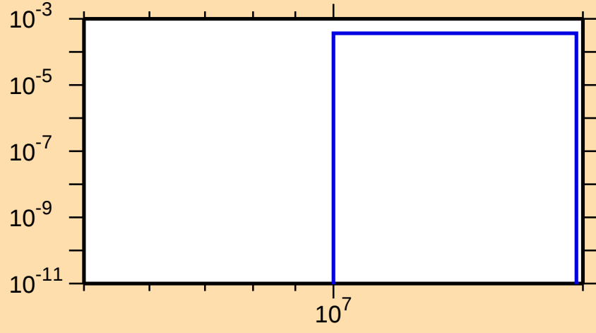
\sigma vs. E for ^{73}\text{Ge}(n,t)
