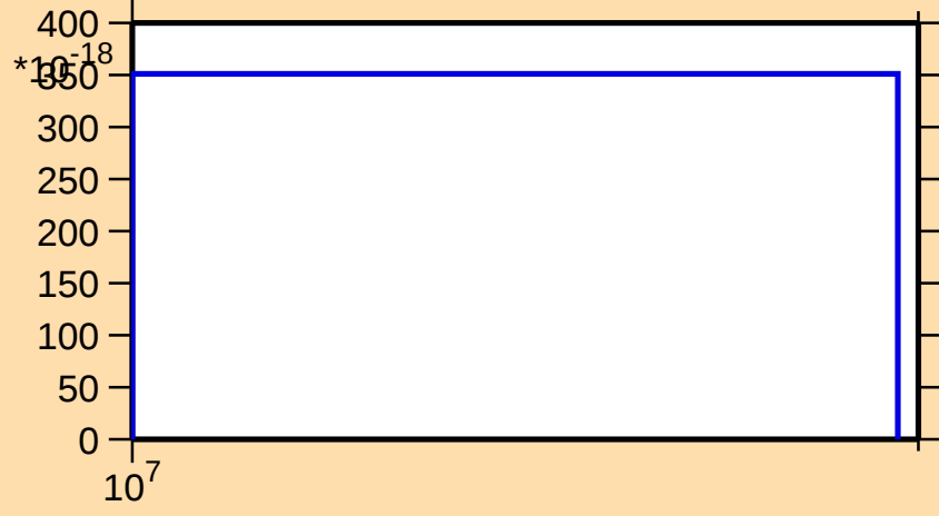
\sigma vs. E for ^{73}\text{Ge}(n,\text{pt})
