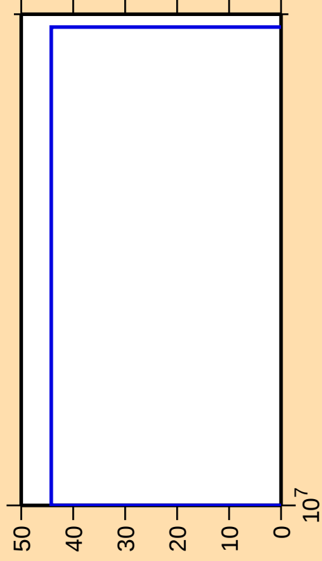
\Delta\sigma/\sigma vs. E for ^{73}\text{Ge}(n,3n)
