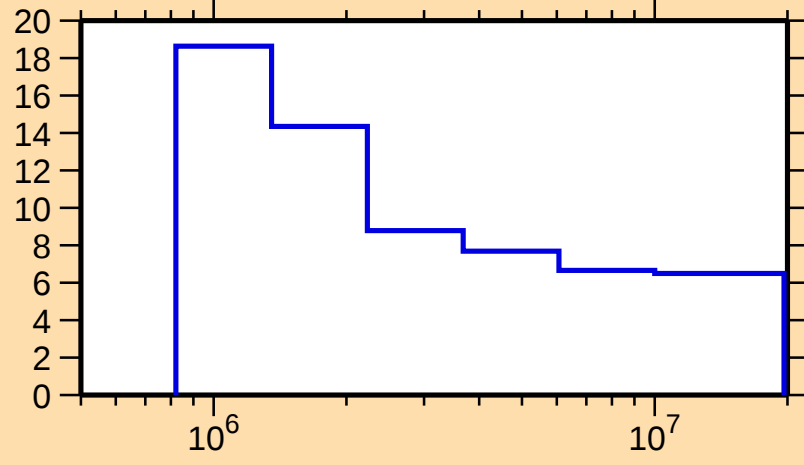
\Delta\sigma/\sigma vs. E for ^{73}\text{Ge}(n,\text{nonel.})
