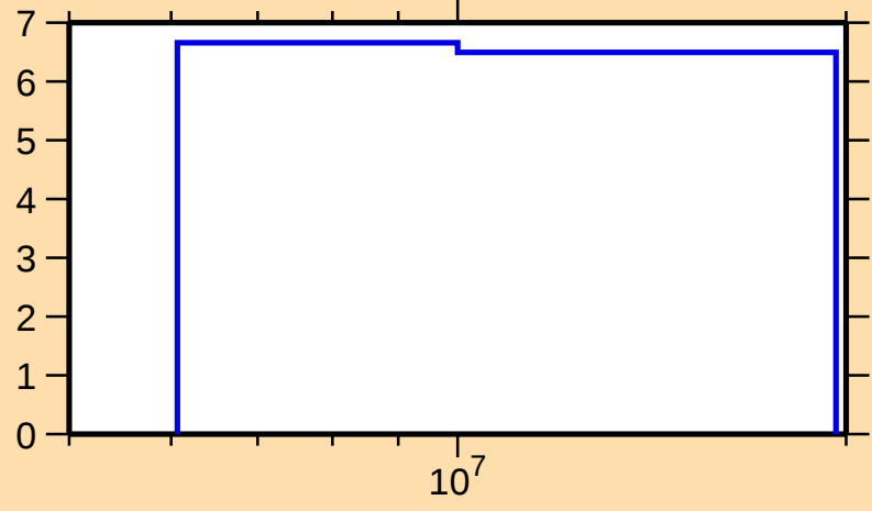
\Delta\sigma/\sigma vs. E for ^{73}\text{Ge}(n,\text{nonel.})
