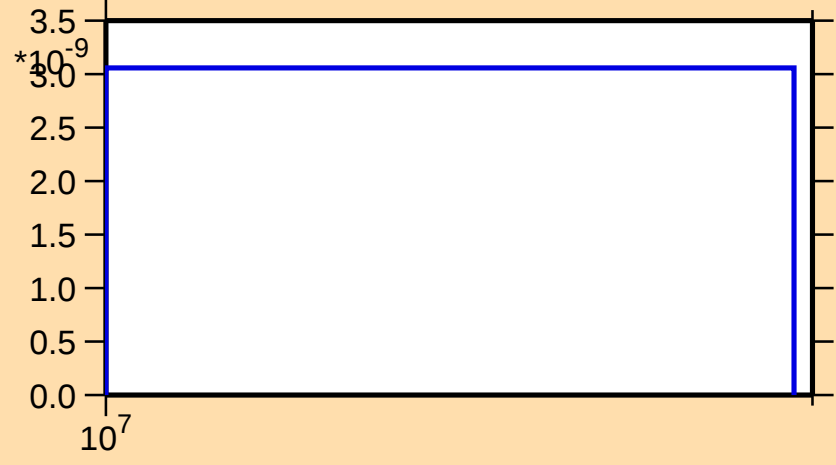
\sigma vs. E for ^{73}\text{Ge}(n,2np)
