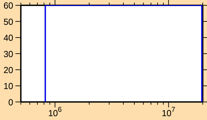
\Delta\sigma/\sigma vs. E for ^{73}\text{Ge}(n,\gamma)
