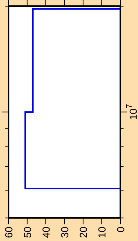
\Delta\sigma/\sigma vs. E for ^{73}\text{Ge}(n,\alpha)
