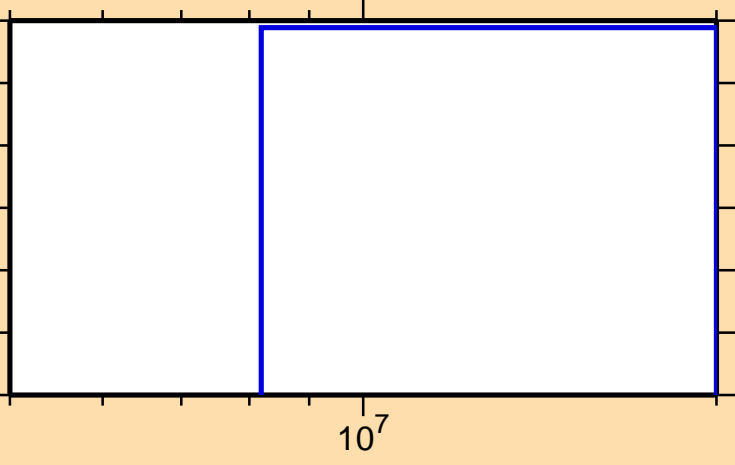
\sigma vs. E for ^{73}\text{Ge}(n,t)
