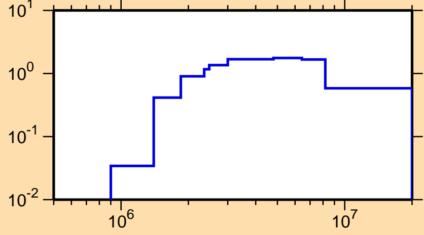
\sigma vs. E for ^{73}\text{Ge}(n,n\text{cont.})
