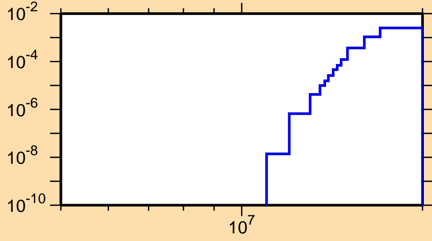
\sigma vs. E for ^{75}\text{Ge}(n,\alpha)
