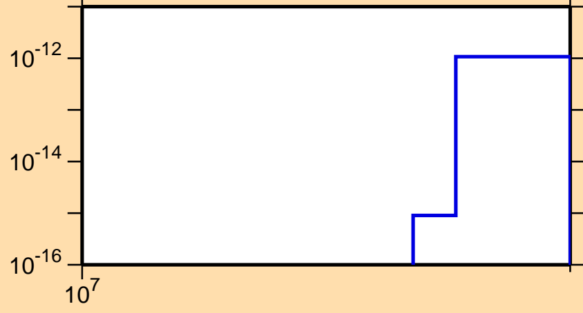
\sigma vs. E for ^{75}\text{Ge}(n,p\alpha)
