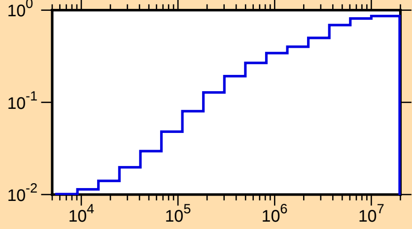
\mu vs. E for ^{76}\text{Ge}(\text{mt251})
