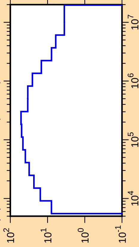
\Delta\mu/\mu vs. E for ^{76}\text{Ge}(\text{mt251})
