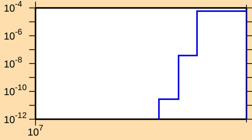
\sigma vs. E for ^{160}\text{Hf}(n,2np)
