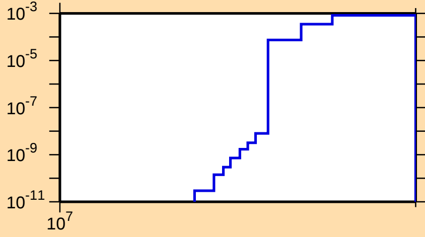
\sigma vs. E for ^{160}\text{Hf}(n,2n\alpha)
