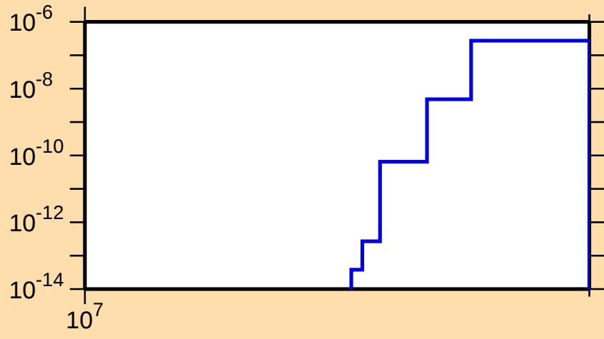
\sigma vs. E for ^{160}\text{Hf}(n,\text{nd})
