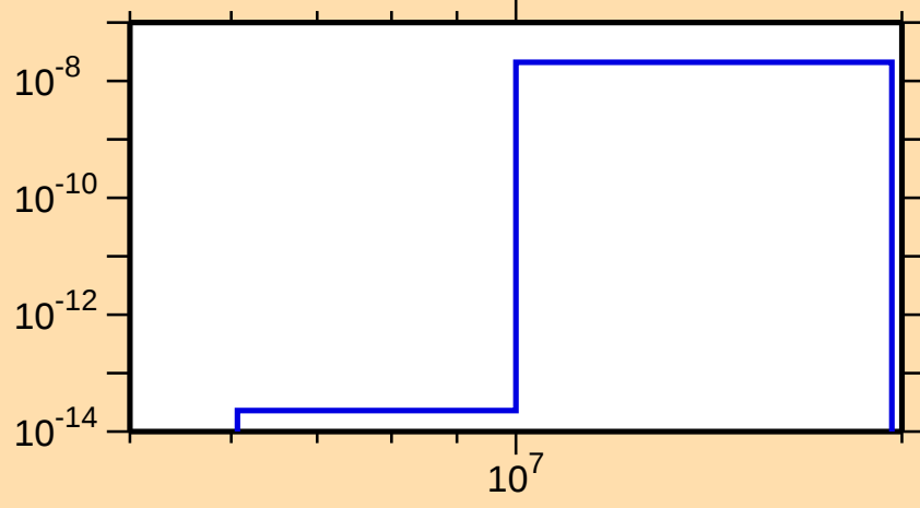
\sigma vs. E for ^{160}\text{Hf}(\text{mt117})
