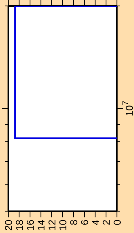
\Delta\sigma/\sigma vs. E for ^{160}\text{Hf}(\text{mt } 34)
