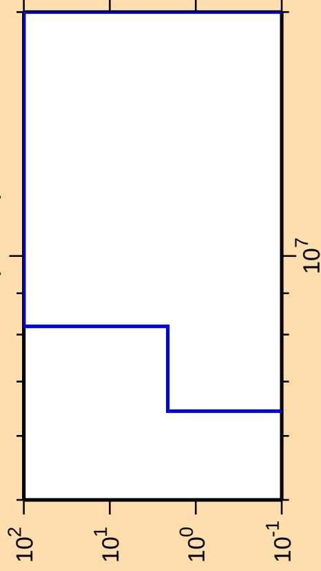
\Delta\sigma/\sigma vs. E for ^{160}\text{Hf}(\text{mt } 45)
