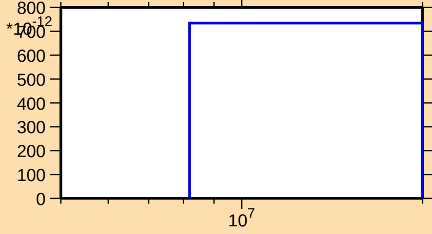
\sigma vs. E for ^{160}\text{Hf}(n,\text{pt})
