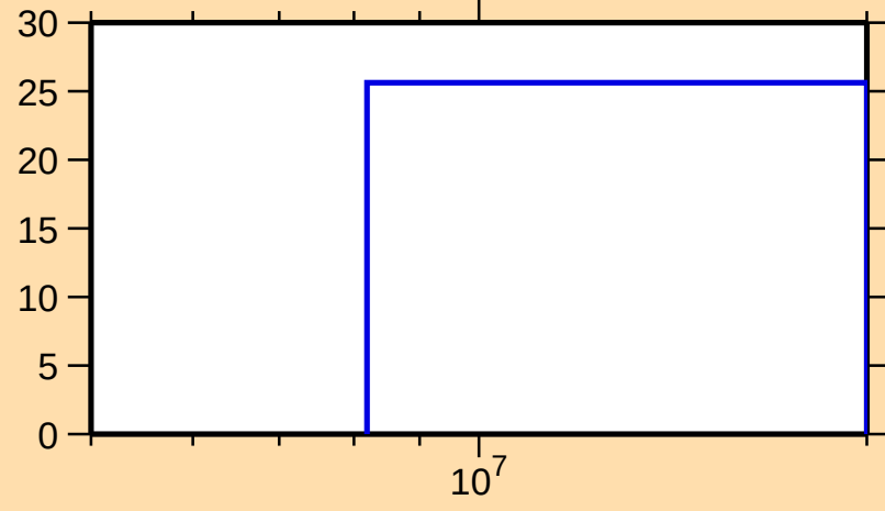
\Delta\sigma/\sigma vs. E for ^{160}\text{Hf}(n,\text{nonel.})
