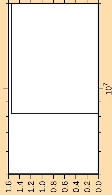
\Delta\sigma/\sigma vs. E for ^{160}\text{Hf}(n,nt)
