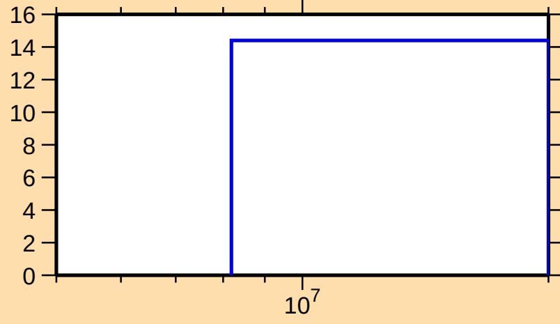
\Delta\sigma/\sigma vs. E for ^{160}\text{Hf}(n,\text{tot.})
