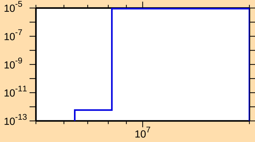
\sigma vs. E for ^{160}\text{Hf}(\text{mt } 45)
