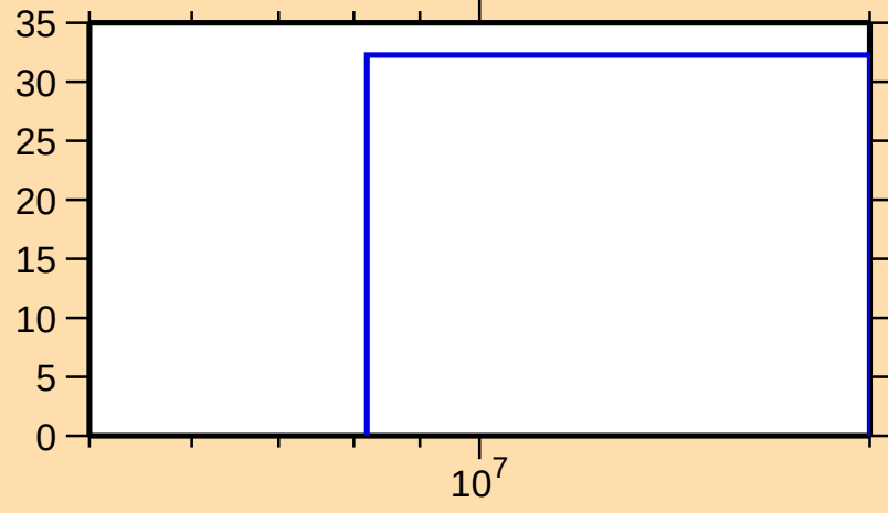
\Delta\sigma/\sigma vs. E for ^{160}\text{Hf}(n,\text{el.})
