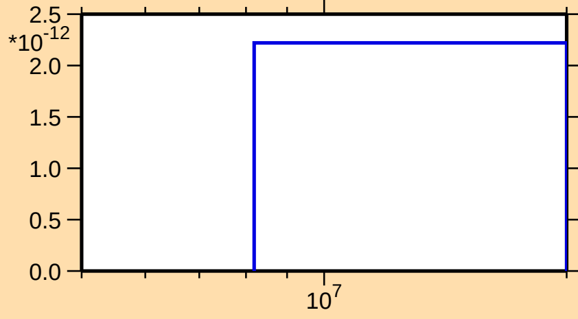
\sigma vs. E for ^{160}\text{Hf}(\text{mt } 34)
