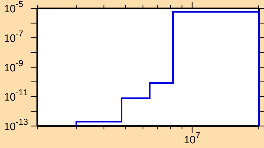
\sigma vs. E for ^{160}\text{Hf}(n,\text{He3})
