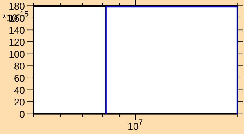
\sigma vs. E for ^{160}\text{Hf}(n,nt)
