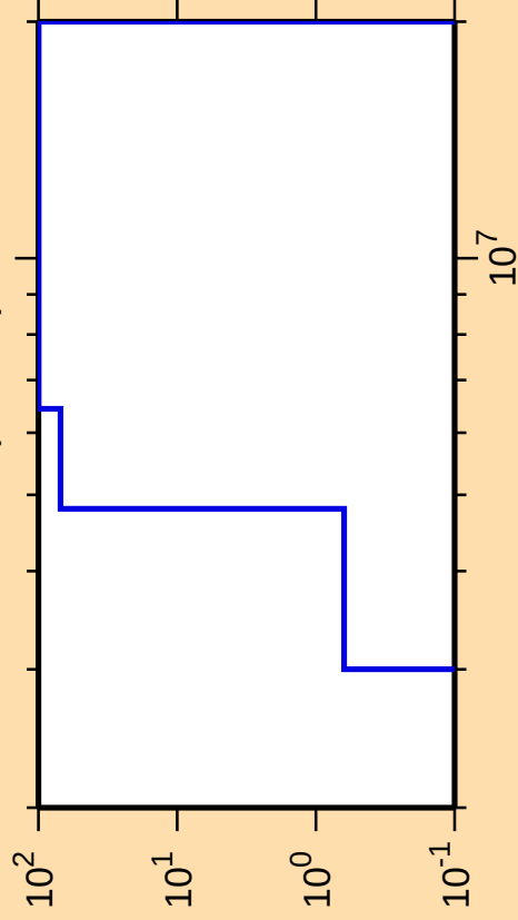
\Delta\sigma/\sigma vs. E for ^{160}\text{Hf}(n,\text{He3})
