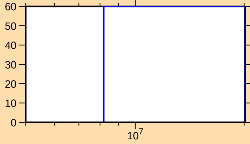
\Delta\sigma/\sigma vs. E for ^{160}\text{Hf}(n,\text{inel.})
