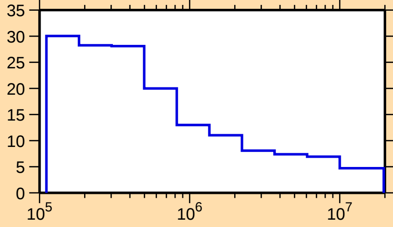
\Delta\sigma/\sigma vs. E for ^{166}\text{Hf}(n,\text{nonel.})
