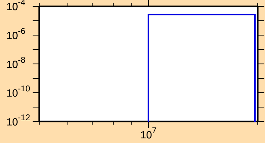
\sigma vs. E for ^{166}\text{Hf}(n,t)
