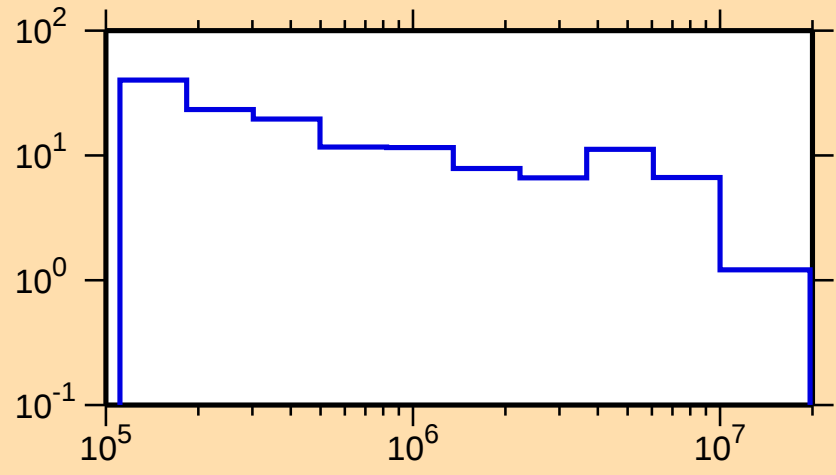
\Delta\sigma/\sigma vs. E for ^{166}\text{Hf}(n,\text{tot.})
