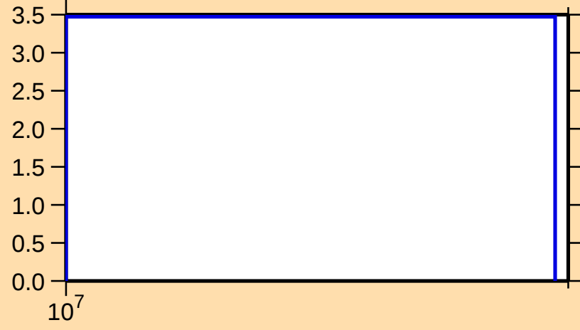
\Delta\sigma/\sigma vs. E for ^{166}\text{Hf}(n,\text{el.})
