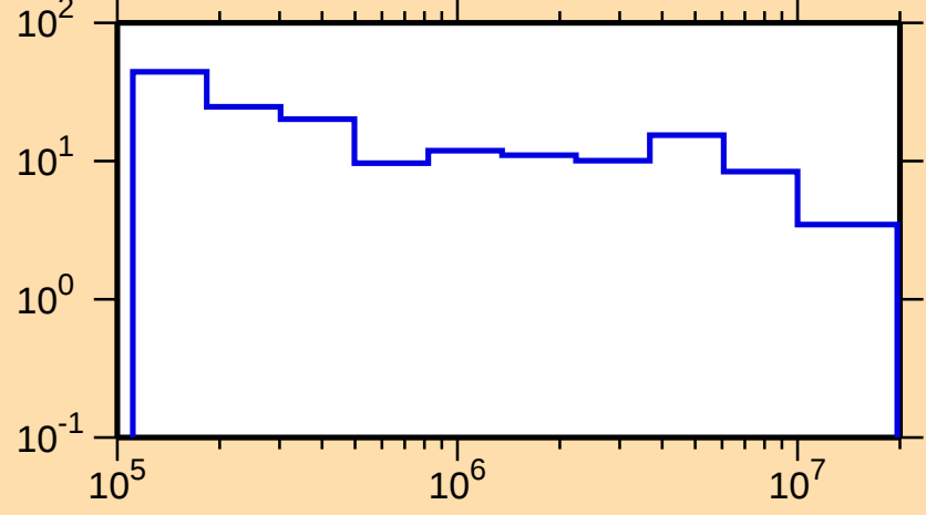
\Delta\sigma/\sigma vs. E for ^{166}\text{Hf}(n,\text{el.})
