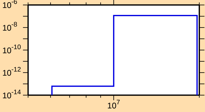
\sigma vs. E for ^{166}\text{Hf}(n,\text{He3})
