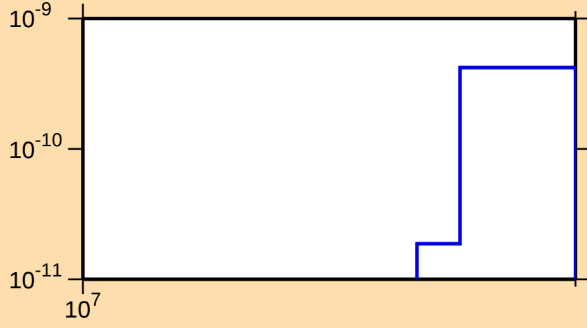
\sigma vs. E for ^{170}\text{Hf}(n,\text{pd})
