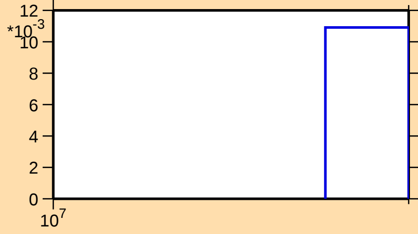
\sigma vs. E for ^{170}\text{Hf}(n,3n)
