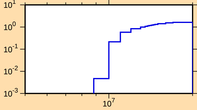
\sigma vs. E for ^{170}\text{Hf}(n,2n)
