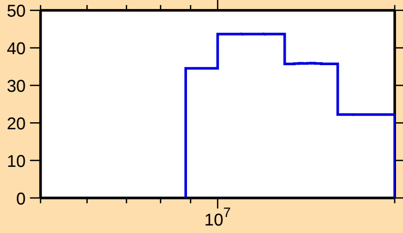
\Delta\sigma/\sigma vs. E for ^{170}\text{Hf}(n,\text{inel.})
