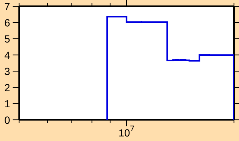
\Delta\sigma/\sigma vs. E for ^{170}\text{Hf}(n,\text{tot.})
