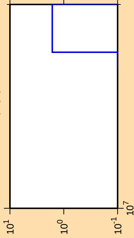
\Delta\sigma/\sigma vs. E for ^{170}\text{Hf}(n,\text{pt})
