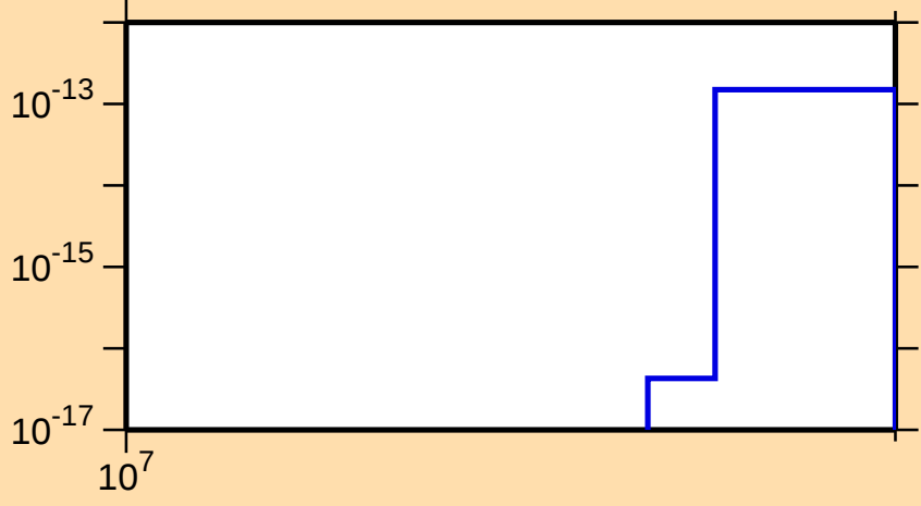
\sigma vs. E for ^{170}\text{Hf} (mt 34)
