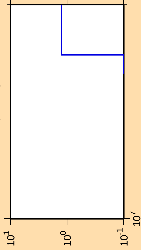
\Delta\sigma/\sigma vs. E for ^{170}\text{Hf} (mt 34)
