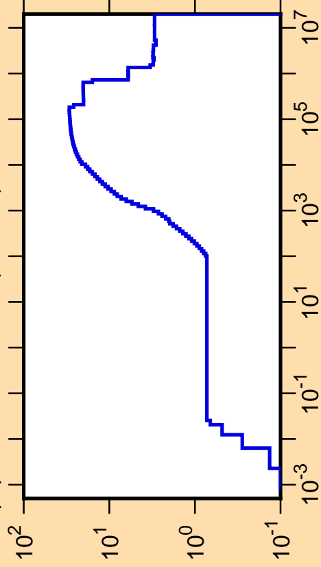
\Delta\mu/\mu vs. E for ^{174}\text{Hf}(\text{mt251})
