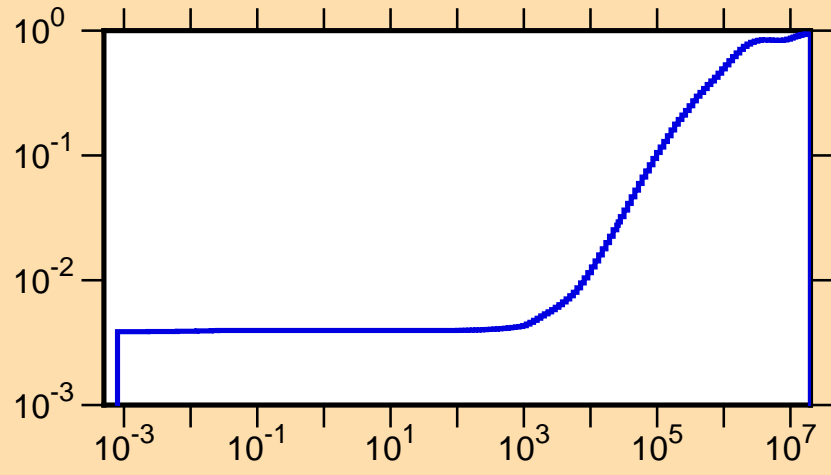
\mu vs. E for ^{174}\text{Hf}(\text{mt251})
