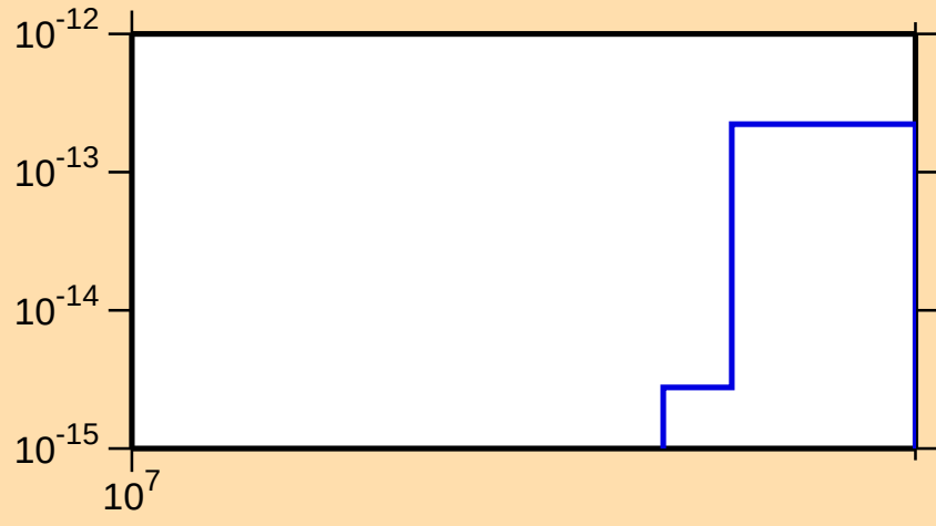
\sigma vs. E for ^{174}\text{Hf}(n,\text{pd})
