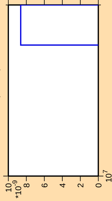
\Delta\sigma/\sigma vs. E for ^{174}\text{Hf}(\text{mt } 11)
