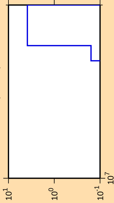
\Delta\sigma/\sigma vs. E for ^{174}\text{Hf}(\text{mt117})
