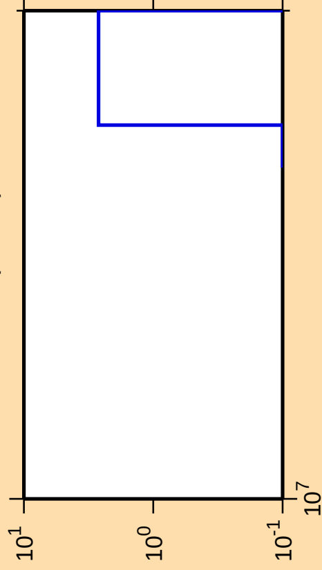
\Delta\sigma/\sigma vs. E for ^{174}\text{Hf}(\text{mt 45})
