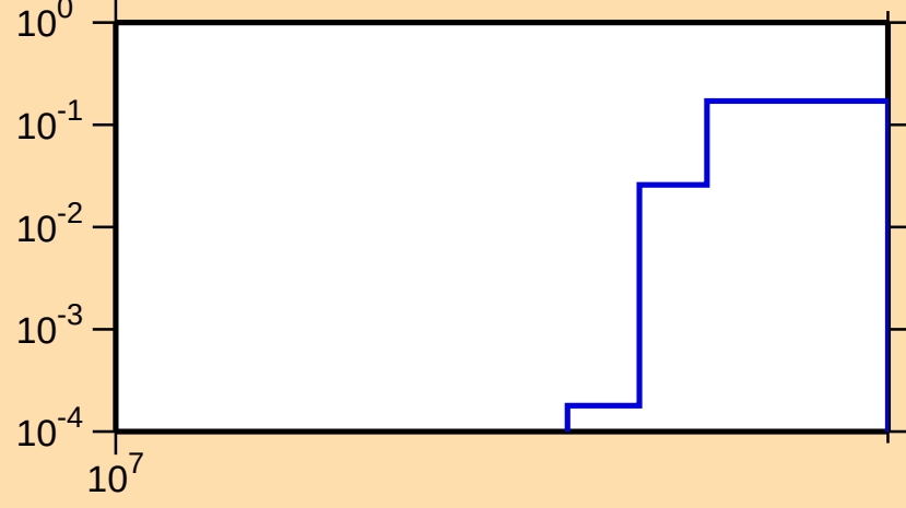
\sigma vs. E for ^{174}\text{Hf}(n,3n)
