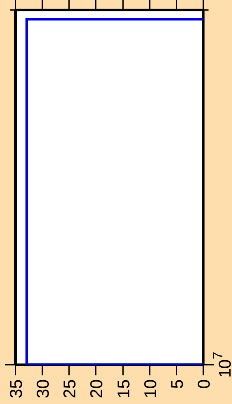
\Delta\sigma/\sigma vs. E for ^{174}\text{Hf}(n,3n)
