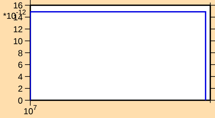
\sigma vs. E for ^{174}\text{Hf}(n,p\alpha)
