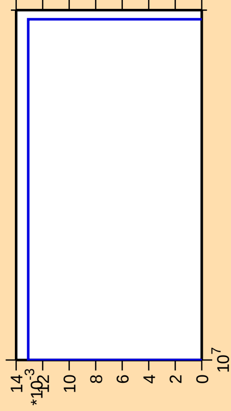
\Delta\sigma/\sigma vs. E for ^{174}\text{Hf}(n,\text{pd})
