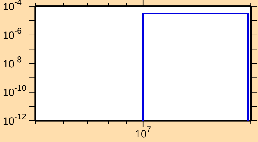
\sigma vs. E for ^{174}\text{Hf}(n,t)
