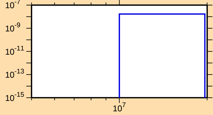
\sigma vs. E for ^{174}\text{Hf}(n,2n\alpha)
