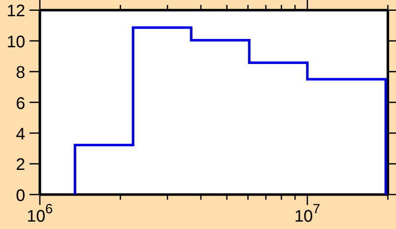
\Delta\sigma/\sigma vs. E for ^{174}\text{Hf}(\text{n},\text{el.})
