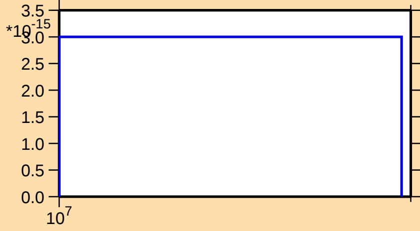
\sigma vs. E for ^{174}\text{Hf}(\text{mt } 45)
