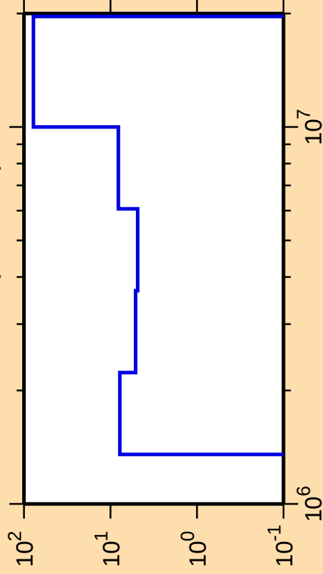
\Delta\sigma/\sigma vs. E for ^{174}\text{Hf}(\text{n},\text{ncont.})
