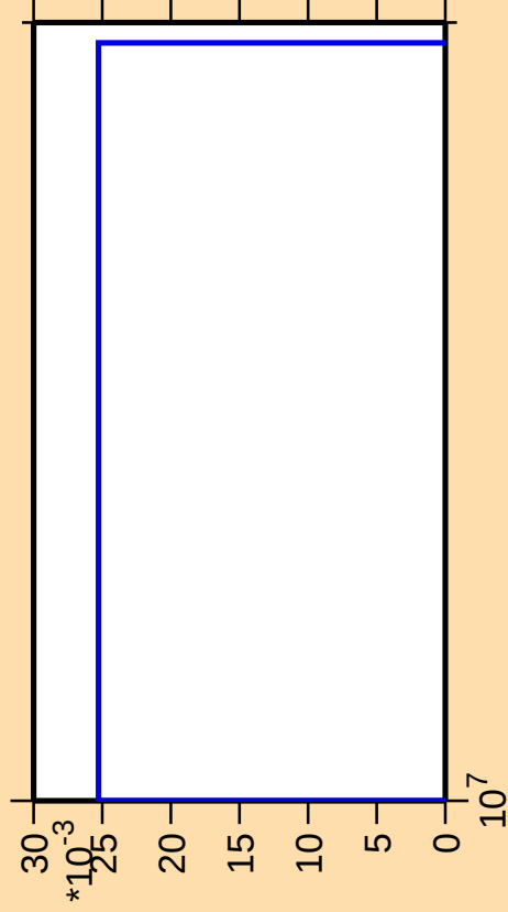
\Delta\sigma/\sigma vs. E for ^{174}\text{Hf}(\text{mt } 45)
