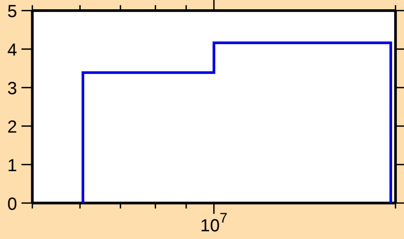
\Delta\sigma/\sigma vs. E for ^{174}\text{Hf}(n,\text{nonel.})
