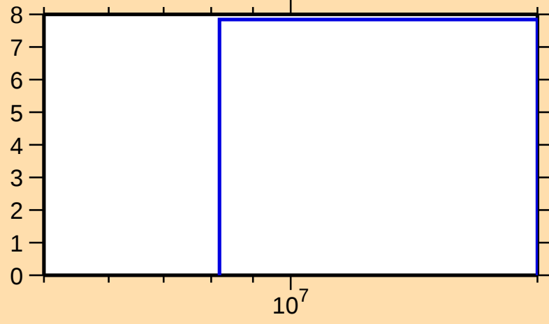
\Delta\sigma/\sigma vs. E for ^{174}\text{Hf}(n,\text{el.})
