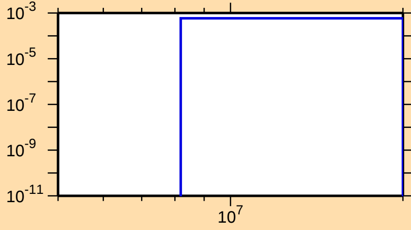
\sigma vs. E for ^{174}\text{Hf}(n,np)
