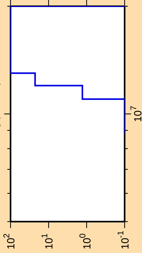
\Delta\sigma/\sigma vs. E for ^{181}\text{Hg}(\text{mt } 34)
