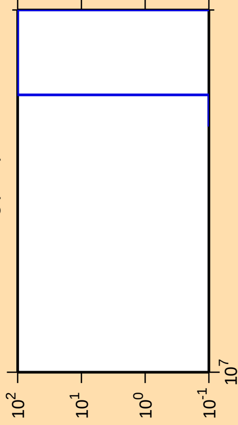
\Delta\sigma/\sigma vs. E for ^{181}\text{Hg}(n,\text{nt})
