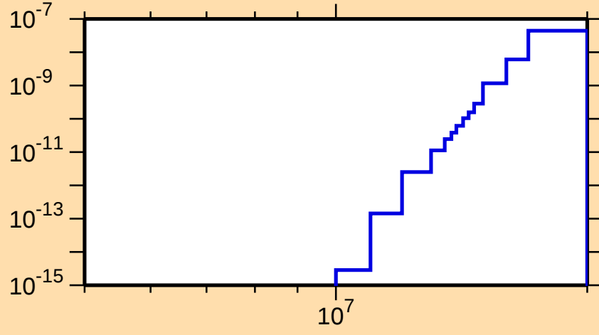
\sigma vs. E for ^{181}\text{Hg}(\text{mt } 34)
