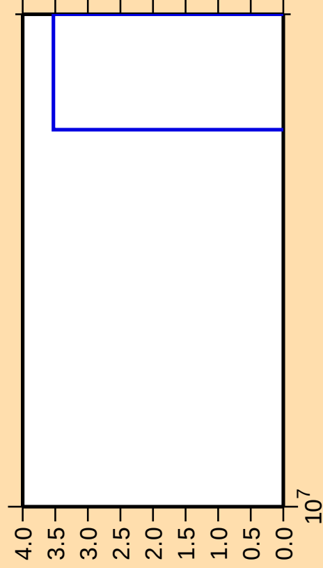
\Delta\sigma/\sigma vs. E for ^{181}\text{Hg}(n,3n)
