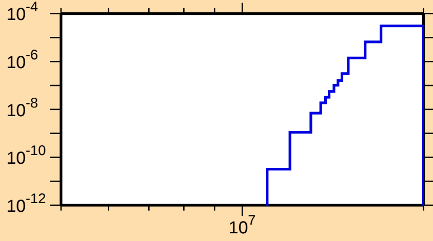
\sigma vs. E for ^{181}\text{Hg}(n,\text{pt})
