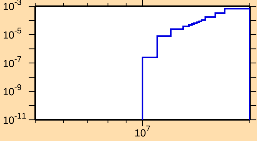
\sigma vs. E for ^{181}\text{Hg}(n,2n\alpha)
