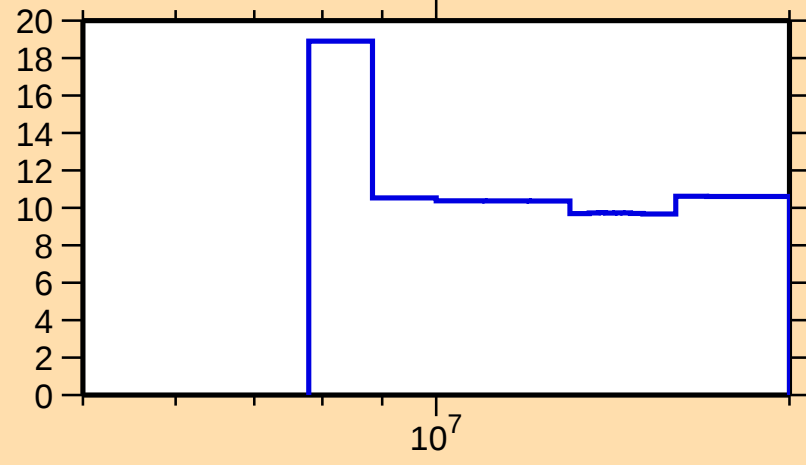
\Delta\sigma/\sigma vs. E for ^{181}\text{Hg}(n,\text{el.})
