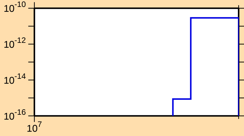
\sigma vs. E for ^{181}\text{Hg}(n,\text{nt})
