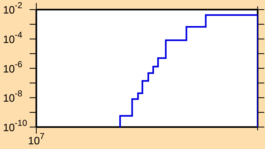
\sigma vs. E for ^{181}\text{Hg}(n,2np)
