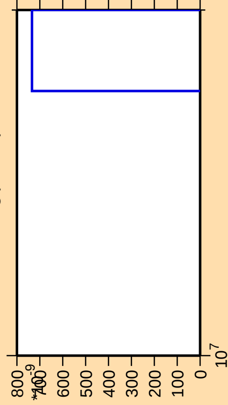
\Delta\sigma/\sigma vs. E for ^{181}\text{Hg} (mt 11)
