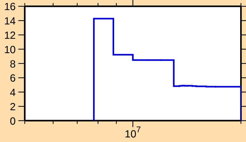
\Delta\sigma/\sigma vs. E for ^{181}\text{Hg}(n,\text{tot.})
