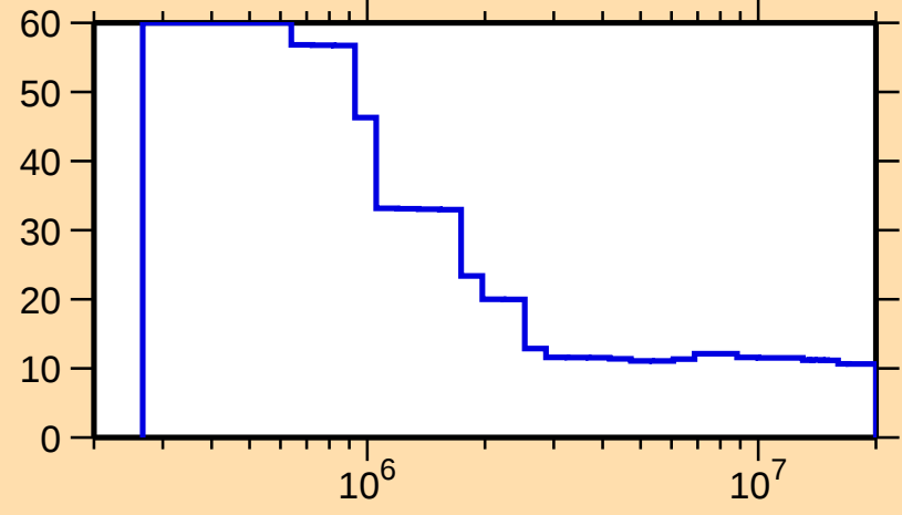
\Delta\sigma/\sigma vs. E for ^{181}\text{Hg}(n,n\text{onel.})
