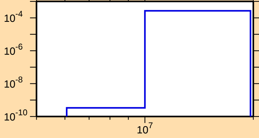
\sigma vs. E for ^{181}\text{Hg}(n,t)
