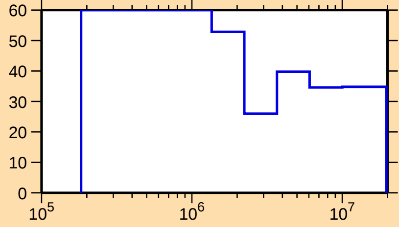
\Delta\sigma/\sigma vs. E for ^{181}\text{Hg}(n,n_1)
