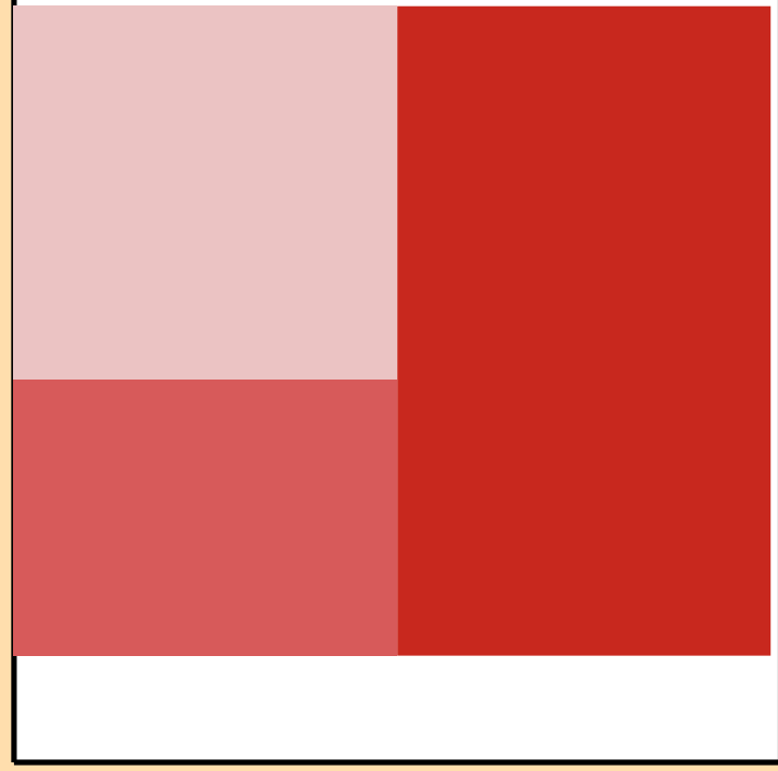
\Delta\sigma/\sigma vs. E for ^{181}\text{Hg}(n,\text{nonel.})
