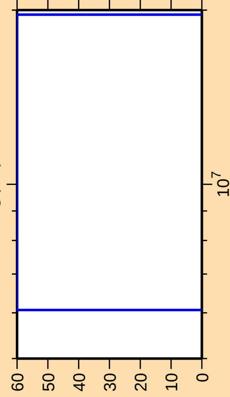
\Delta\sigma/\sigma vs. E for ^{181}\text{Hg}(n,t)
