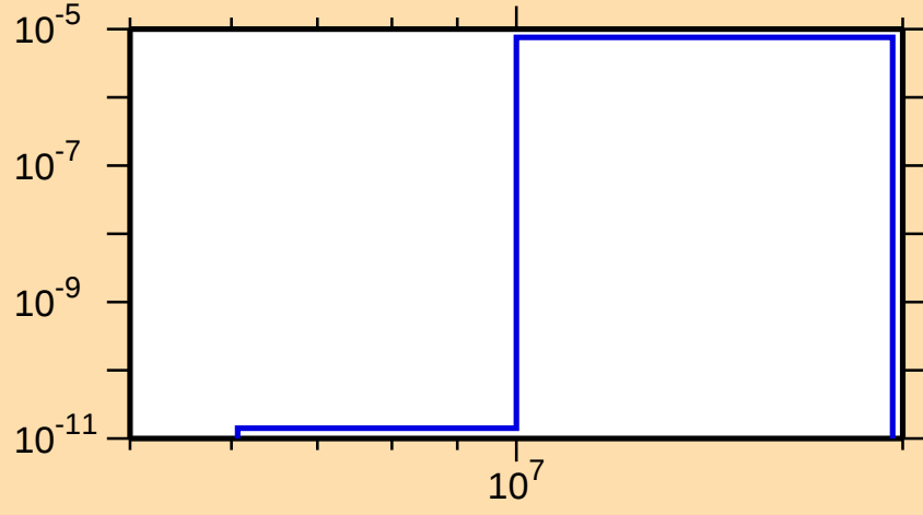
\sigma vs. E for ^{181}\text{Hg}(n,\text{pd})
