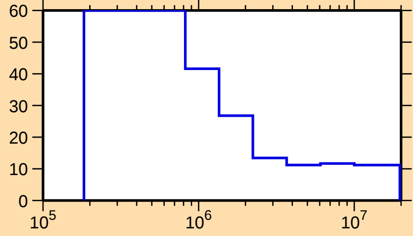
\Delta\sigma/\sigma vs. E for ^{181}\text{Hg}(\text{n},\text{nonel.})
