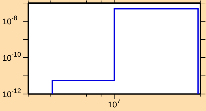
\sigma vs. E for ^{181}\text{Hg}(\text{mt117})
