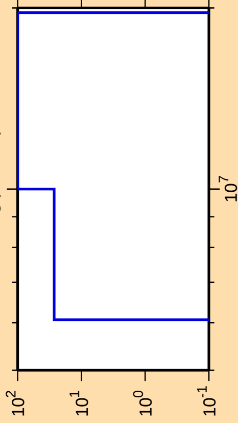
\Delta\sigma/\sigma vs. E for ^{181}\text{Hg}(\text{mt117})
