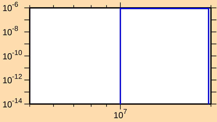
\sigma vs. E for ^{181}\text{Hg}(n,\text{pt})
