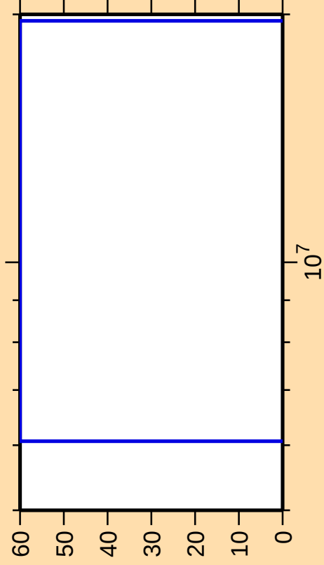
\Delta\sigma/\sigma vs. E for ^{181}\text{Hg}(n,\text{pd})
