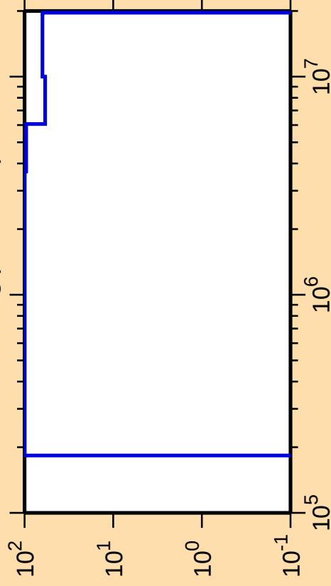
\Delta\sigma/\sigma vs. E for ^{181}\text{Hg}(\text{n},\text{ncont.})
