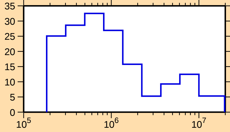
\Delta\sigma/\sigma vs. E for ^{181}\text{Hg}(\text{n},\text{tot.})
