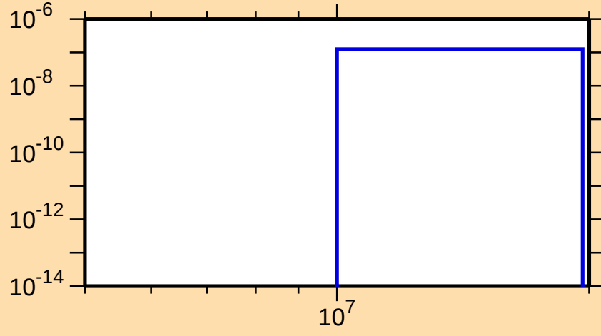
\sigma vs. E for ^{181}\text{Hg}(n,\text{nd})
