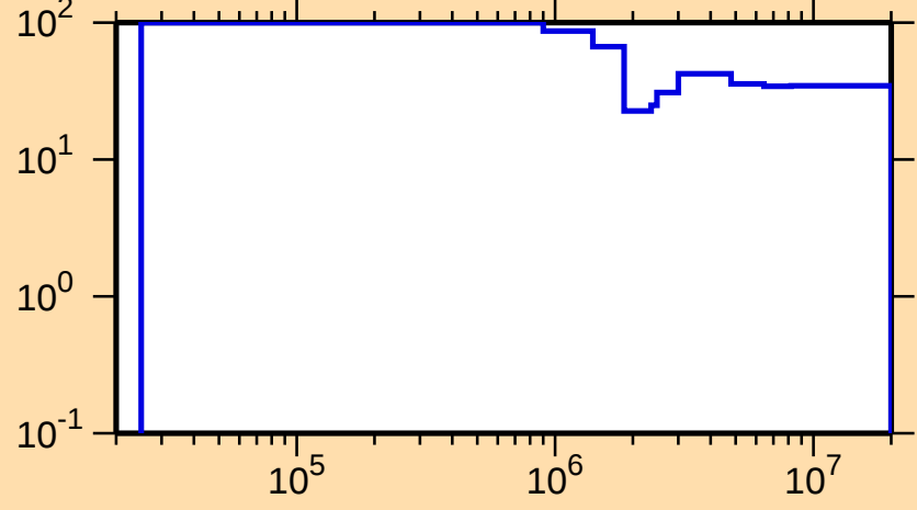
\Delta\sigma/\sigma vs. E for ^{181}\text{Hg}(n,n_1)
