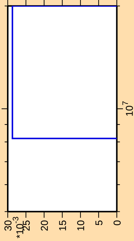
\Delta\sigma/\sigma vs. E for ^{181}\text{Hg}(n,3n)
