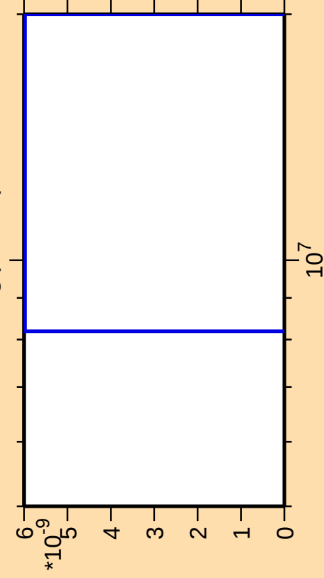
\Delta\sigma/\sigma vs. E for ^{181}\text{Hg}(\text{mt } 11)
