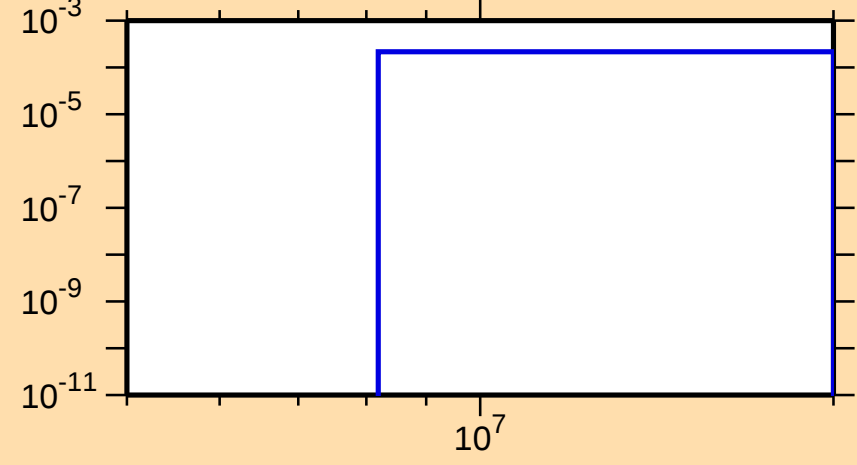
\sigma vs. E for ^{181}\text{Hg}(n,t)
