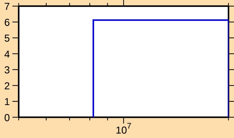
\Delta\sigma/\sigma vs. E for ^{181}\text{Hg}(n,\text{tot.})
