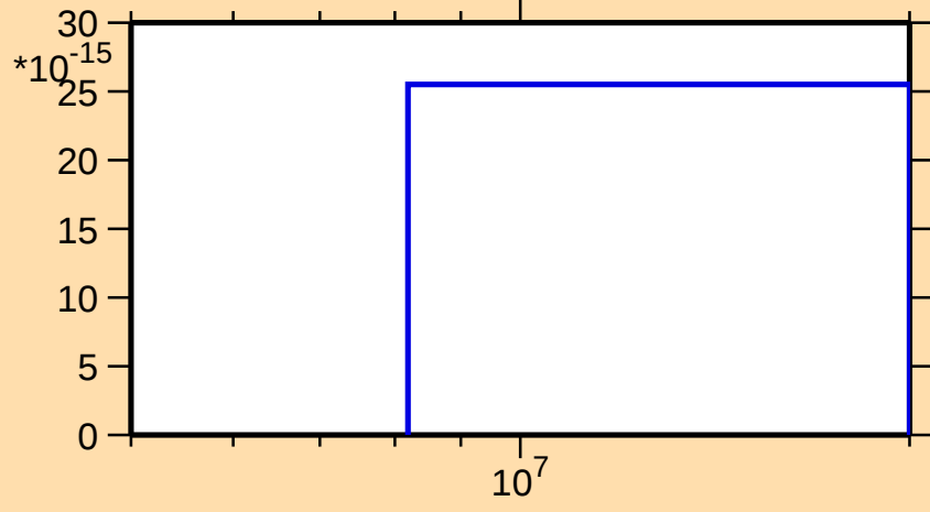
\sigma vs. E for ^{181}\text{Hg}(n,3n)
