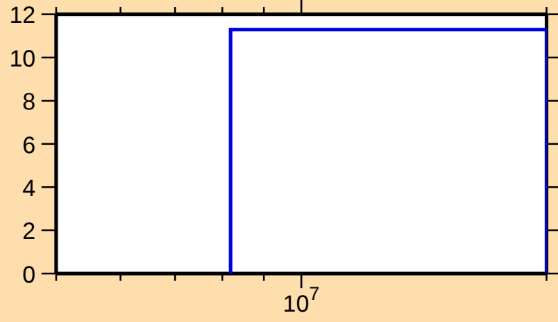
\Delta\sigma/\sigma vs. E for ^{181}\text{Hg}(n,\text{nonel.})
