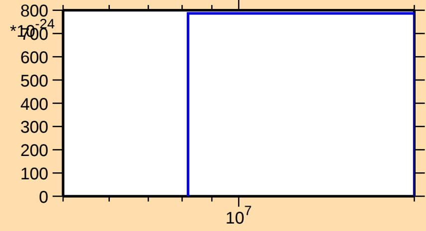
\sigma vs. E for ^{181}\text{Hg}(\text{mt } 11)
