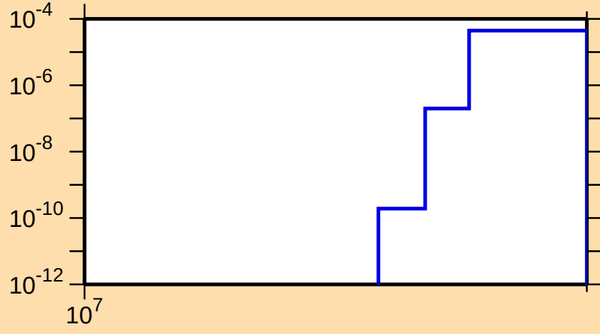
\sigma vs. E for ^{182}\text{Hg}(n,2np)
