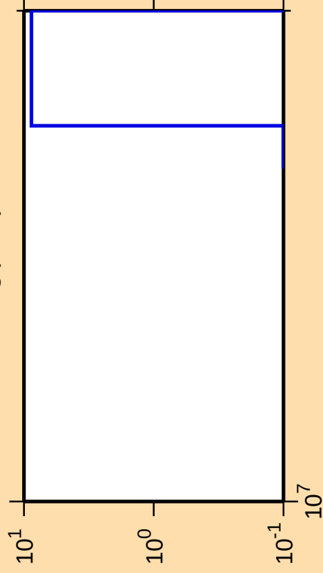
\Delta\sigma/\sigma vs. E for ^{182}\text{Hg}(n,\text{nt})
