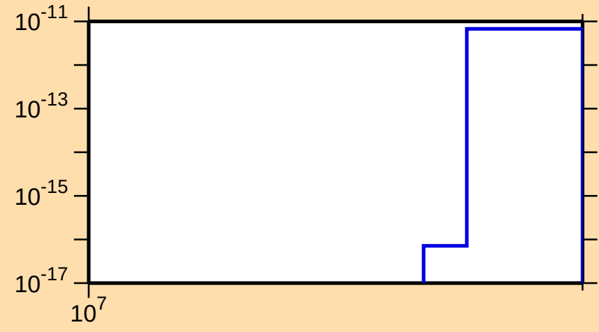
\sigma vs. E for ^{182}\text{Hg}(n,\text{nt})
