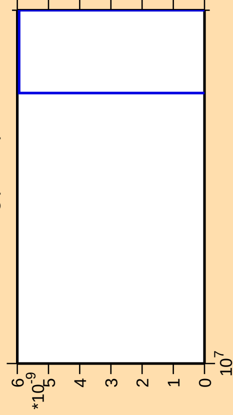
\Delta\sigma/\sigma vs. E for ^{182}\text{Hg} (mt 11)
