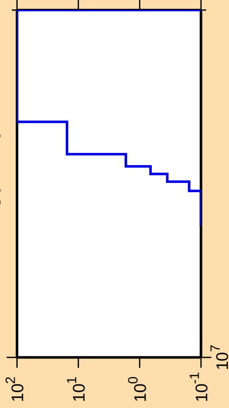
\Delta\sigma/\sigma vs. E for ^{182}\text{Hg}(\text{mt } 34)
