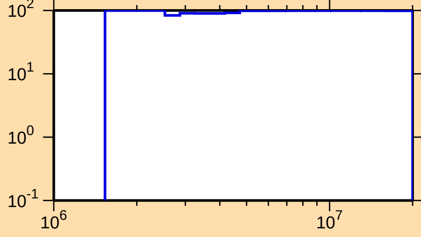
\Delta\sigma/\sigma vs. E for ^{182}\text{Hg}(n,n\text{cont.})
