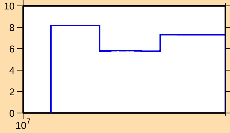
\Delta\sigma/\sigma vs. E for ^{182}\text{Hg}(n,\text{tot.})
