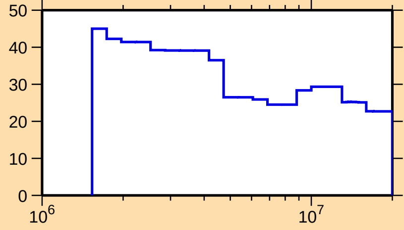
\Delta\sigma/\sigma vs. E for ^{182}\text{Hg}(\text{n},\text{nonel.})
