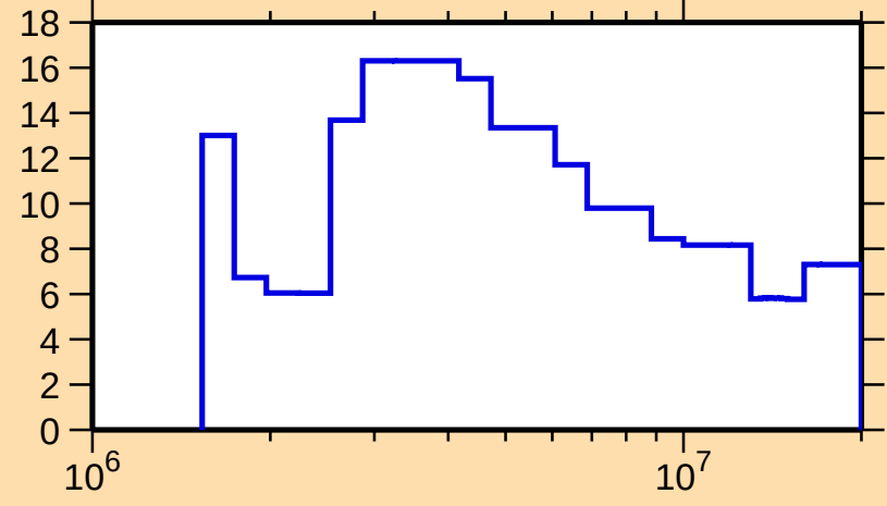
\Delta\sigma/\sigma vs. E for ^{182}\text{Hg}(\text{n},\text{tot.})
