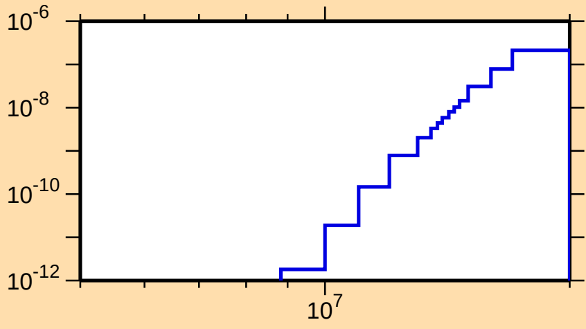
\sigma vs. E for ^{182}\text{Hg}(\text{mt117})
