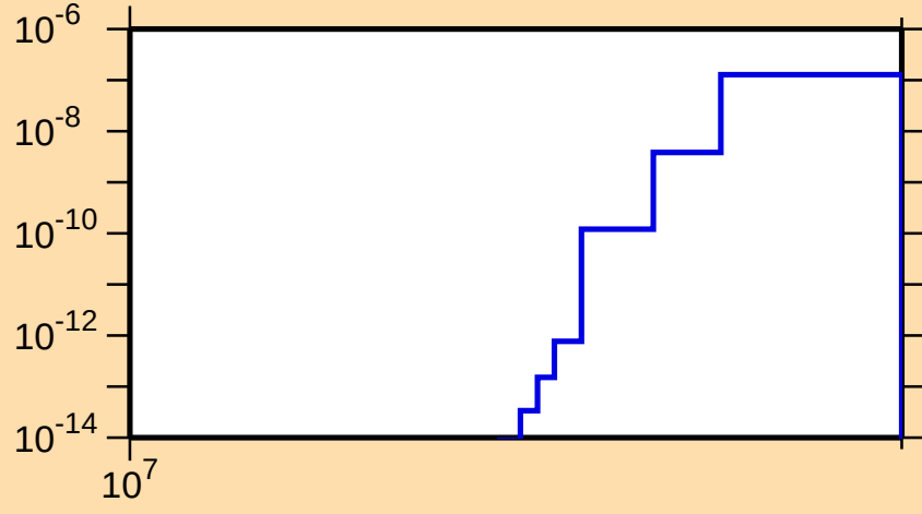
\sigma vs. E for ^{182}\text{Hg}(n,\text{nd})
