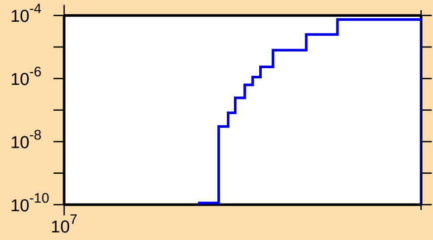
\sigma vs. E for ^{182}\text{Hg}(n,2n\alpha)
