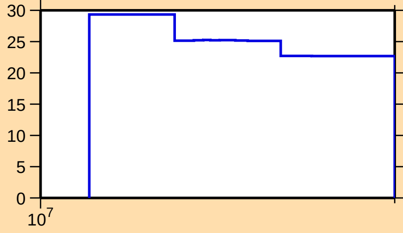
\Delta\sigma/\sigma vs. E for ^{182}\text{Hg}(n,\text{nonel.})
