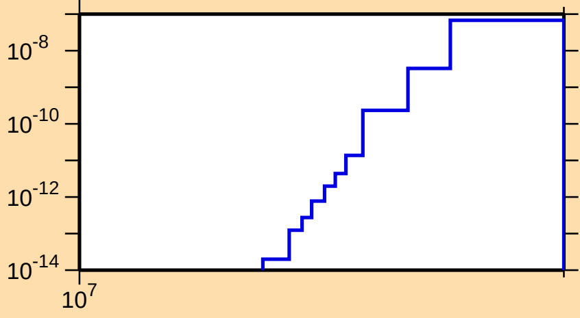
\sigma vs. E for ^{182}\text{Hg}(n,\text{pt})
