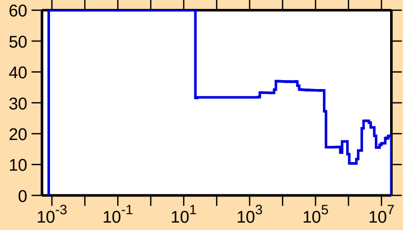
\Delta\sigma/\sigma vs. E for ^{182}\text{Hg}(n,\text{el.})
