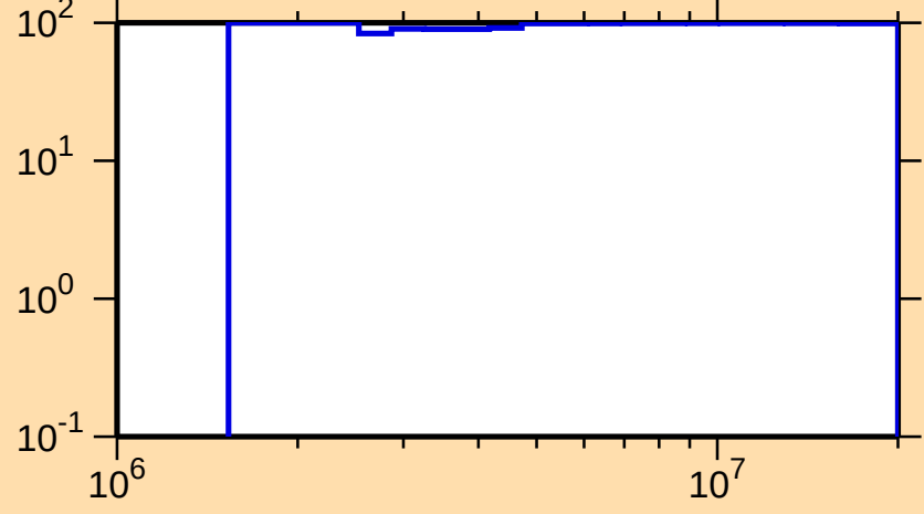
\Delta\sigma/\sigma vs. E for ^{182}\text{Hg}(n,n\text{cont.})
