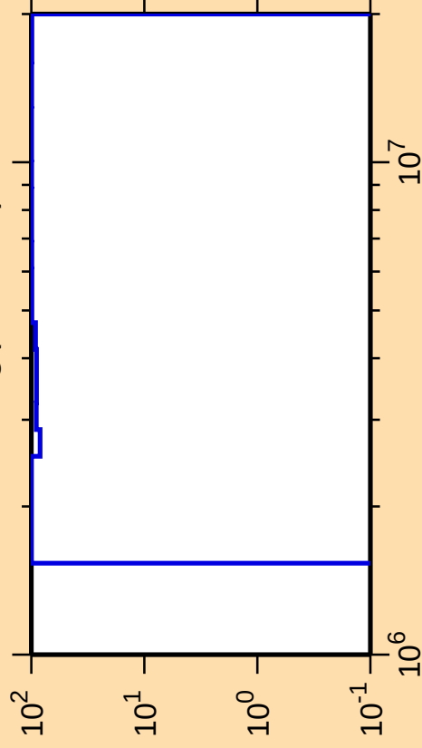
\Delta\sigma/\sigma vs. E for ^{182}\text{Hg}(\text{n},\text{ncont.})
