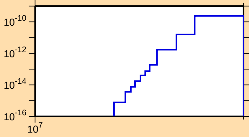
\sigma vs. E for ^{182}\text{Hg}(\text{mt } 34)
