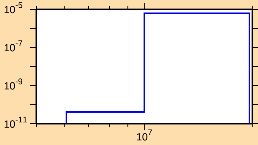
\sigma vs. E for ^{182}\text{Hg}(\text{mt } 45)
