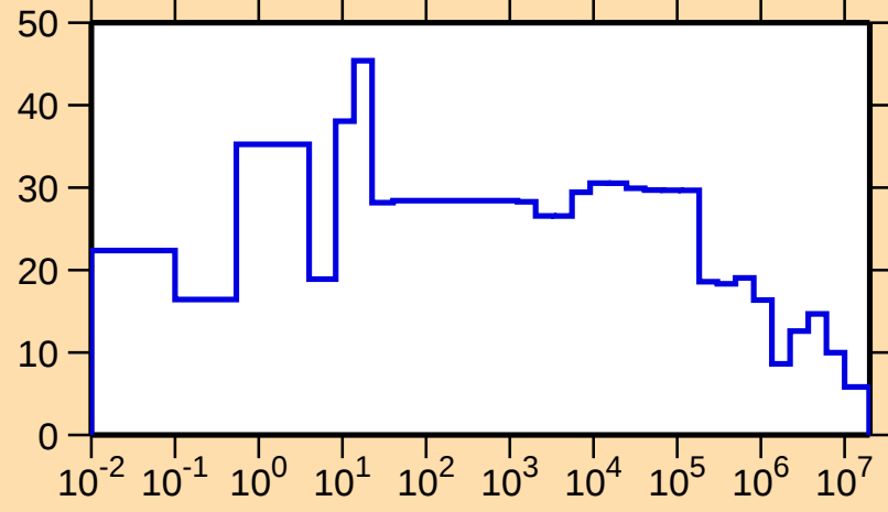
\Delta\sigma/\sigma vs. E for ^{182}\text{Hg}(\text{n,tot.})
