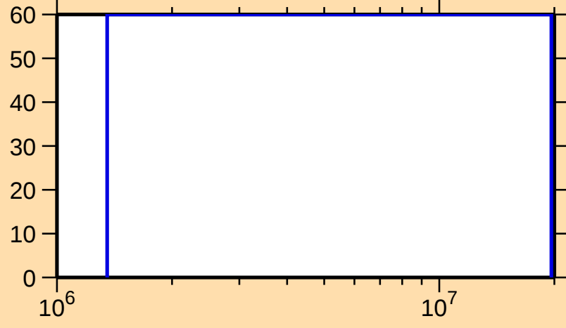
\Delta\sigma/\sigma vs. E for ^{182}\text{Hg}(n,\text{ncont.})
