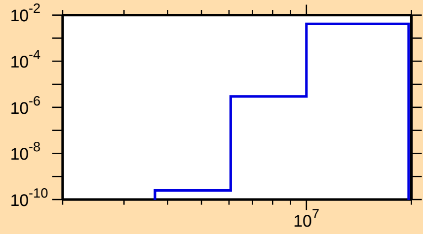
\sigma vs. E for ^{182}\text{Hg}(n,d)
