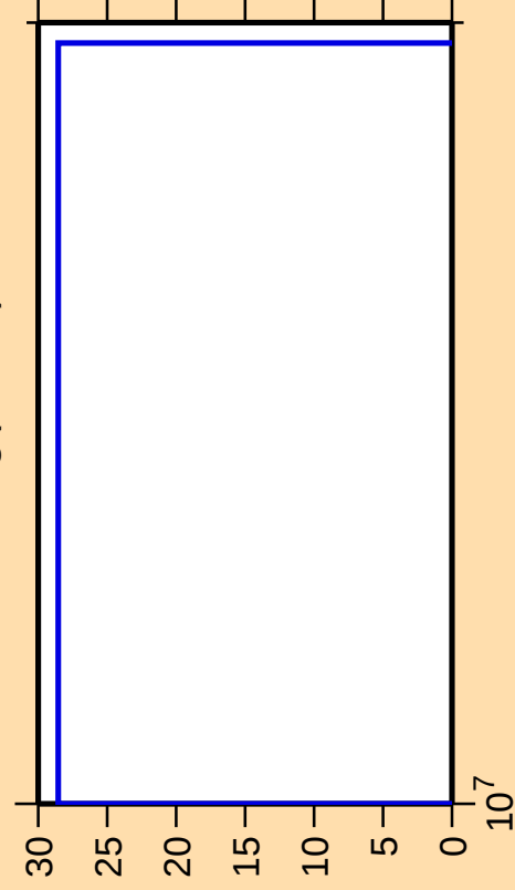
\Delta\sigma/\sigma vs. E for ^{182}\text{Hg} (mt 34)
