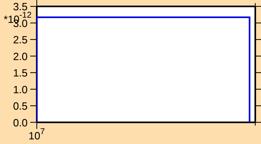
\sigma vs. E for ^{182}\text{Hg} (mt 34)
