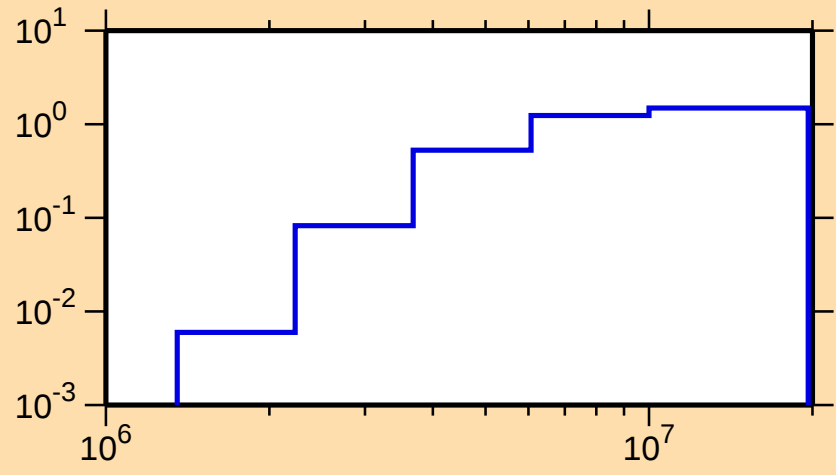
\sigma vs. E for ^{182}\text{Hg}(n,n\text{cont.})
