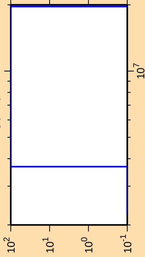
\Delta\sigma/\sigma vs. E for ^{182}\text{Hg}(n,d)
