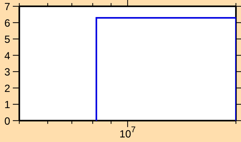
\Delta\sigma/\sigma vs. E for ^{182}\text{Hg}(n,\text{tot.})
