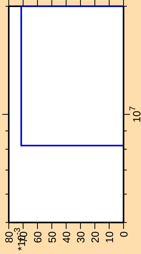
\Delta\sigma/\sigma vs. E for ^{182}\text{Hg}(n,\text{nt})
