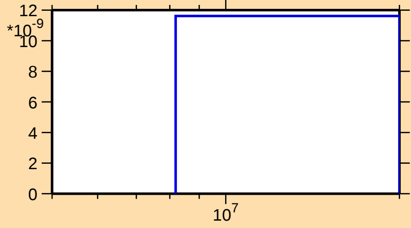
\sigma vs. E for ^{182}\text{Hg}(\text{mt117})
