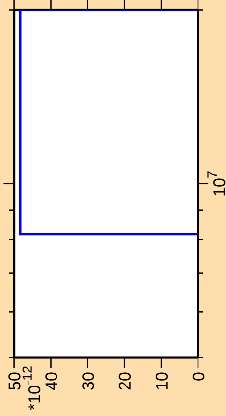
\Delta\sigma/\sigma vs. E for ^{182}\text{Hg}(\text{mt } 11)
