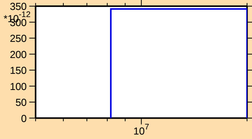
\sigma vs. E for ^{182}\text{Hg}(n,3n)
