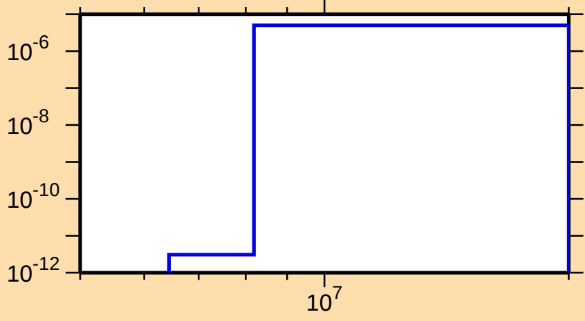
\sigma vs. E for ^{182}\text{Hg}(\text{mt } 45)
