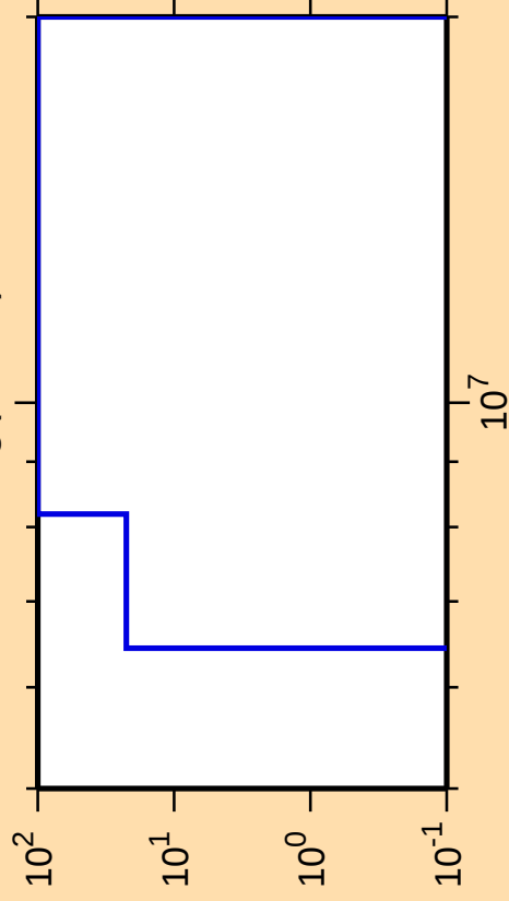
\Delta\sigma/\sigma vs. E for ^{182}\text{Hg}(\text{mt } 45)
