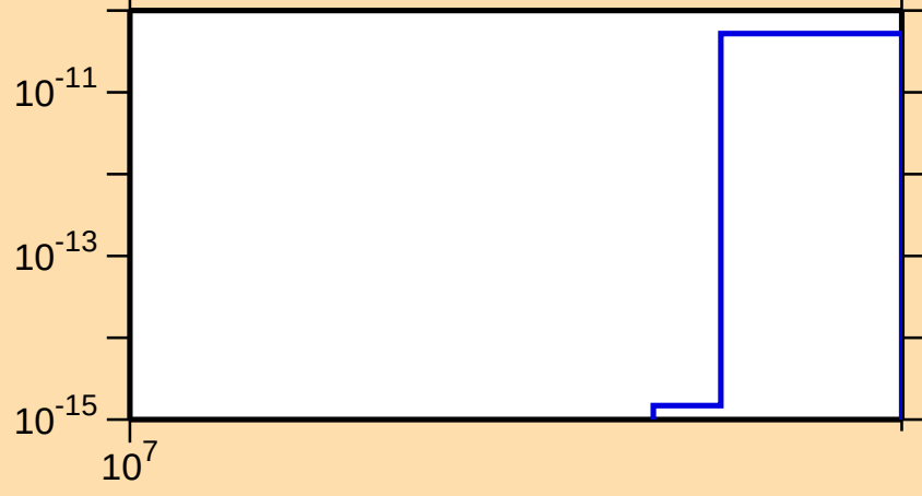
\sigma vs. E for ^{186}\text{Hg}(n,\text{nt})
