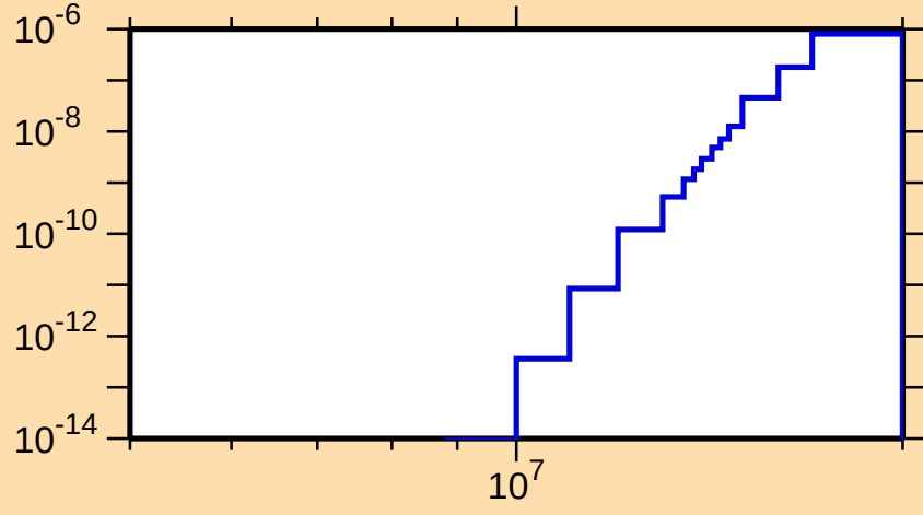
\sigma vs. E for ^{186}\text{Hg}(\text{mt } 45)
