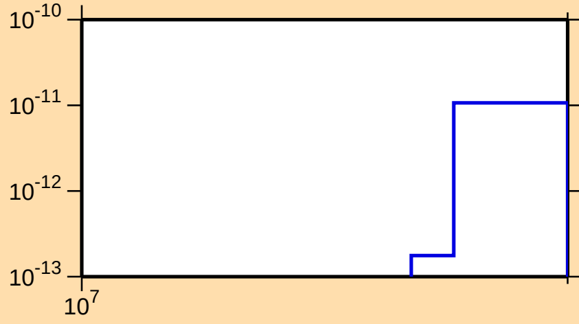
\sigma vs. E for ^{186}\text{Hg} (mt 34)
