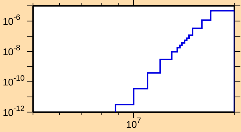
\sigma vs. E for ^{186}\text{Hg}(n,\text{He}3)
