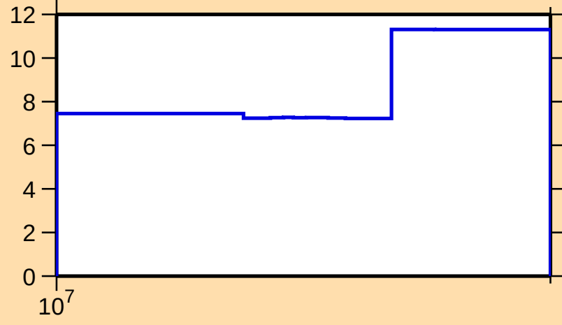
\Delta\sigma/\sigma vs. E for ^{186}\text{Hg}(n,\text{tot.})
