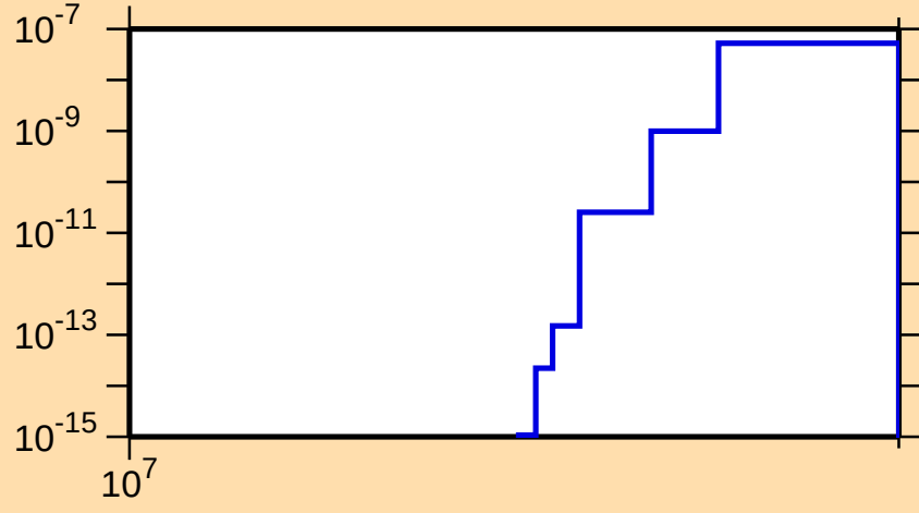
\sigma vs. E for ^{186}\text{Hg}(n,\text{nd})
