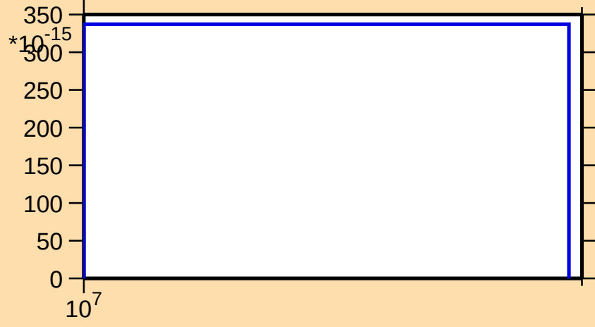
\sigma vs. E for ^{186}\text{Hg}(n,\text{nt})
