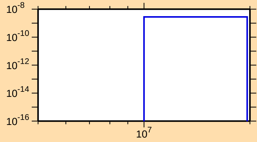
\sigma vs. E for ^{186}\text{Hg}(n,\text{pd})
