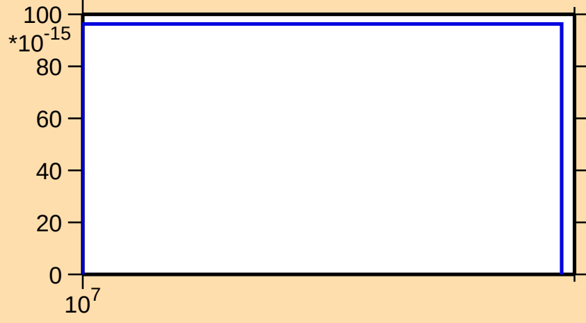
\sigma vs. E for ^{186}\text{Hg} (mt 34)
