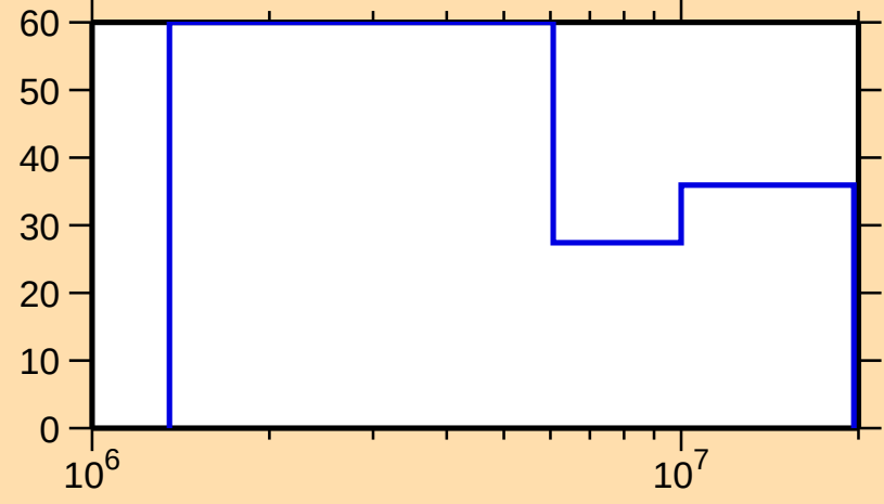
\Delta\sigma/\sigma vs. E for ^{186}\text{Hg}(\text{n},\text{inel.})
