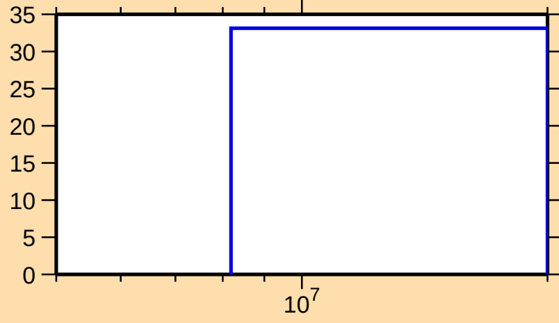
\Delta\sigma/\sigma vs. E for ^{186}\text{Hg}(n,\text{inel.})
