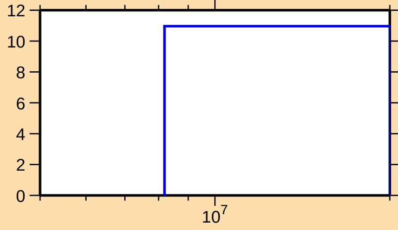
\Delta\sigma/\sigma vs. E for ^{186}\text{Hg}(n,\text{nonel.})
