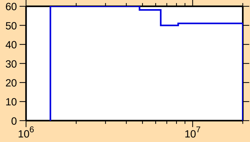
\Delta\sigma/\sigma vs. E for ^{186}\text{Hg}(n,n_1)
