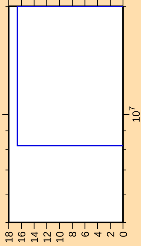
\Delta\sigma/\sigma vs. E for ^{186}\text{Hg}(n,\text{pt})
