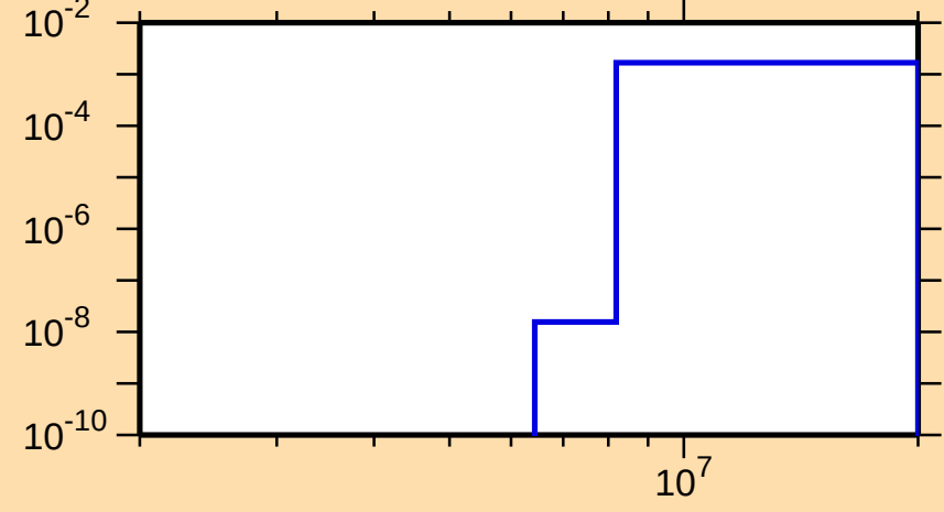
\sigma vs. E for ^{186}\text{Hg}(n,d)
