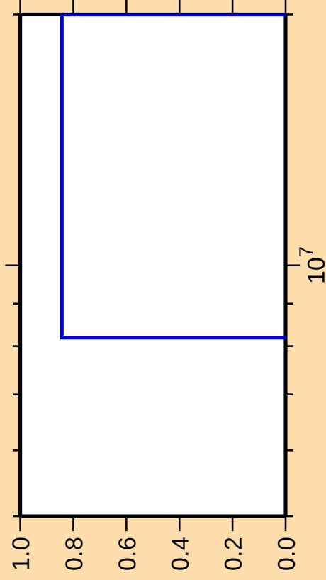
\Delta\sigma/\sigma vs. E for ^{186}\text{Hg}(\text{mt } 34)
