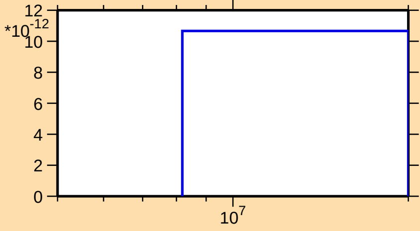
\sigma vs. E for ^{186}\text{Hg}(n,3n\alpha)
