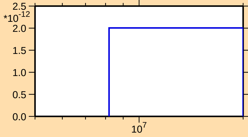
\sigma vs. E for ^{186}\text{Hg}(n,\text{pt})
