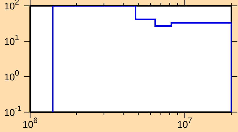
\Delta\sigma/\sigma vs. E for ^{186}\text{Hg}(\text{n},\text{inel.})
