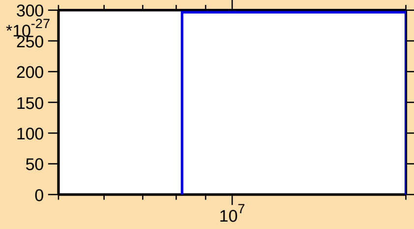
\sigma vs. E for ^{186}\text{Hg}(\text{mt } 11)
