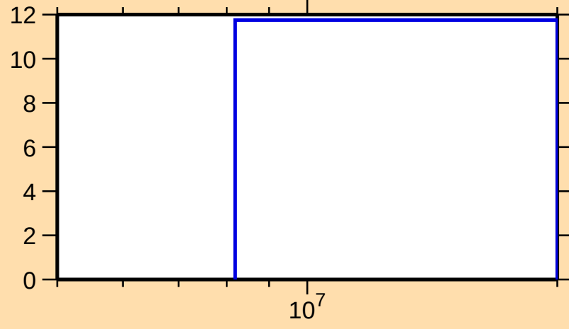
\Delta\sigma/\sigma vs. E for ^{186}\text{Hg}(n,\text{el.})
