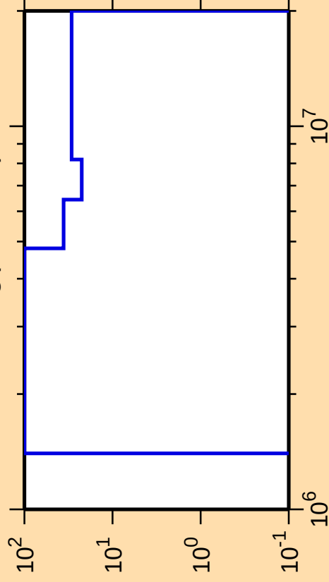
\Delta\sigma/\sigma vs. E for ^{186}\text{Hg}(\text{n},\text{ncont.})
