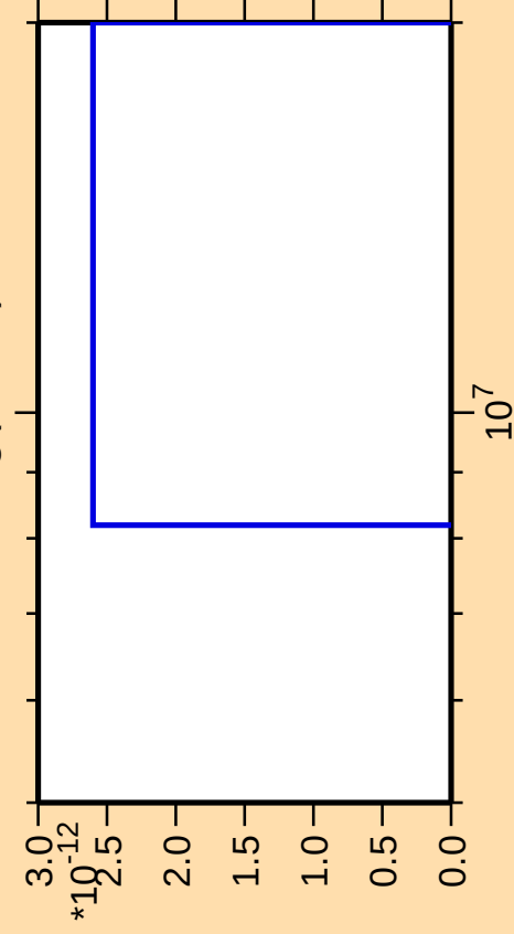
\Delta\sigma/\sigma vs. E for ^{186}\text{Hg}(\text{mt } 11)
