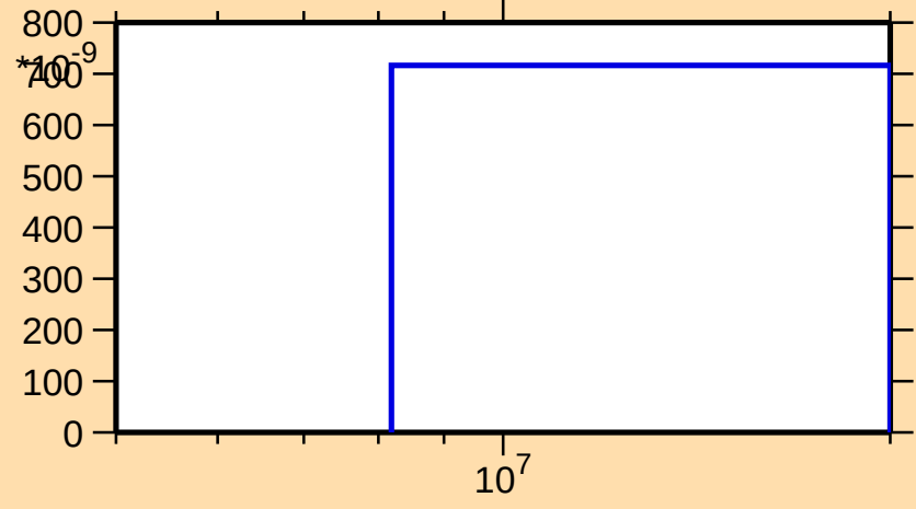
\sigma vs. E for ^{186}\text{Hg}(n,2n\alpha)
