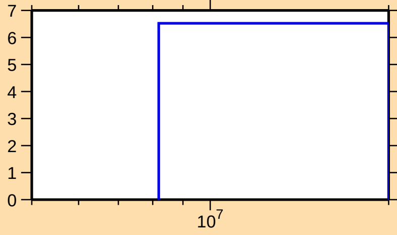
\Delta\sigma/\sigma vs. E for ^{186}\text{Hg}(n,\text{tot.})
