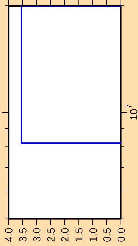
\Delta\sigma/\sigma vs. E for ^{186}\text{Hg}(n,\text{nt})
