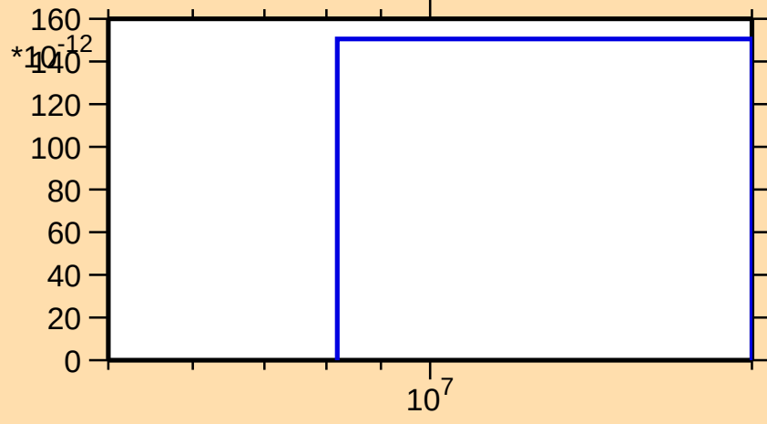
\sigma vs. E for ^{186}\text{Hg}(\text{mt117})
