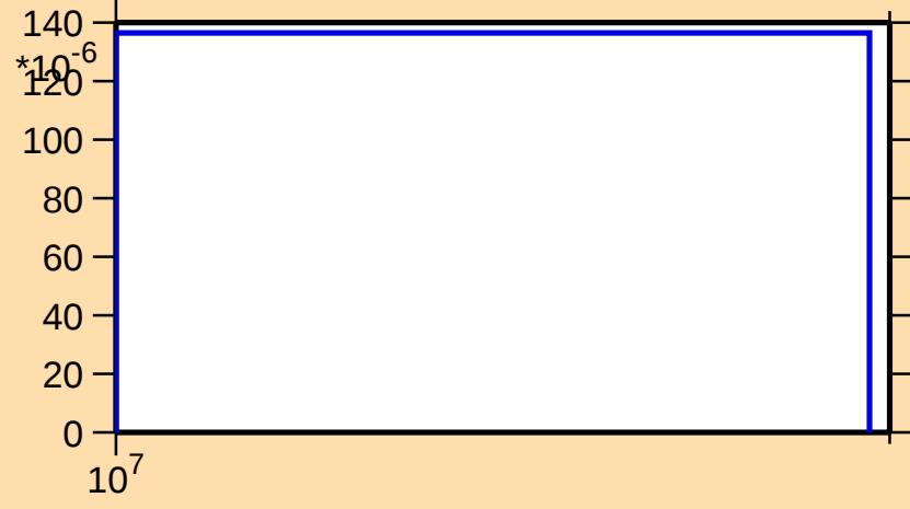
\sigma vs. E for ^{194}\text{Hg}(n,3n)
