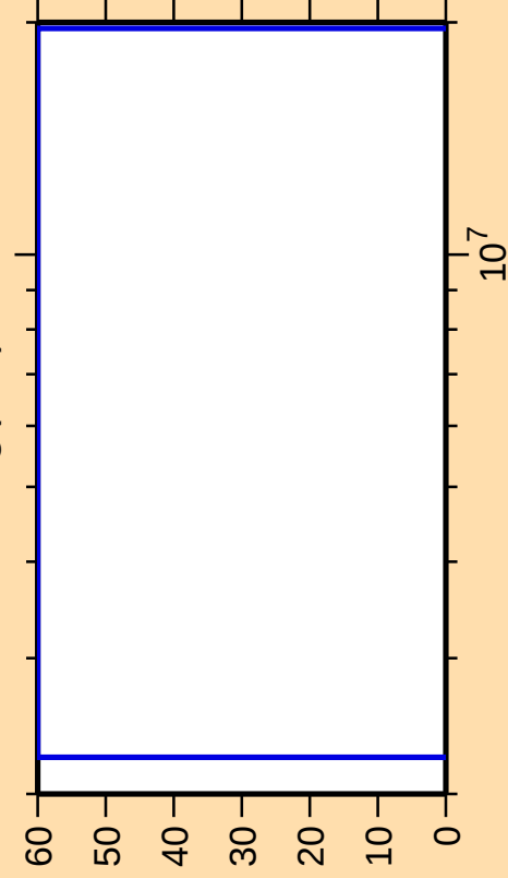
\Delta\sigma/\sigma vs. E for ^{194}\text{Hg}(n,\alpha)
