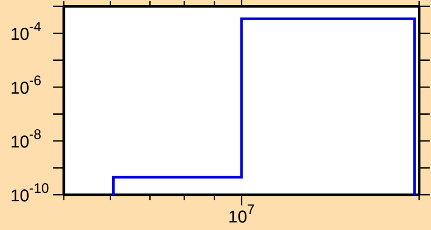
\sigma vs. E for ^{194}\text{Hg}(n,d)
