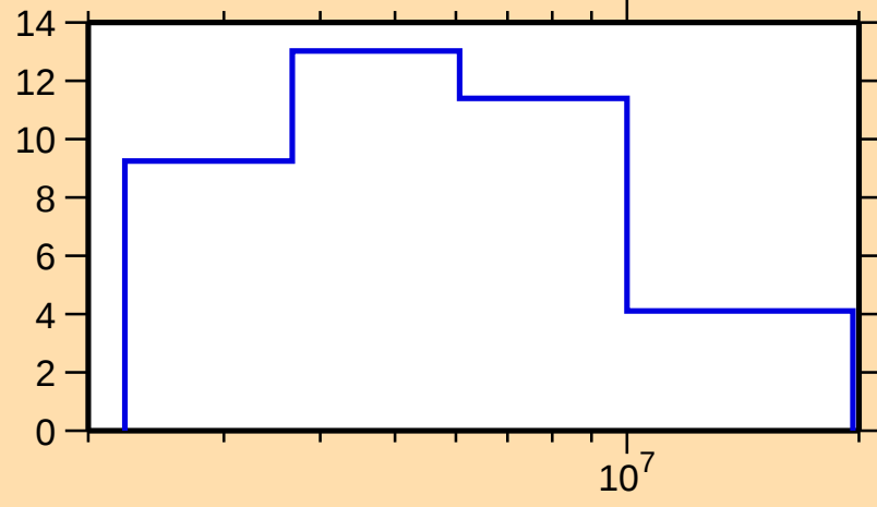
\Delta\sigma/\sigma vs. E for ^{194}\text{Hg}(\text{n},\text{tot.})
