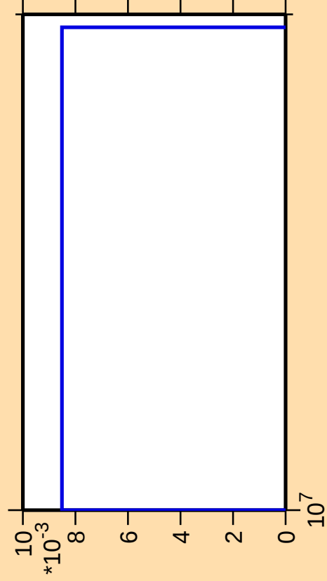
\Delta\sigma/\sigma vs. E for ^{194}\text{Hg}(n,\text{pd})
