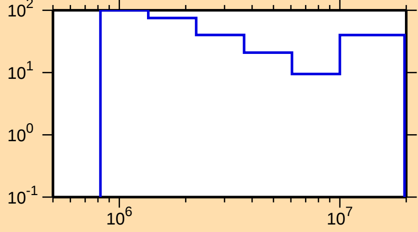
\Delta\sigma/\sigma vs. E for ^{194}\text{Hg}(n,\text{inel.})
