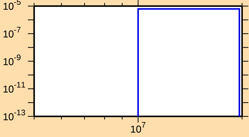
\sigma vs. E for ^{194}\text{Hg}(n,t)
