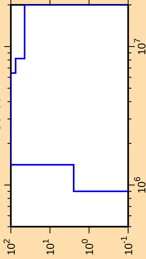
\Delta\sigma/\sigma vs. E for ^{194}\text{Hg}(n,p)
