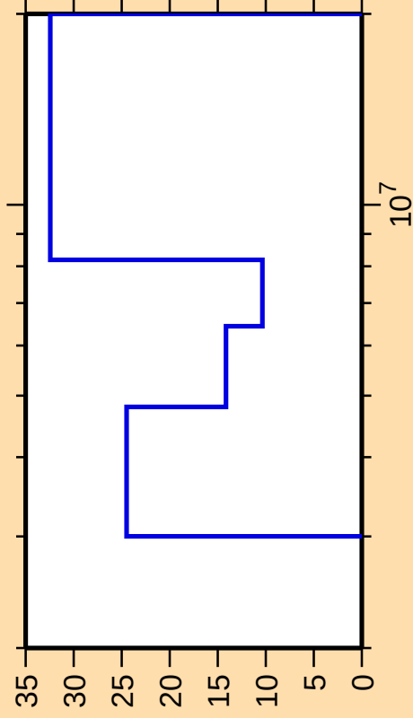
\Delta\sigma/\sigma vs. E for ^{194}\text{Hg}(n,\text{ncont.})
