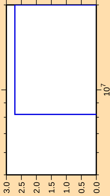
\Delta\sigma/\sigma vs. E for ^{194}\text{Hg}(n,\text{nt})
