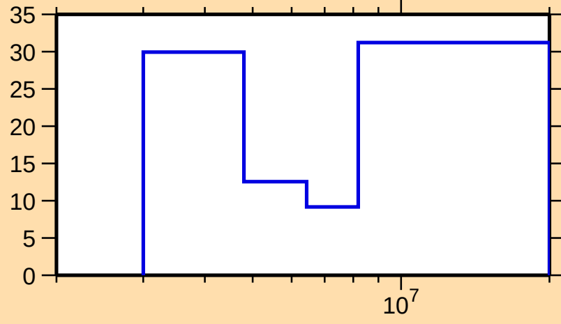
\Delta\sigma/\sigma vs. E for ^{194}\text{Hg}(\text{n},\text{inel.})
