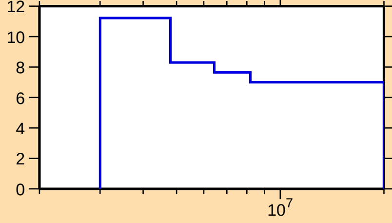
\Delta\sigma/\sigma vs. E for ^{194}\text{Hg}(\text{n},\text{nonel.})
