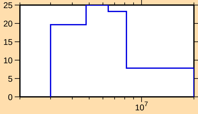
\Delta\sigma/\sigma vs. E for ^{194}\text{Hg}(\text{n},\text{el.})
