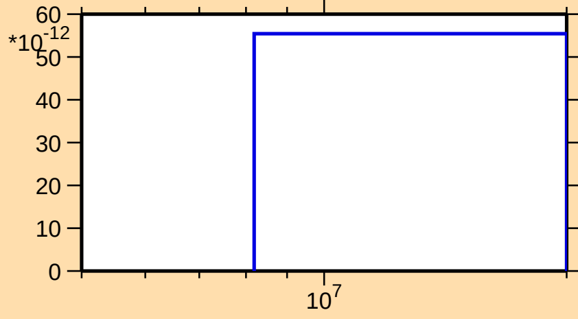
\sigma vs. E for ^{194}\text{Hg}(n,2np)
