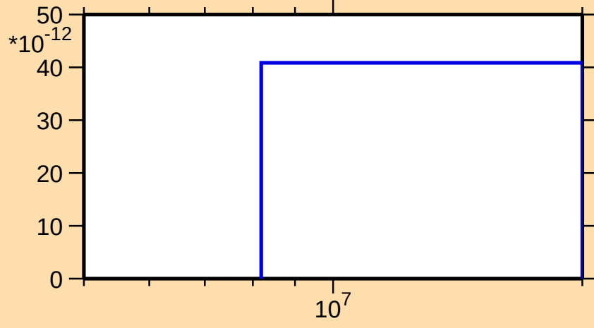
\sigma vs. E for ^{194}\text{Hg}(n,\text{He}3)
