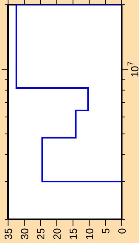
\Delta\sigma/\sigma vs. E for ^{194}\text{Hg}(\text{n},\text{ncont.})
