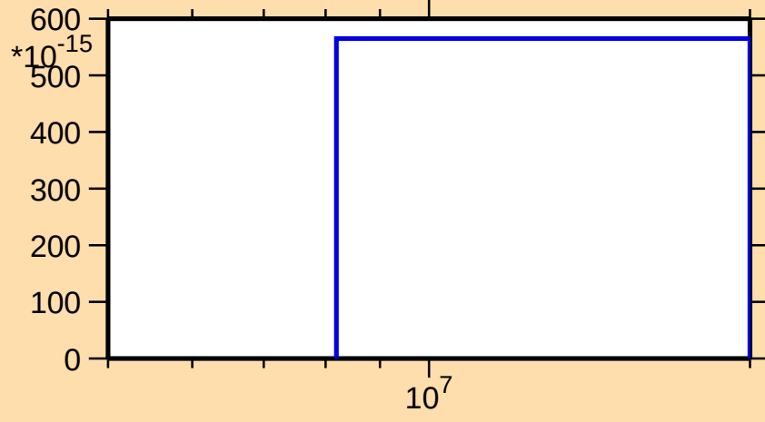
\sigma vs. E for ^{194}\text{Hg}(n,\text{nt})
