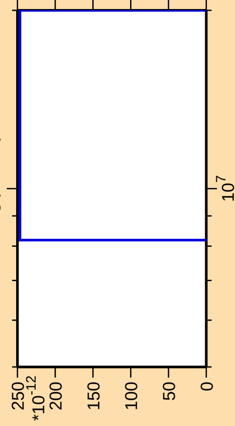
\Delta\sigma/\sigma vs. E for ^{194}\text{Hg}(\text{mt } 11)
