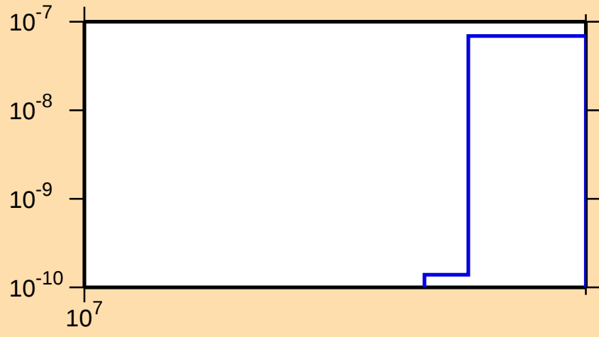
\sigma vs. E for ^{207}\text{Hg}(n,2np)
