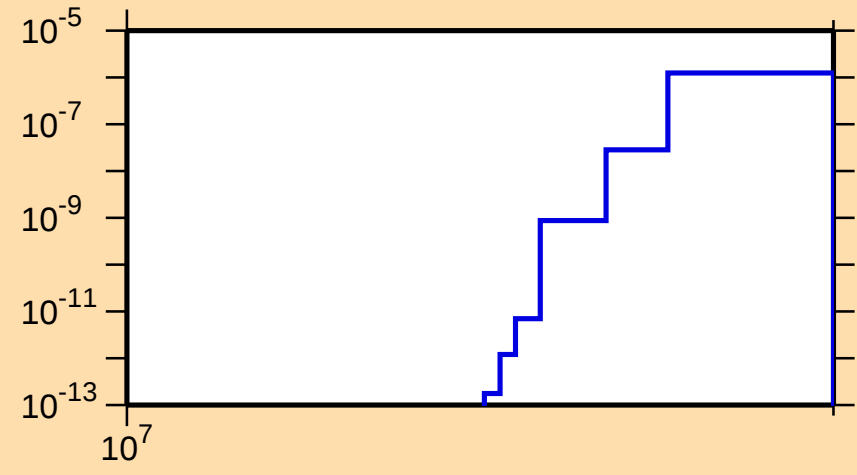
\sigma vs. E for ^{207}\text{Hg}(n,\text{nd})
