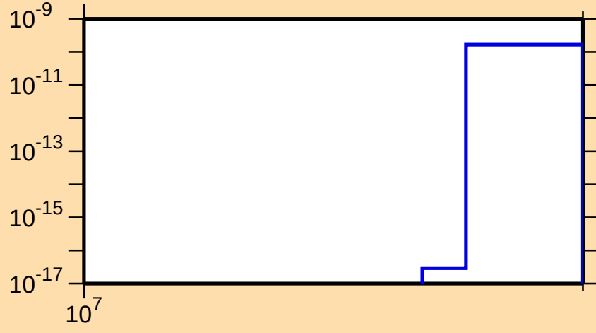
\sigma vs. E for ^{214}\text{Hg}(n,2np)
