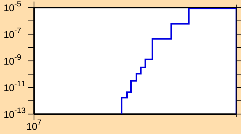
\sigma vs. E for ^{214}\text{Hg}(n,np)
