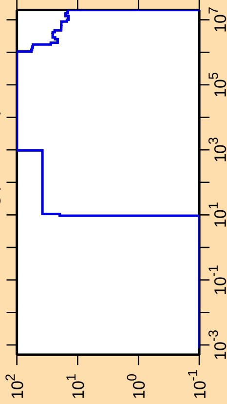
\Delta\sigma/\sigma vs. E for ^{214}\text{Hg}(n,\text{nonel.})
