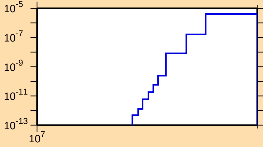
\sigma vs. E for ^{214}\text{Hg}(n,\text{nt})
