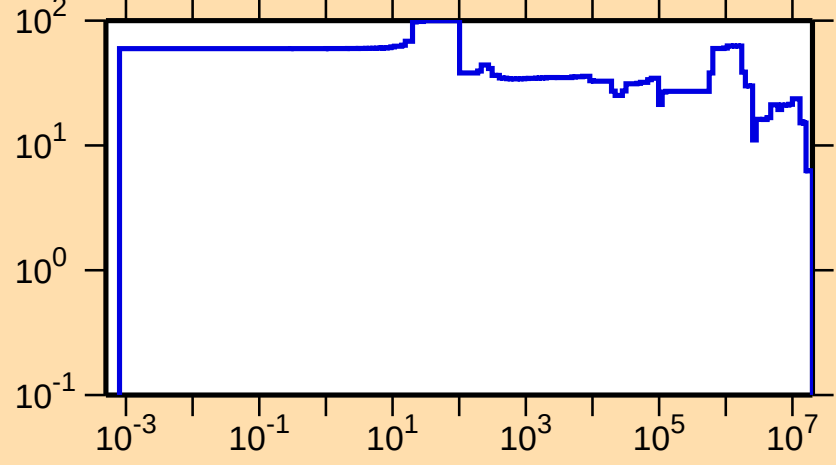
\Delta\sigma/\sigma vs. E for ^{214}\text{Hg}(\text{n,el.})
