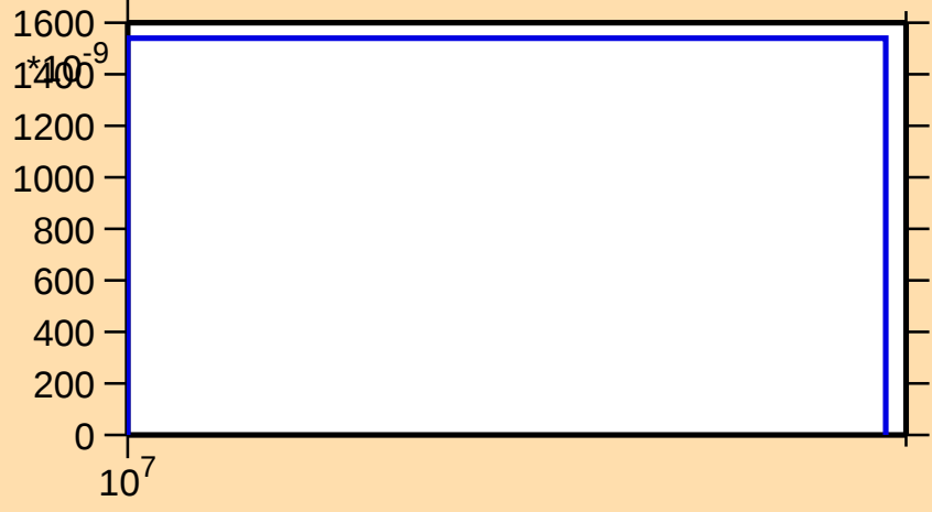
\sigma vs. E for ^{214}\text{Hg}(n,p)
