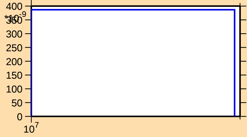
\sigma vs. E for ^{214}\text{Hg}(n,d)
