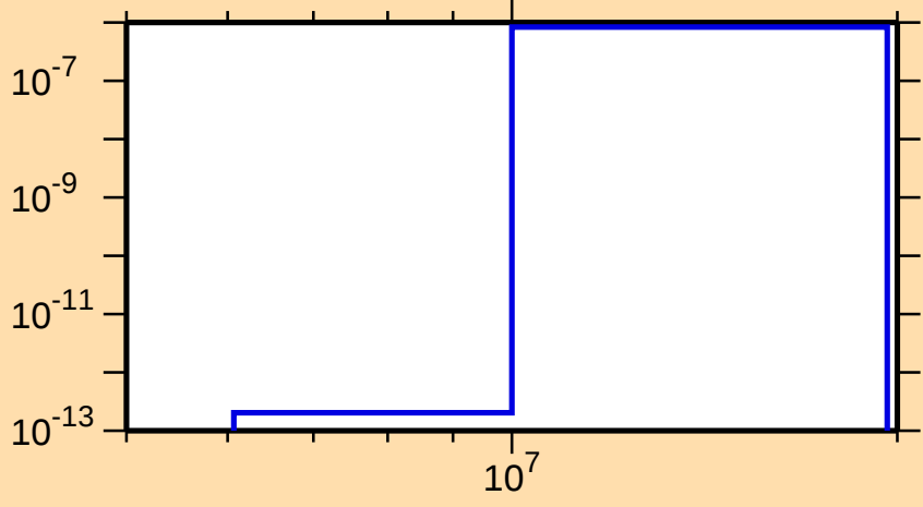
\sigma vs. E for ^{214}\text{Hg}(n,\alpha)
