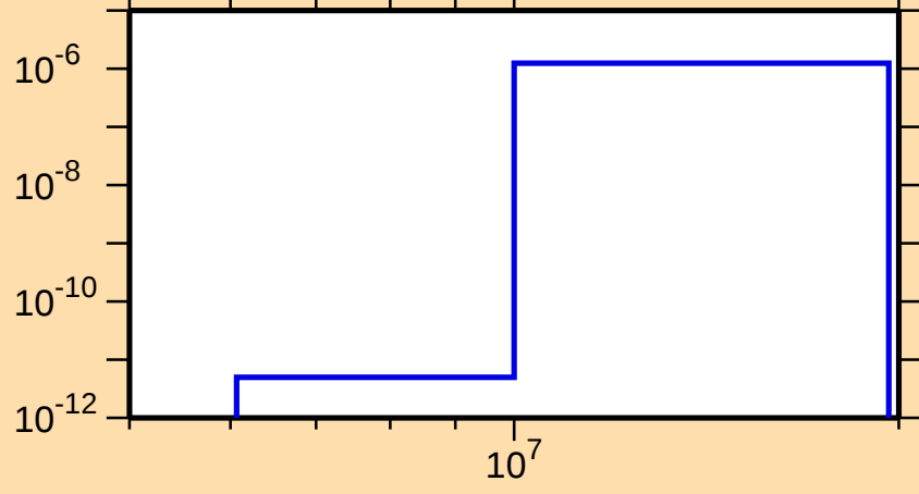
\sigma vs. E for ^{214}\text{Hg}(n,\alpha)
