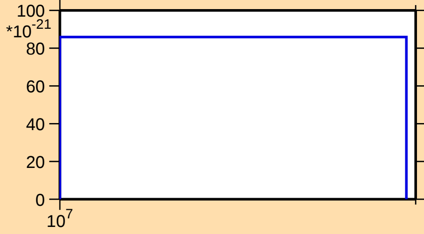
\sigma vs. E for ^{214}\text{Hg} (mt 42)
