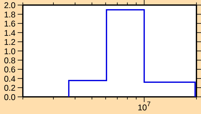
\sigma vs. E for ^{214}\text{Hg}(n,2n)
