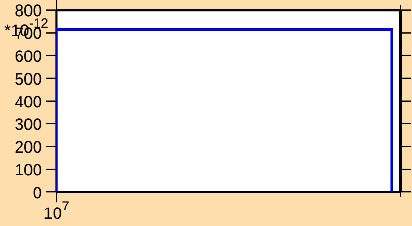
\sigma vs. E for ^{214}\text{Hg}(n,2n\alpha)
