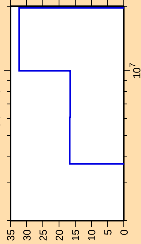
\Delta\sigma/\sigma vs. E for ^{214}\text{Hg}(n,2n)
