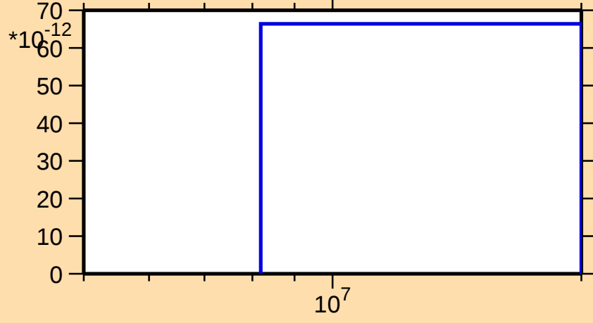
\sigma vs. E for ^{214}\text{Hg}(n,\text{nd})
