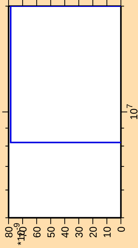
\Delta\sigma/\sigma vs. E for ^{214}\text{Hg}(\text{mt } 42)
