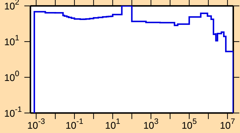
\Delta\sigma/\sigma vs. E for ^{214}\text{Hg}(n,\text{tot.})
