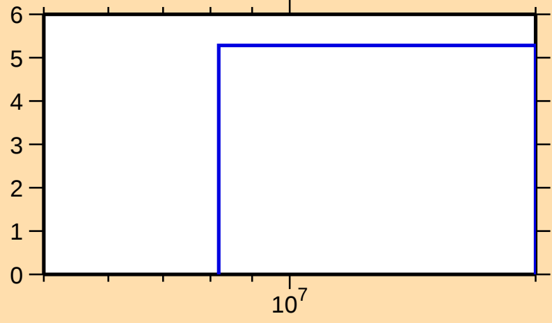
\Delta\sigma/\sigma vs. E for ^{214}\text{Hg}(n,\text{tot.})
